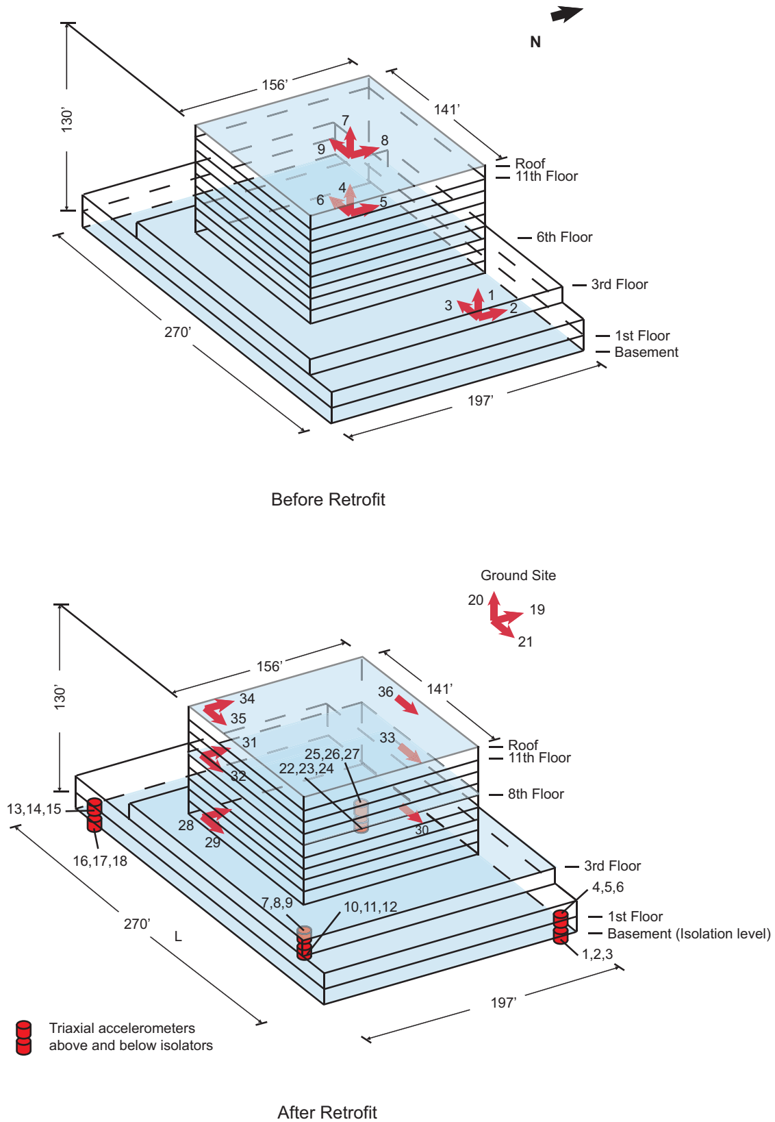
Figure 16. Instrumentation scheme for 5901 E. 7 th St., showing configurations before (left) and after (right) seismic retrofit
