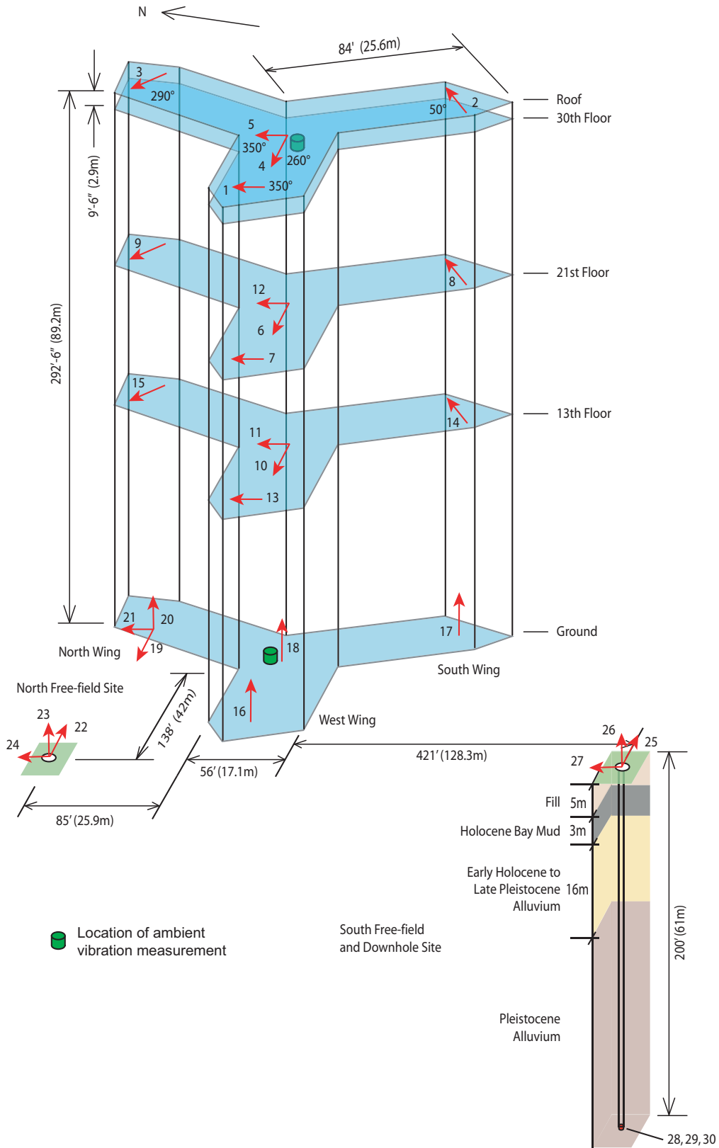
Figure 14. Instrumentation scheme and ambient vibration measurement locations for 6363 Christie Ave. Ambient velocity measurements taken on 30 th floor while permanent instruments are located on roof.
