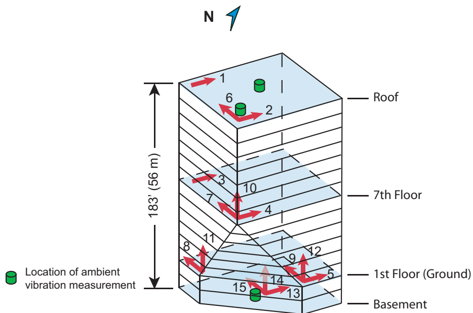
Figure 23. Instrumentation scheme and ambient vibration measurement locations for 1990 MacArthur Blvd.
