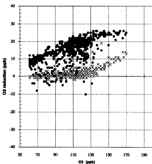
Fig. 11. Predicted reduction in peak O_3 (ppb) on 10 August 1992 resulting from a 35% reduction in emission of anthropogenic ROG (crosses) or from a 35% reduction in anthropogenic NO_x emissions (circles) plotted vs peak O_3 , based on the eight-layer scenario B (reduced vertical mixing).
