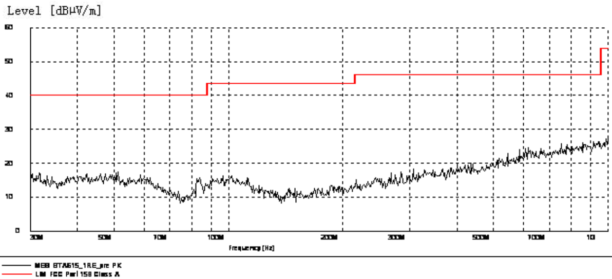
Figure B.1 Radiated Emission from 30MHz to 1GHz
