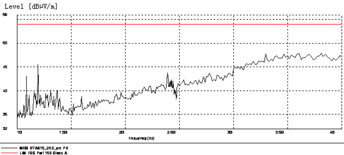
Figure B.2 Radiated Emission from 1GHz to 4GHz
