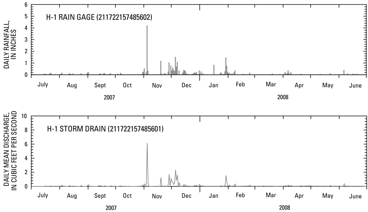
Figure 12. Rainfall for H-1 rain gage and discharge for H-1 storm drain, Oahu, Hawaii, for July 1, 2007, to June 30, 2008.
