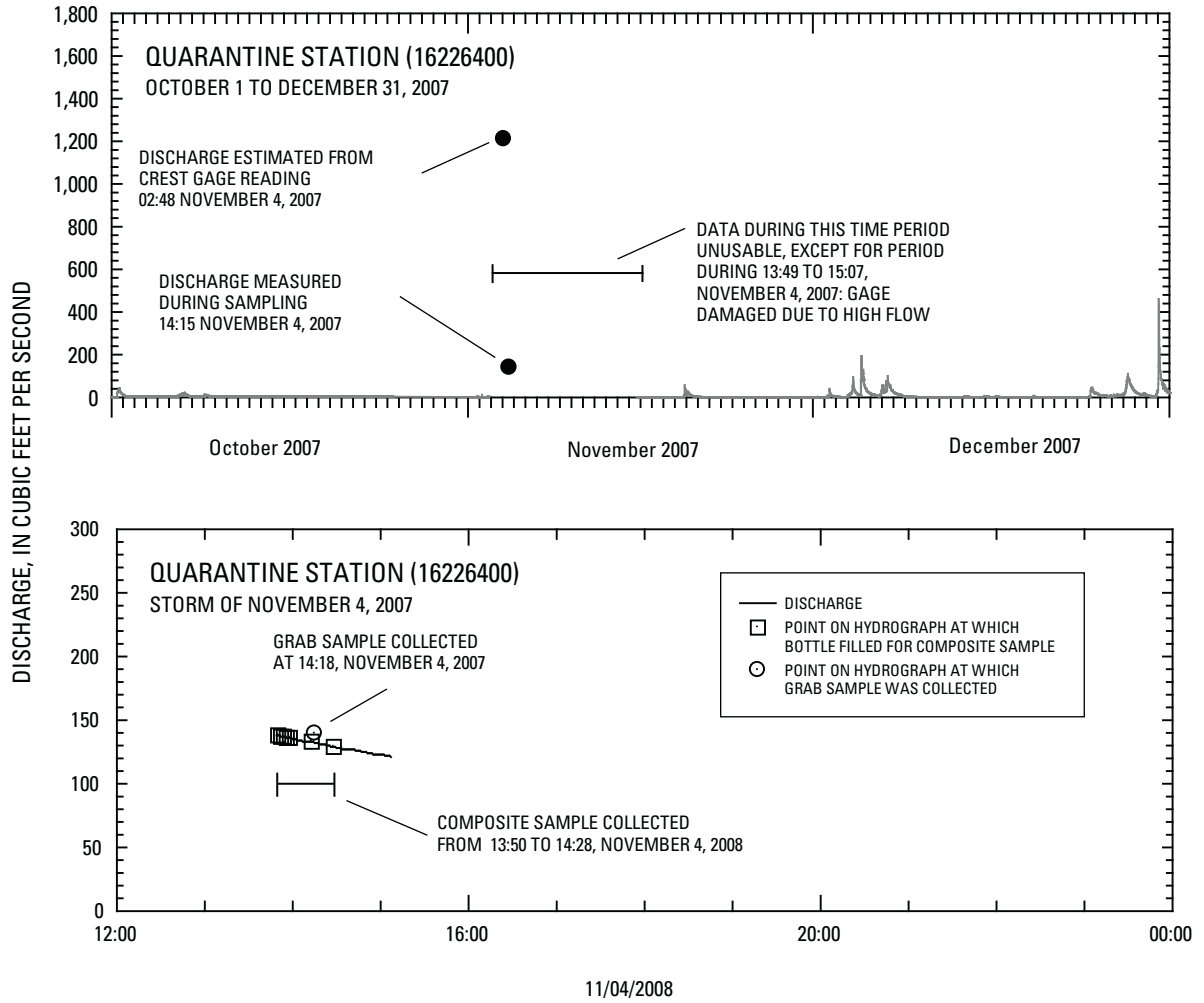
Figure 7. Stream discharge at Quarantine station (16226400) for October 1 to December 31, 2007; and detail of 12-hour period from 12:00 November 4 to 00:00 November 5, 2007, Oahu, Hawaii.
