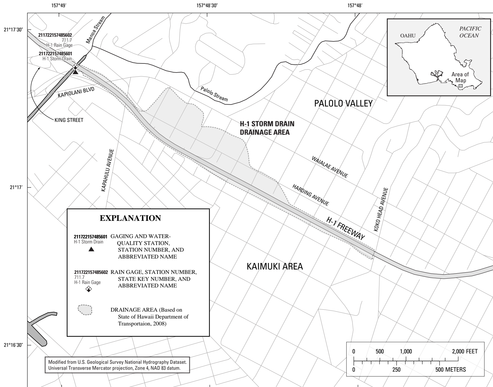
Figure 2. Drainage area of the H-1 storm drain and location of the H-1 rain gage, H-1 storm drain gage and sampling site, Oahu, Hawaii.
