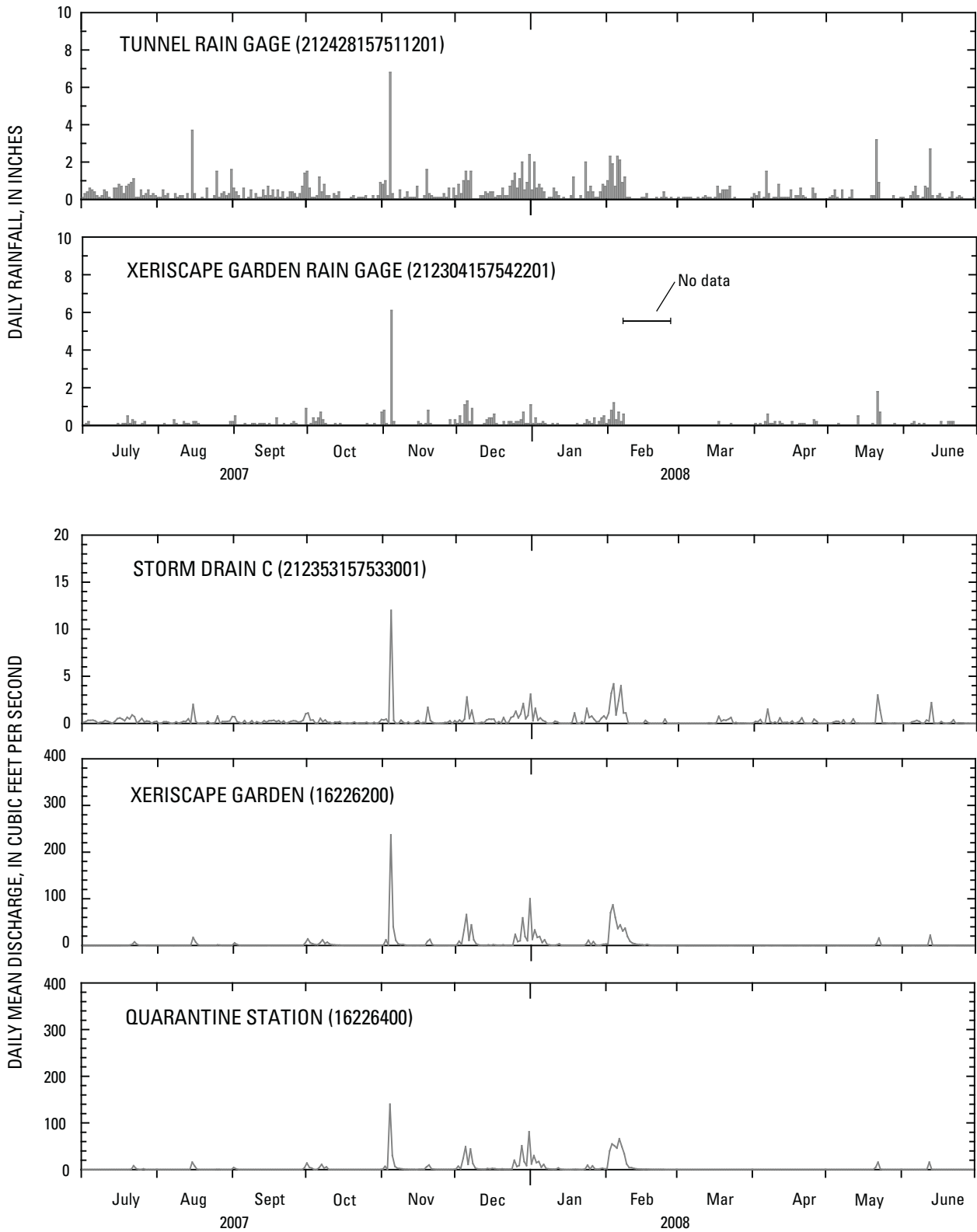
Figure 3. Rainfall and discharge for stations within the Halawa Stream drainage basin, Oahu, Hawaii, for July 1, 2007, to June 30, 2008.
