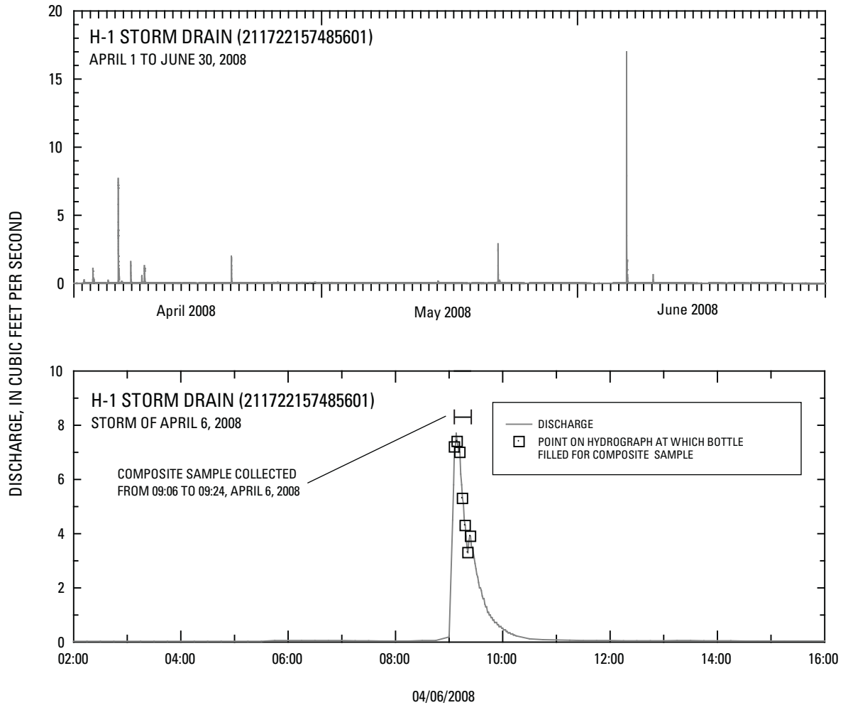
Figure 16. Discharge at H-1 storm drain (211722157485601) for April 1 to June 30, 2008; and detail of 14-hour period from 02:00 to 16:00, April 6, 2008, Oahu, Hawaii.
