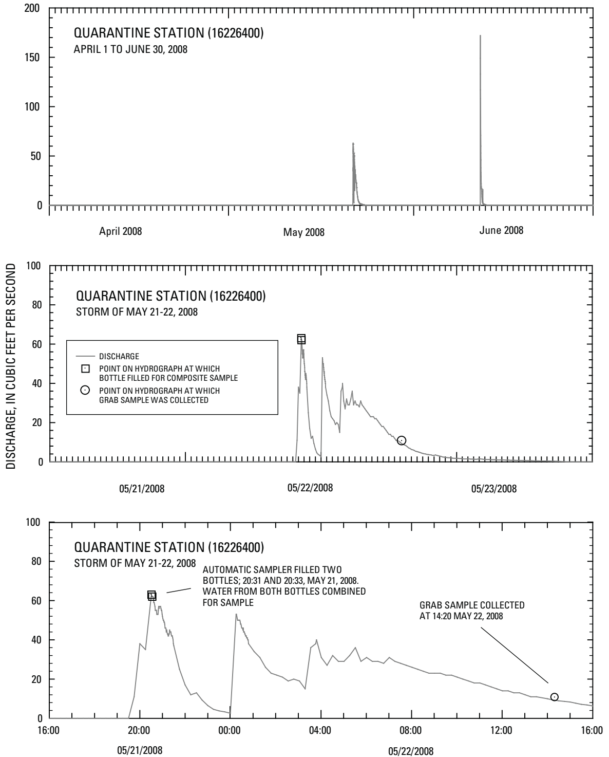
Figure 11. Stream discharge at Quarantine station (16226400) for April 1 to June 30, 2008; detail of 3-day period from May 21 to 23, 2008; and detail of 24-hour period from 16:00 May 21 to 16:00 May 22, 2008, Oahu, Hawaii.
