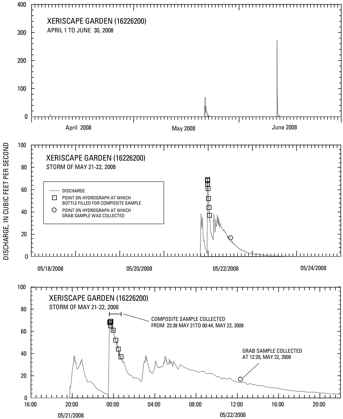
Figure 10. Stream discharge at Xeriscape garden station (16226200) for April 1 to June 30, 2008; detail of 7-day period from May 18 to 24, 2008; and detail of 30-hour period from 16:00 May 21 to 22:00 May 22, 2008, Oahu, Hawaii.
