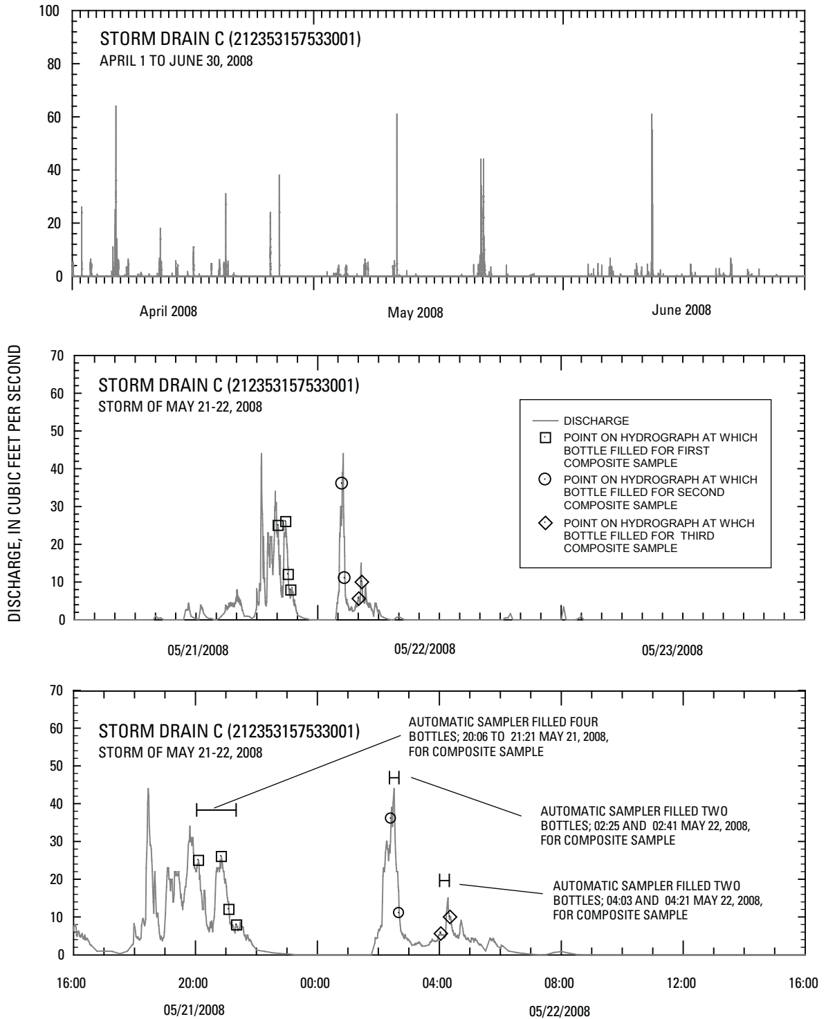
Figure 9. Discharge at Storm drain C (212353157533001) for April 1 to June 30, 2008; detail of 3-day period from May 21 to 23, 2008; and detail of 24-hour period from 16:00 May 21 to 16:00 May 22, 2008, Oahu, Hawaii.
