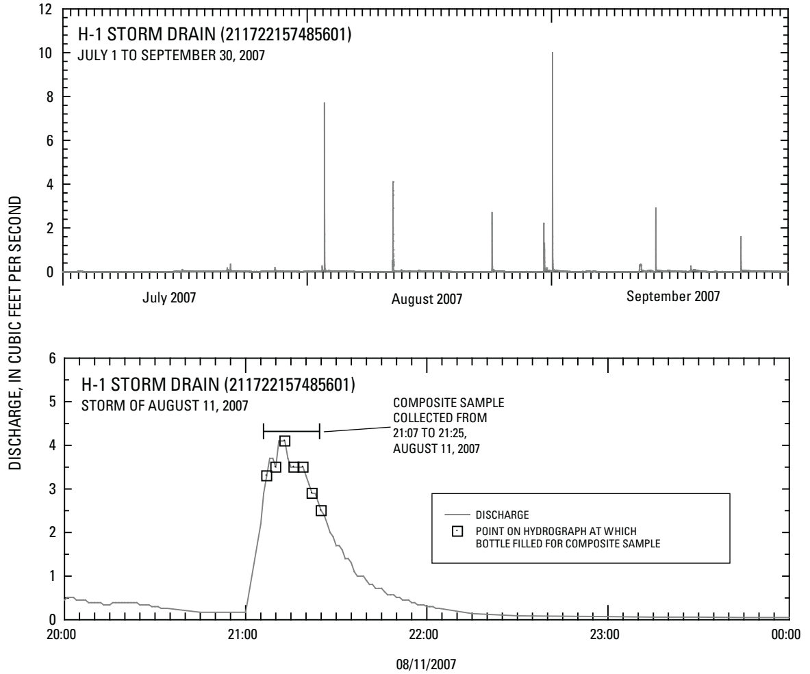
Figure 13. Discharge at H-1 storm drain (211722157485601) for July 1 to September 30, 2007; and detail of 4-hour period from 20:00 August 11 to 00:00 August 12, 2007, Oahu, Hawaii.
