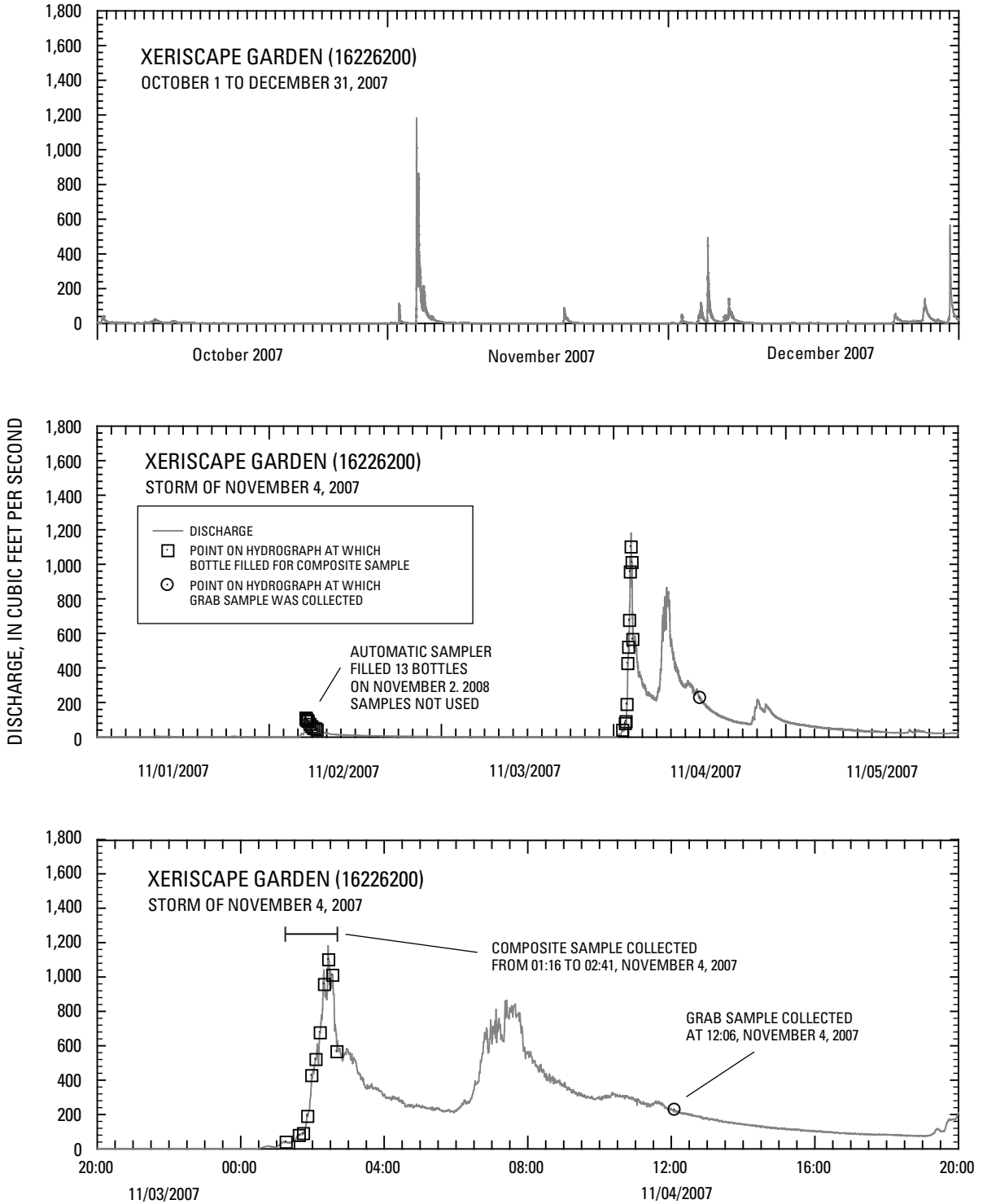
Figure 6. Stream discharge at Xeriscape garden station (16226200) for October 1 to December 31, 2007; detail of 5-day period from November 1 to 5, 2007; and detail of 24-hour period from 20:00 November 3 to 20:00 November 4, 2007, Oahu, Hawaii.
