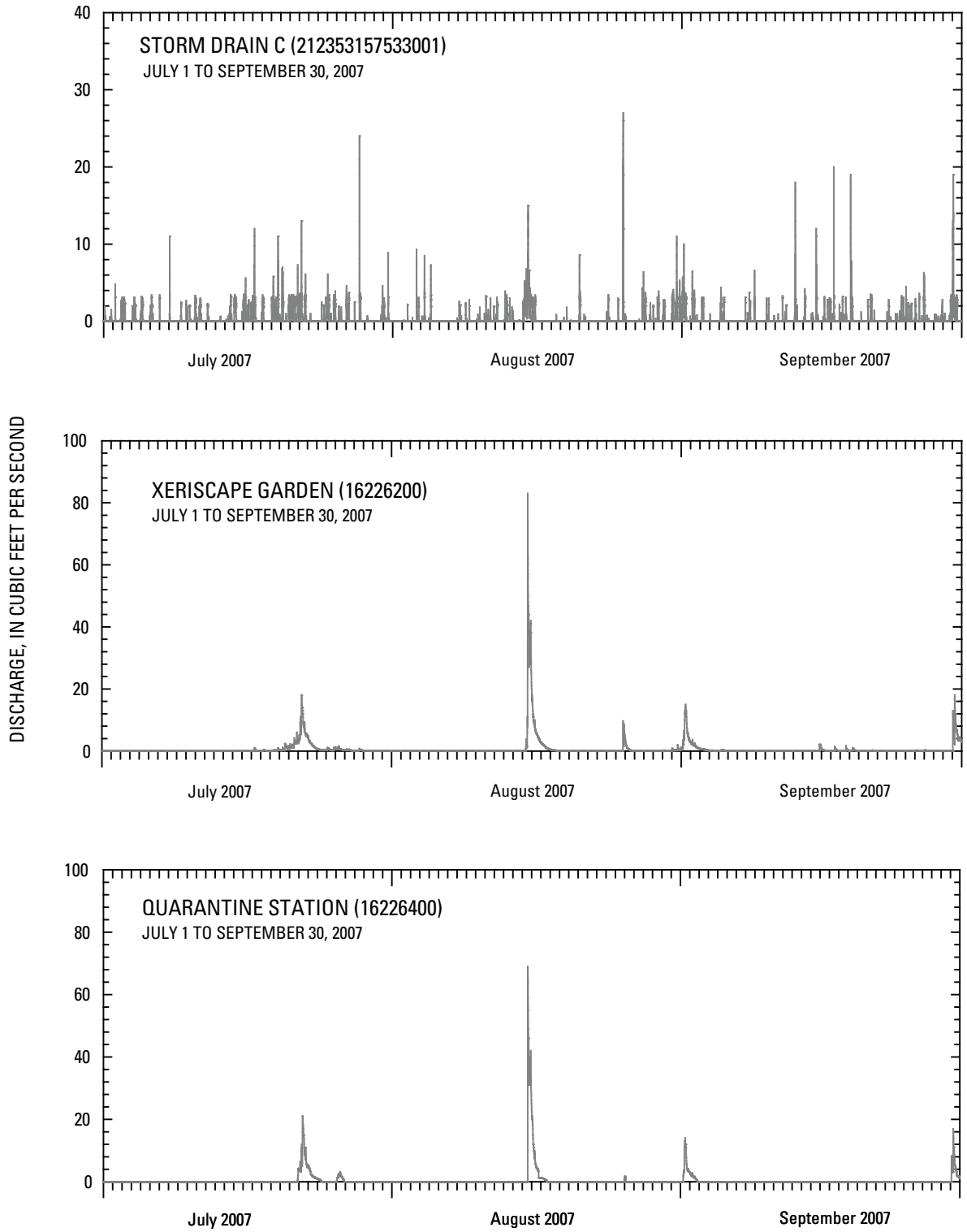
Figure 4. Discharge at Storm Drain C (212353157533001), and stream discharge at Xeriscape garden (16226200) and Quarantine station (16226400), for July 1 to September 30, 2007, Oahu, Hawaii.
