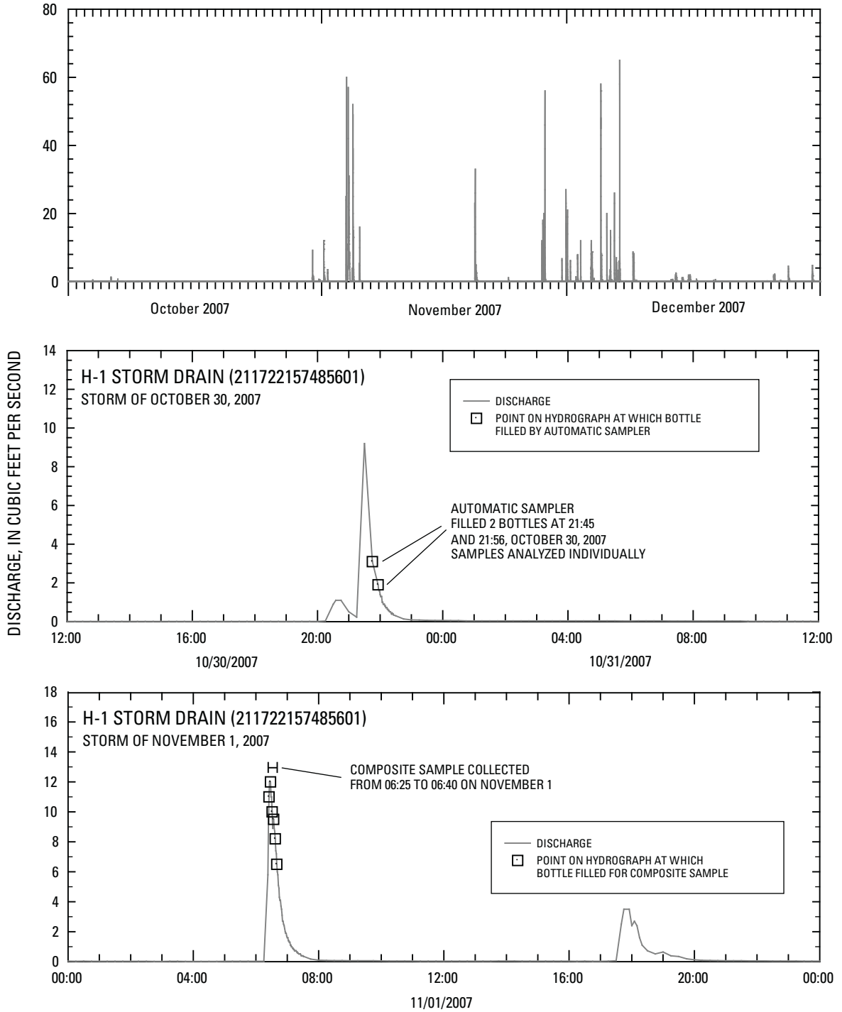
Figure 14. Discharge at H-1 storm drain (211722157485601) for October 1 to December 31, 2007; detail of 24-hour period from 12:00 October 30 to 12:00 October 31, 2007; and detail of 24-hour period from 00:00 November 1 to 00:00 November 2, 2007, Oahu, Hawaii.
