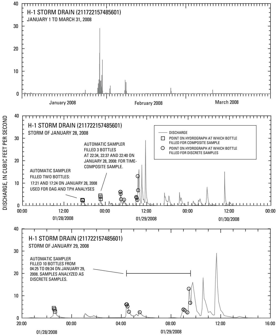
Figure 15. Discharge at H-1 storm drain (211722157485601) for January 1 to March 31, 2008; detail of 3-day period from January 28 to 30, 2008; and detail of 20-hour period from 20:00 January 28 to 16:00 January 29, 2008, Oahu, Hawaii.
