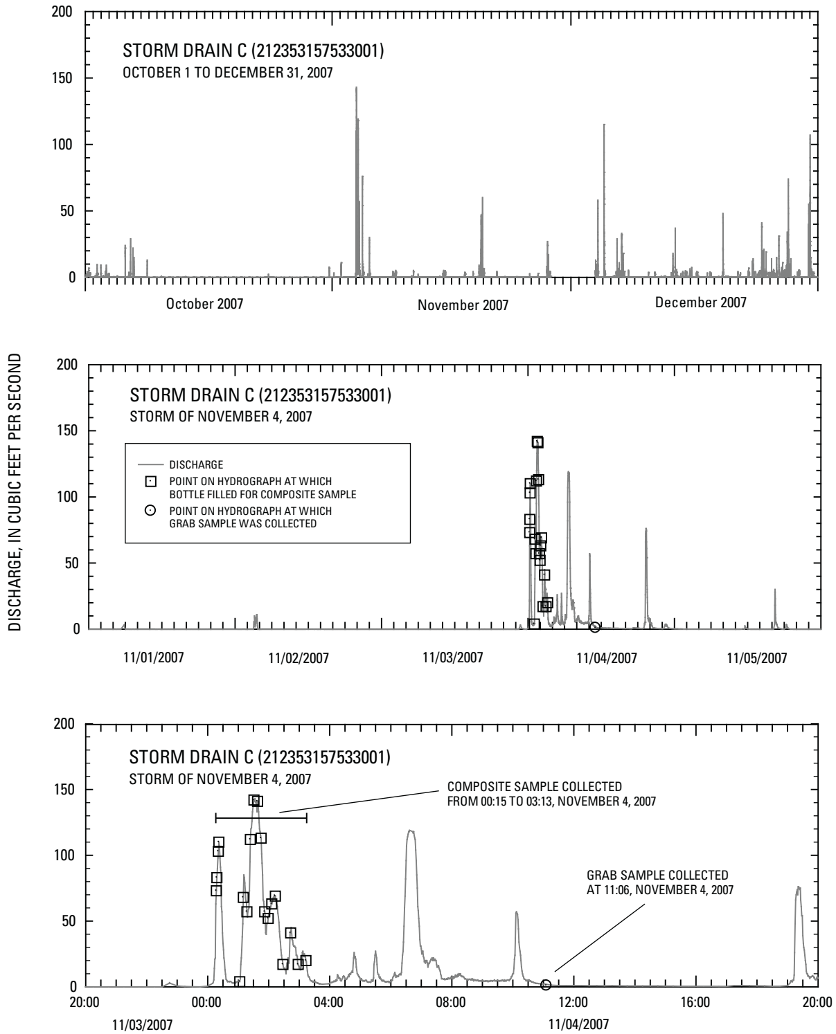
Figure 5. Discharge at Storm drain C (212353157533001) for October 1 to December 31, 2007; detail of 5-day period from November 1 to 5, 2007; and detail of 24-hour period from 20:00 November 3 to 20:00 November 4, 2007, Oahu, Hawaii.
