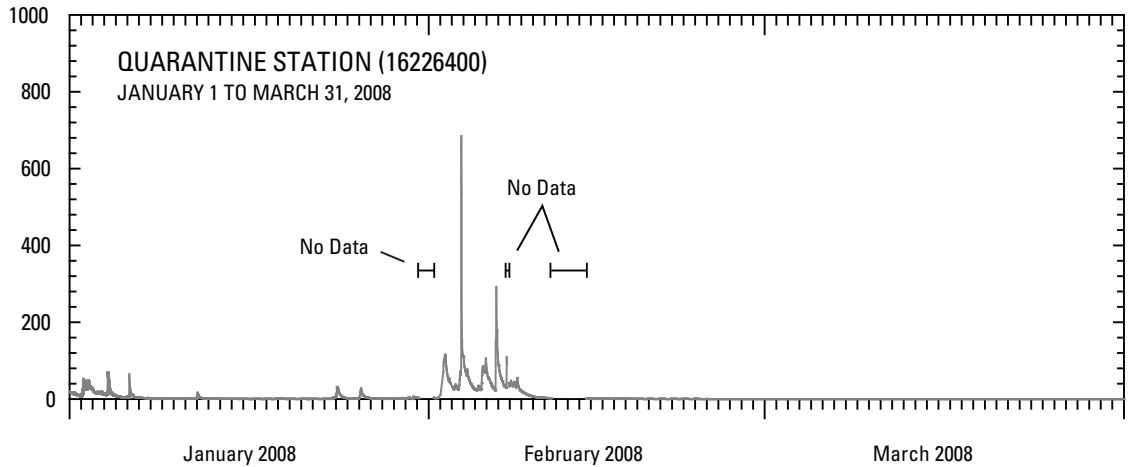
Figure 8. Discharge at Storm Drain C (212353157533001), and stream discharge at Xeriscape garden (16226200) and Quarantine station (16226400), for January 1 to March 31, 2008, Oahu, Hawaii.
