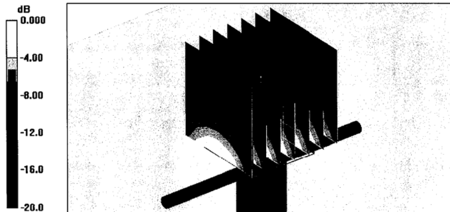
0 dB = 11.0mW/g
