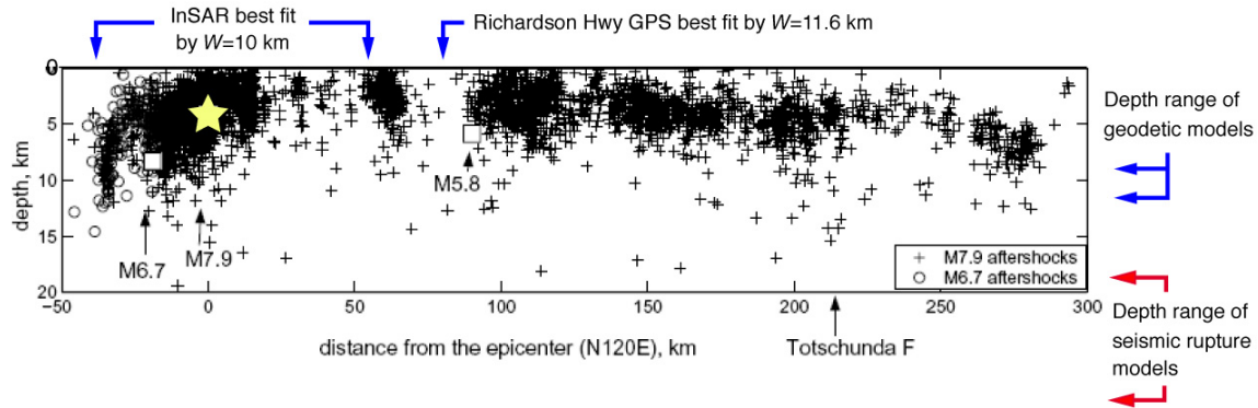
Figure 2. The aftershocks of the 2002 M=7.9 Denali shock ( Eberhart-Phillips and others, 2003 ) compared to geodetic ( Wright and others, 2004 ) and telesismic ( Asano and others, 2005; Oglesby and others, 2004, Ozacar and others, 2003 ) inferences for the lower depth of coseismic rupture.
