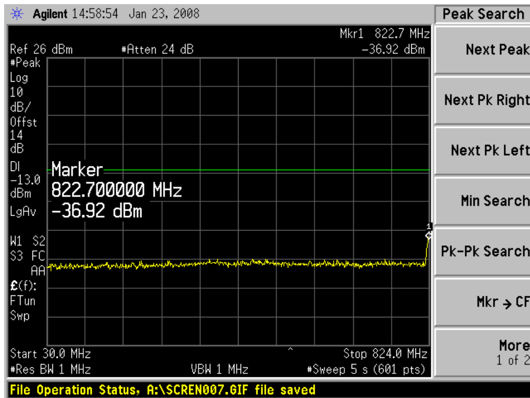
Channel 384, 30MHz~824MHz
