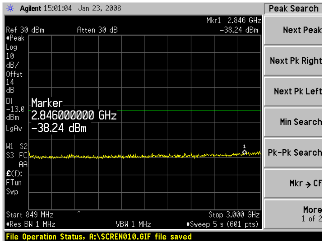
Channel 384, 849MHz~3GHz
