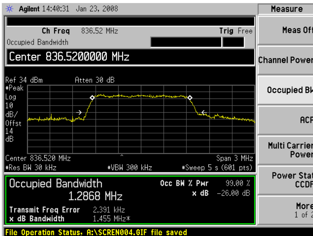
Channel 384
