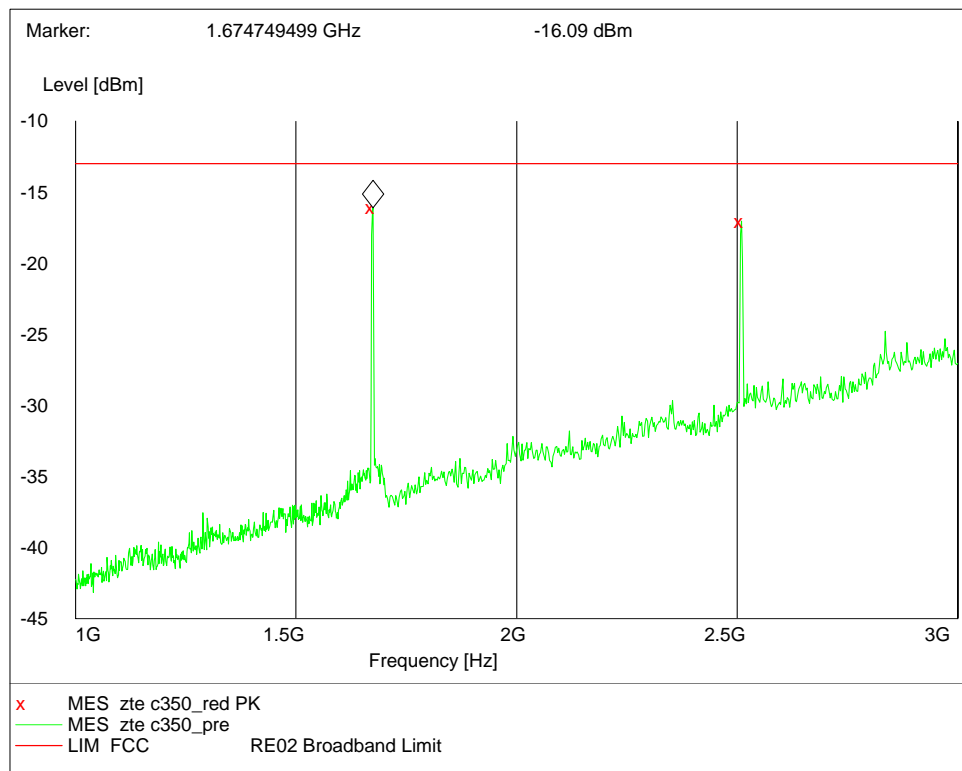
Channel 384, 1GHz~3GHz (Traffic Mode)
