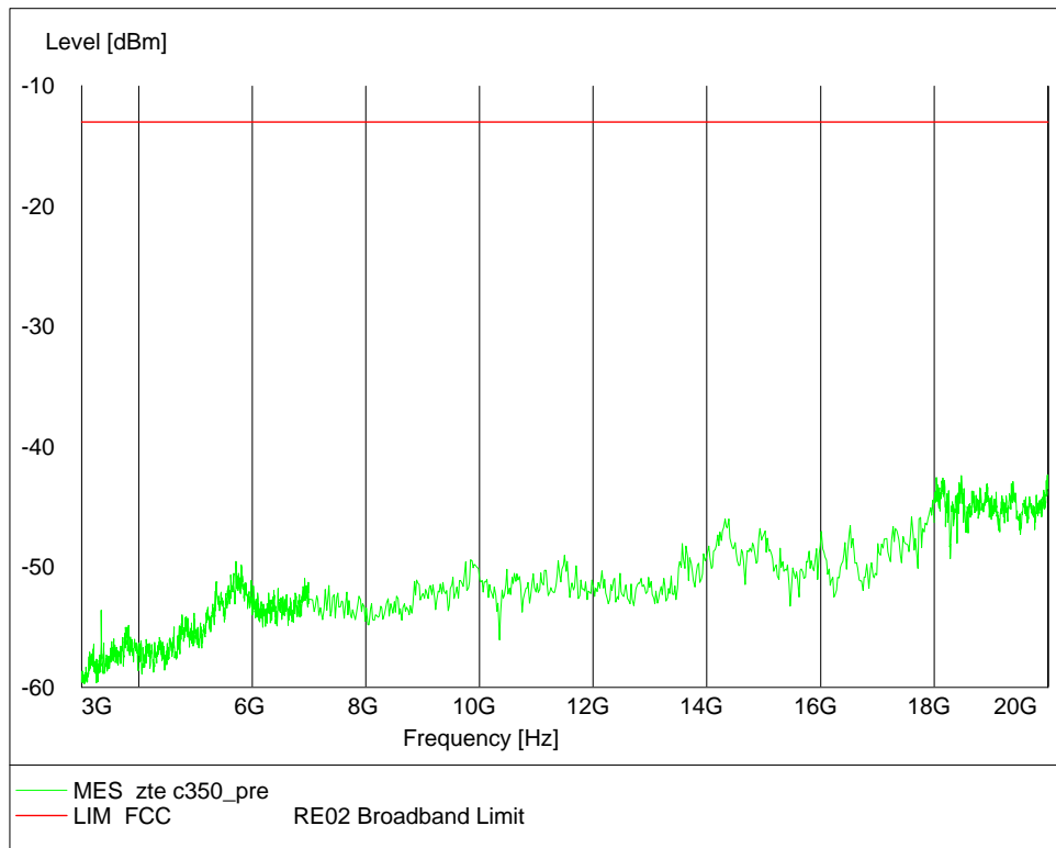
Channel 384, 3GHz~20GHz (Traffic Mode)
