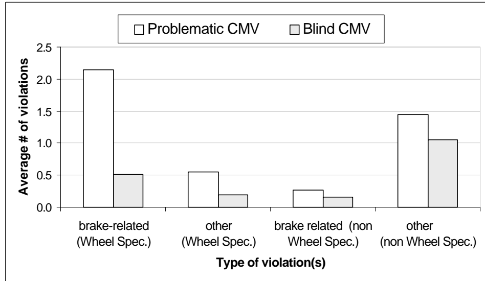
Figure 2. Average number of FMCSR violations reported in Level 1 inspections for CMVs screened with the IRISystem.
