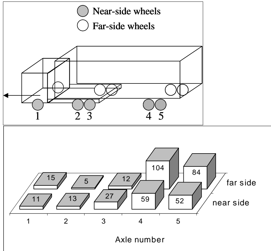
Figure 1. Number of problematic wheels identified by IRISystem as a function of wheel location on a 3-S2 CMV. The data are for all states. The arrow indicates the direction of the vehicle. The schematic illustrates the near-side and far-side wheel location as well as the axle numbers.
