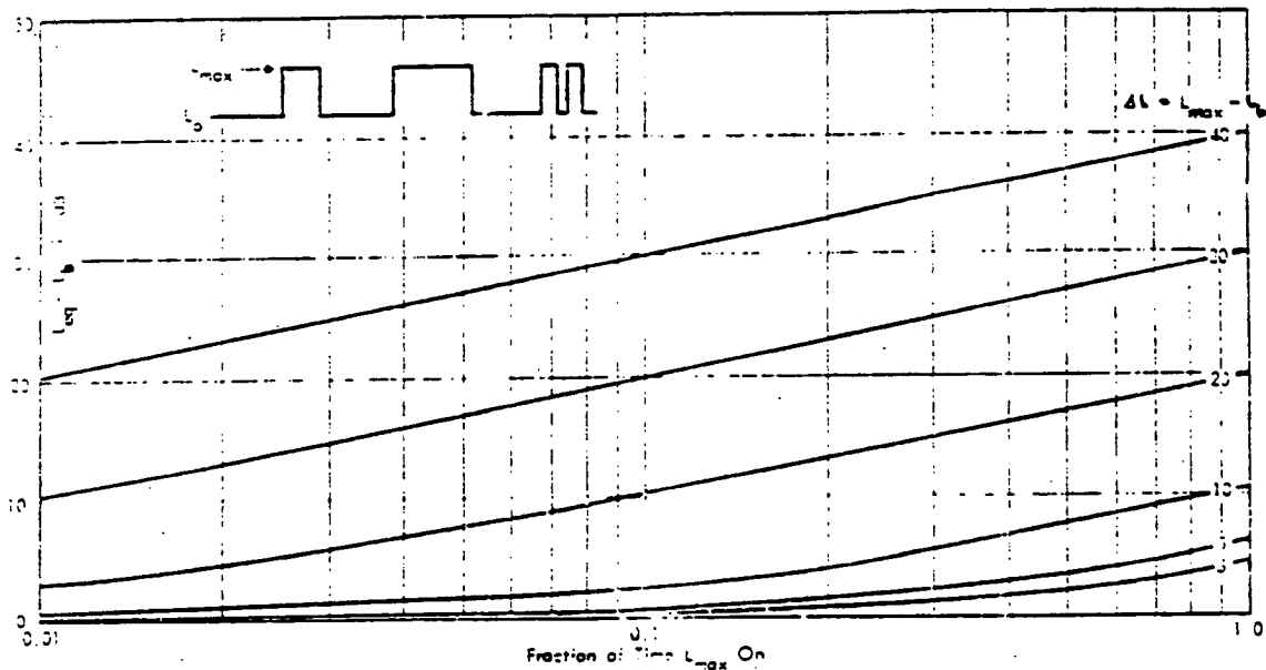
Figure A-1. L_{\text{eq}} for Intermittent L_{\max} Added to L_b A-25
