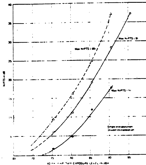
Figure C-5. NIPTS as a Function of Exposure Level for the 50th, 90th and 99th Percentiles
