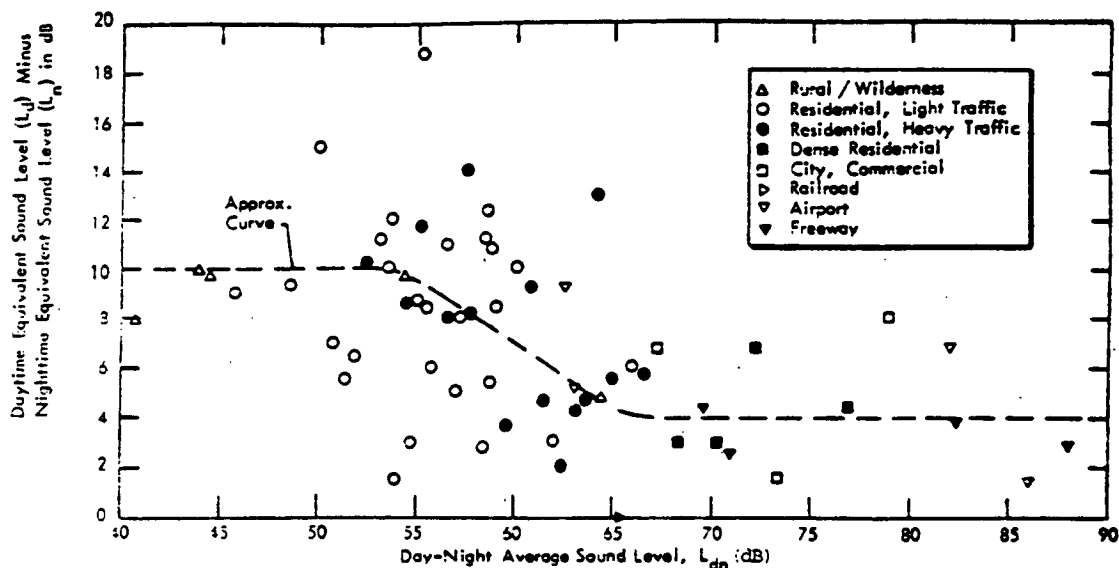
Figure A-7. Comparison of the Difference Between Day and Night Values of the Equivalent Sound Level with the Day-Night Average Sound Level, L_{dn} A-25
