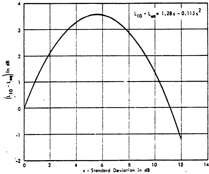
Figure A-6. Difference Between L_{10} and L_{eq} for a Normal Distribution A-25
