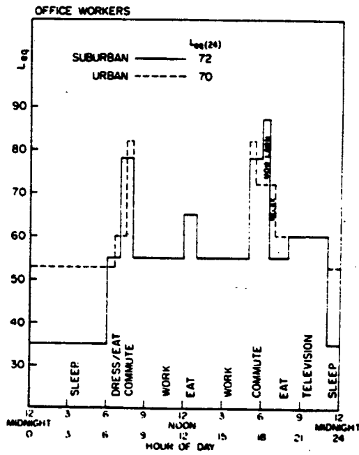
Figure B-4. Typical Noise Exposure Pattern of an Office Worker B-1,B-4,B-8,B-9
