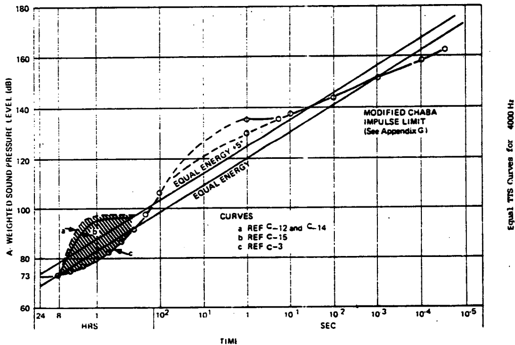
Figure C-6. Equal TTS Curves for 4000 Hz
