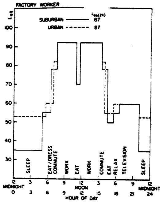
Figure B-3. Typical Noise Exposure Pattern of a Factory Worker B-1,B-4,B-8,B-9
