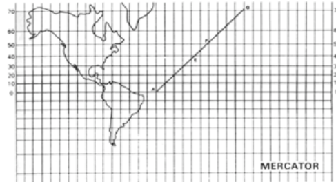
Figure 10. Mercator projection illustrating how a nonlinear distortion of the latitude scale can be used to straighten out the path traced by a rhumb line.
