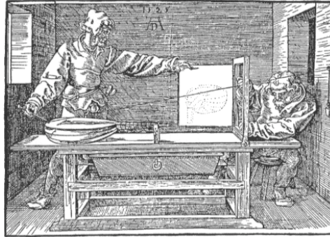
Figure 2. Woodcut by Dürer illustrating how to plot lines of sight with string in order to make a correct perspective projective © New York City Public Library
