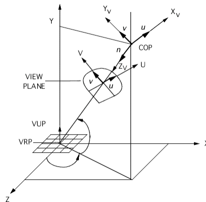
Figure 15. Illustration of the geometry of perspective projection showing the azimuth and the elevation of the viewing vector R , directed from the center of projection COP .
