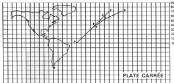
Figure 9. Plate carrée projection illustrating the curved path traced by a rhumb line on this format, i.e., line A E F G.
