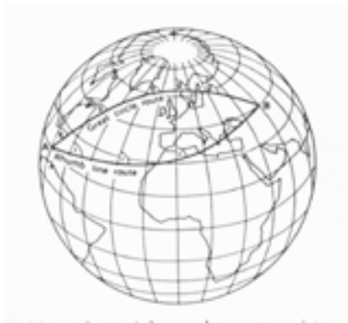
Figure 8. Rhumb-line and great-circle routes between two points on the globe. Note the constant bearing of the rhumb-line route and the constantly changing bearing of the great-circle route. On the globe the great-circle route is analogous to a straight line and direction Z is the azimuth of B from A.
