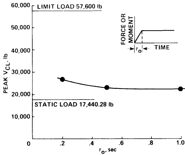
Fig. 27 Variation of rear-hook peak vertical load with braking condition.
