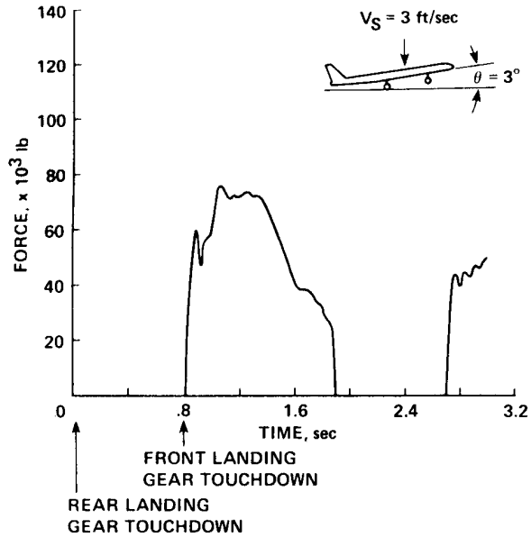
Fig. 5 Combined front landing gear force: V_S = 3 ft/sec, \theta = 3^\circ .
