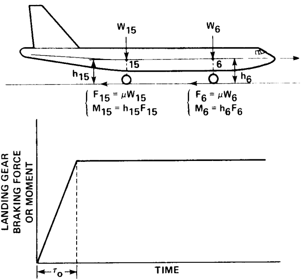
Fig. 7 Landing-gear braking force (or moment) curve.
