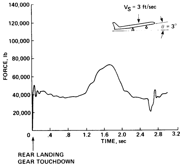
Fig. 6 Combined rear landing gear force: V_S = 3 ft/sec, \theta = 3^\circ .
