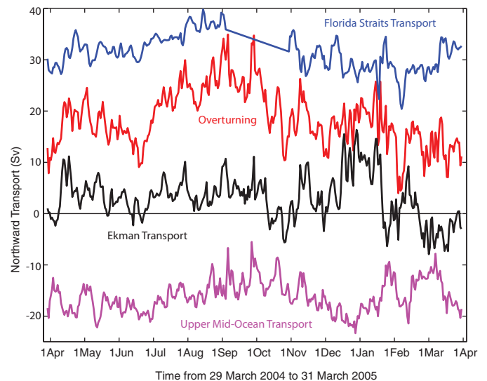
Fig. 3. Daily time series of Florida Straits transport (blue), Ekman transport (black), upper mid-ocean transport (magenta), and overturning transport (red) for the period 29 March 2004 to 31 March 2005. Florida Straits transport is based on electromagnetic cable measurements; a gap in the time series of ~2 months from 4 September to 28 October 2004 is due to Hurricane Frances, which destroyed the facility recording the voltage (linear interpolation is chosen here to fill the gap). Ekman transport is based on QuikScat-determined winds. The upper mid-ocean transport, based on the RAPID time series, is the vertical integral of the transport per unit depth down to the deepest northward velocity (~1100 m) on each day. Overturning transport is then the sum of the Florida Straits, Ekman, and upper mid-ocean transports and represents the maximum northward transport of upper-layer waters on each day (SOM text).
