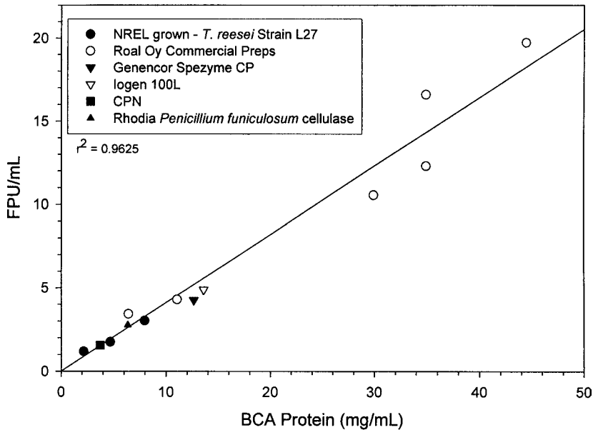
Fig. 3. Commercial and in-house-produced T. reesei cellulase preparations assayed for protein content and FPU activity plotted to determine correlation between the two factors. FPU's were determined using the standard FPA, and protein concentration was determined using the Pierce BCA method following desalting chromatography into 20 mM acetate, 100 mM NaCl, pH 5.0 buffer to remove interfering compounds.
