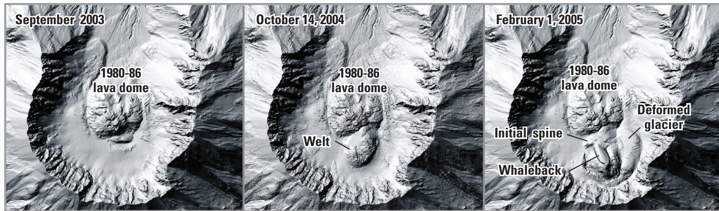
Topographic changes of the Mount St. Helens crater measured from aerial photographs and laser imaging (Lidar). Images show the rapid growth of the welt and new lava dome, the whaleback-shaped extrusion, and the deformed glacier. (October 14, 2004, image courtesy of NASA)
