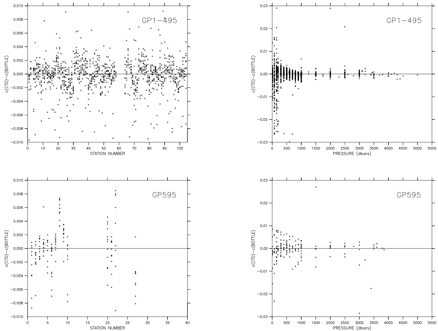
Fig. 2a. Calibrated CTD-bottle conductivity differences plotted against station number and pressure for cruises GP1-495 (upper panels) and GP595 (lower panels).
