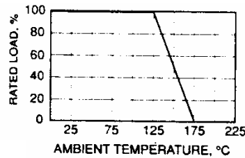
Figure 2. - Resistor derating (based on ambient "free air" operating environment).
