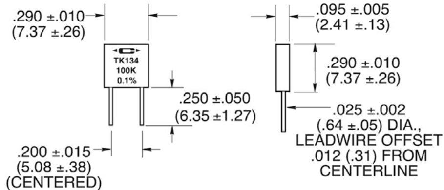
Figure 1. - Resistor outline drawing - inches (mm).
