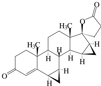
Drospirenone
