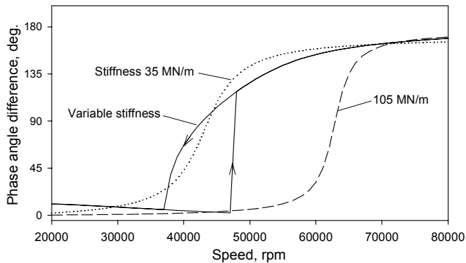
Figure 12. Phase angle difference between bearings
