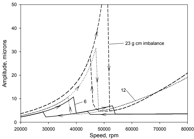
Figure 5. Station 10 amplitude
