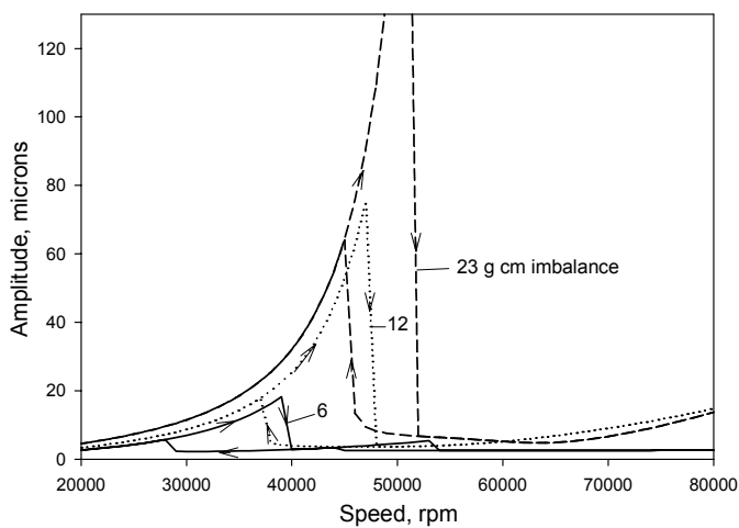
Figure 8. Station 7 amplitude
