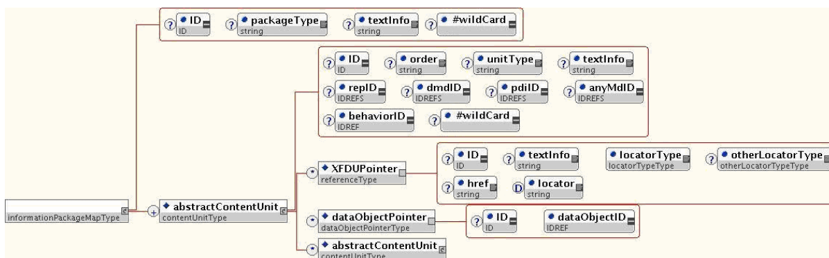
Figure 7-1: InformationPackageMapType Schema Diagram
