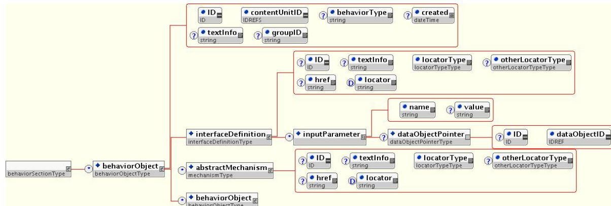
Figure 10-1: behaviorObjectType Schema Diagram
