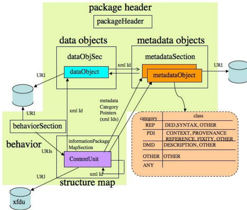
Figure 2-2: XFDU Manifest Logical View
