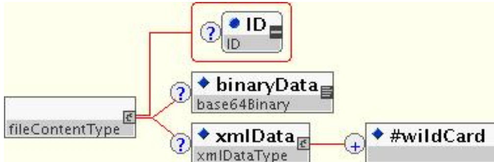
Figure 4-4: fileContentType/binaryData/xmlData 1 Schema Diagram
