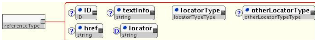
Figure 4-2: referenceType Schema Diagram
