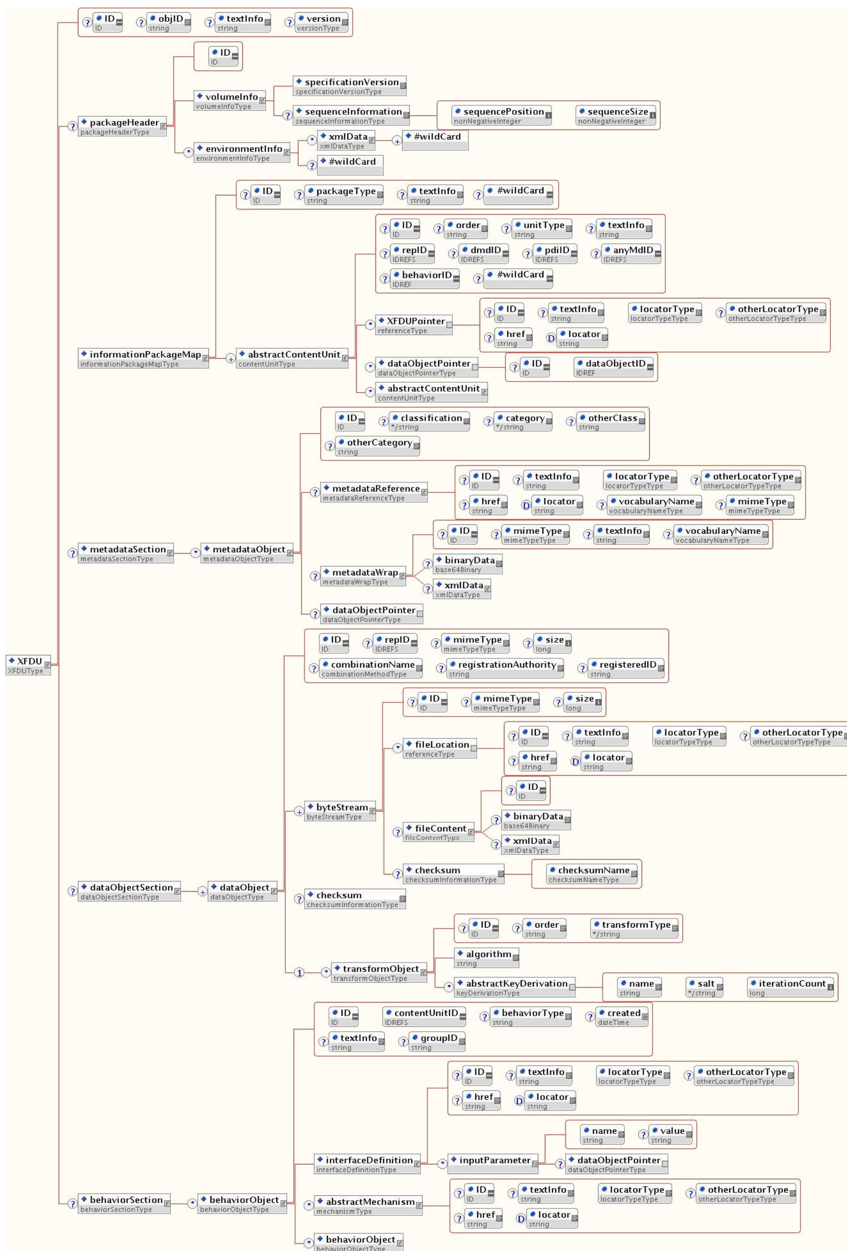
Figure 11-1: Full XFDU Schema Diagram
