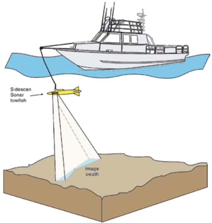
Deployment of sidescan sonar system with fan-shaped path perpendicular to vessel track-line.
