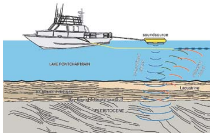
Seismic system collecting soundings from below seafloor.
