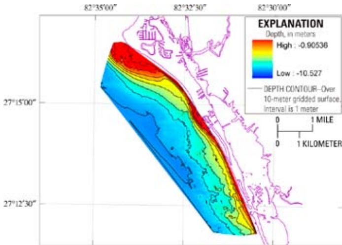
Bathymetric or water depth map created from single-beam soundings off Sarasota, Florida.
