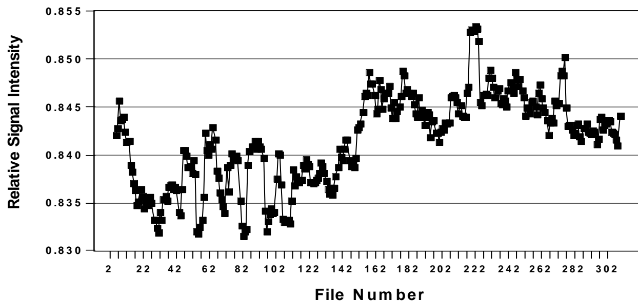
Figure 4. Relative single-beam signal intensity at 2500 cm -1 ratioed to that at 985 cm -1 .
