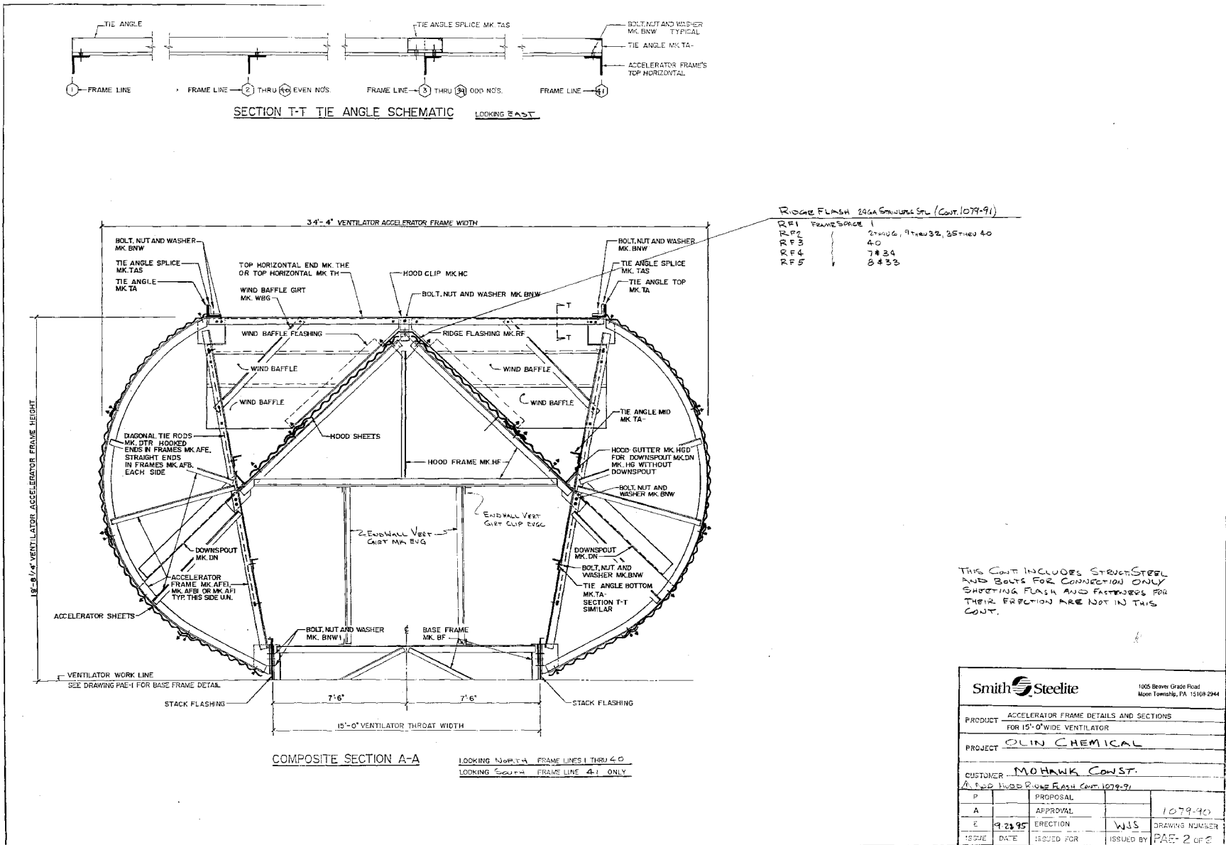
Figure 4-1. Cross-section of roof ventilator showing internal structure.
