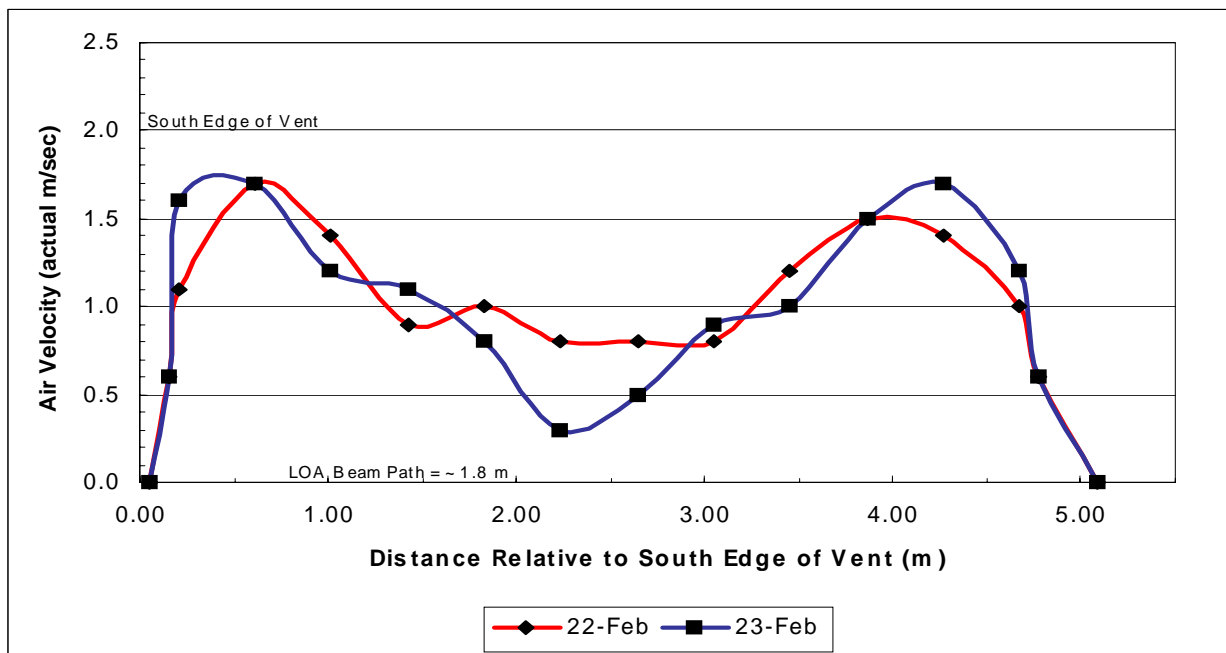
Figure 5-33. Hand-held anemometer readings at the optical anemometer measurement height on the west sampling platform, looking west.
