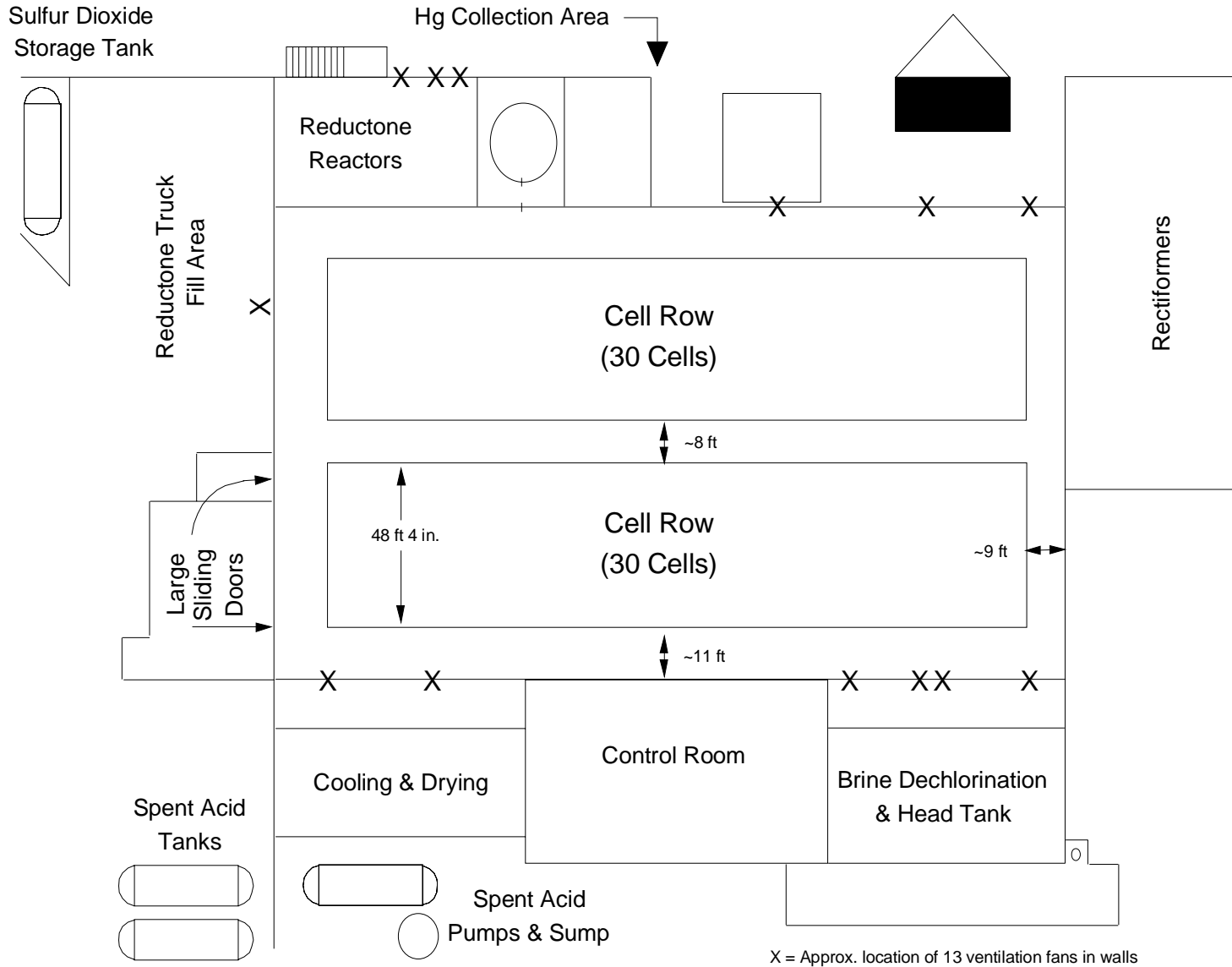
Figure 3-8. General diagram of the cell building showing cell rows, general fan locations, etc.
