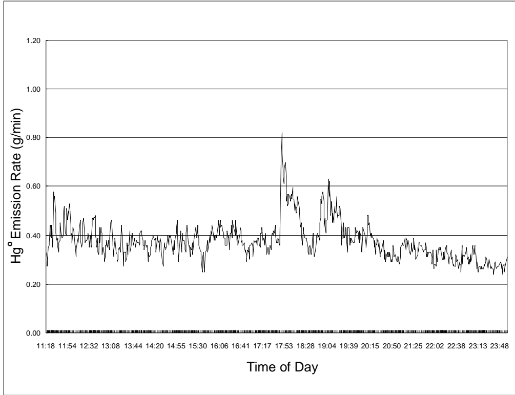
Figure 5-19. Elemental mercury emission rates for February 17, 2000.
