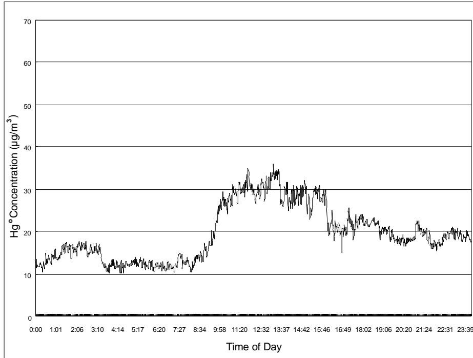
Figure 5-7. Time history of roof vent elemental mercury concentration for February 23, 2000.
