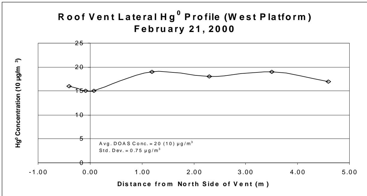
Figure 5-28. Lateral profile of elemental mercury concentration as determined by the Jerome 431-X instrument.
