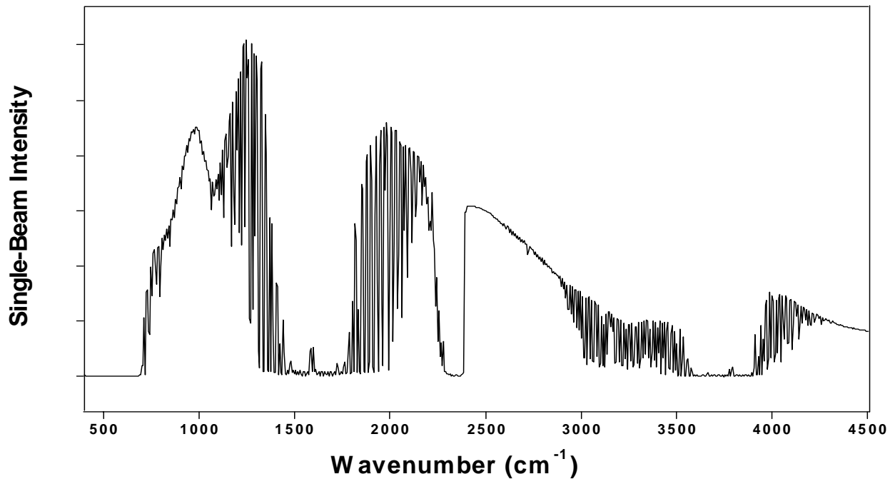
Figure 2. Single-beam OP/FTIR spectrum collected at Research Triangle Park with a 414-m pathlength.
