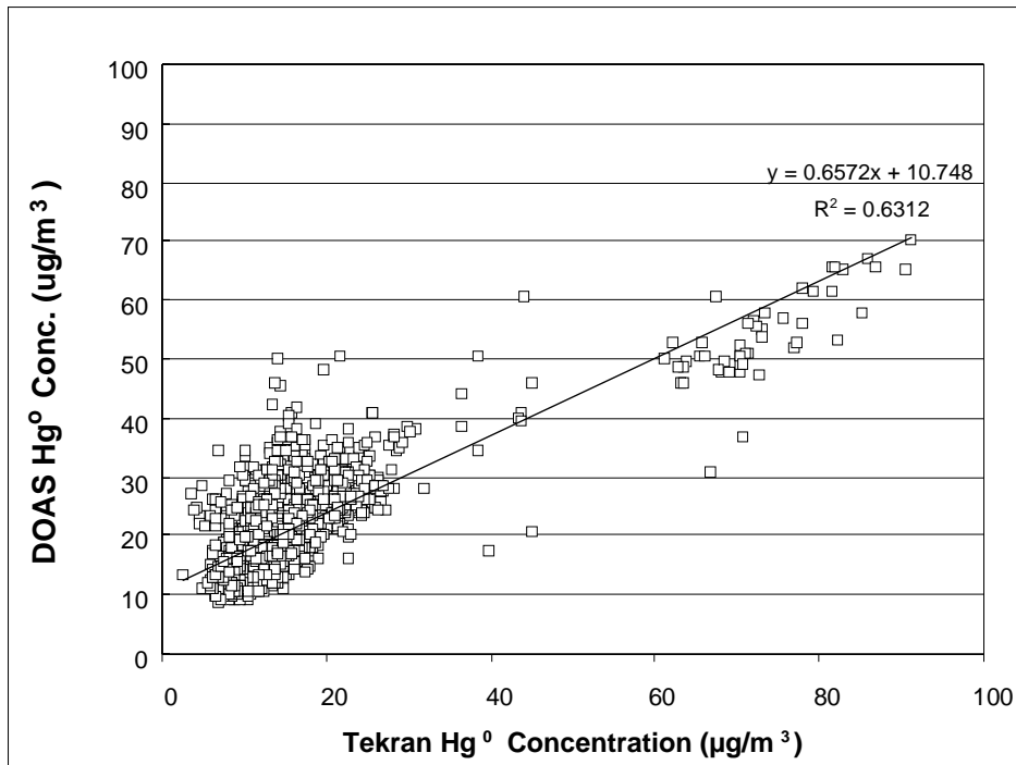
Figure 5-29. UV-DOAS/Tekran comparison (February 17-21, 2000).
