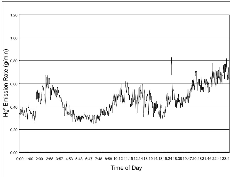
Figure 5-26. Elemental mercury emission rates for February 24, 2000.
