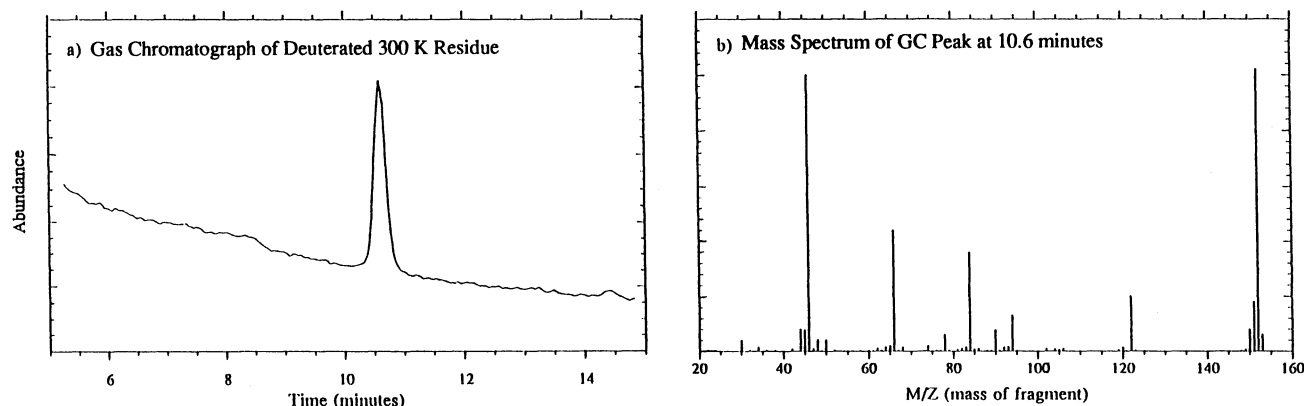
FIG. 5.—(a) Gas chromatograph and (b) mass spectrum of the residue generated from UV photolysis of a \text{D}_2\text{O}:\text{CD}_3\text{OD}:\text{CO}:\text{ND}_3 = 100:50:10:10 mixture that was subsequently warmed to 300 K. The parent mass peak at 152 indicates that fully deuterated HMT was produced upon photolysis and warming.
