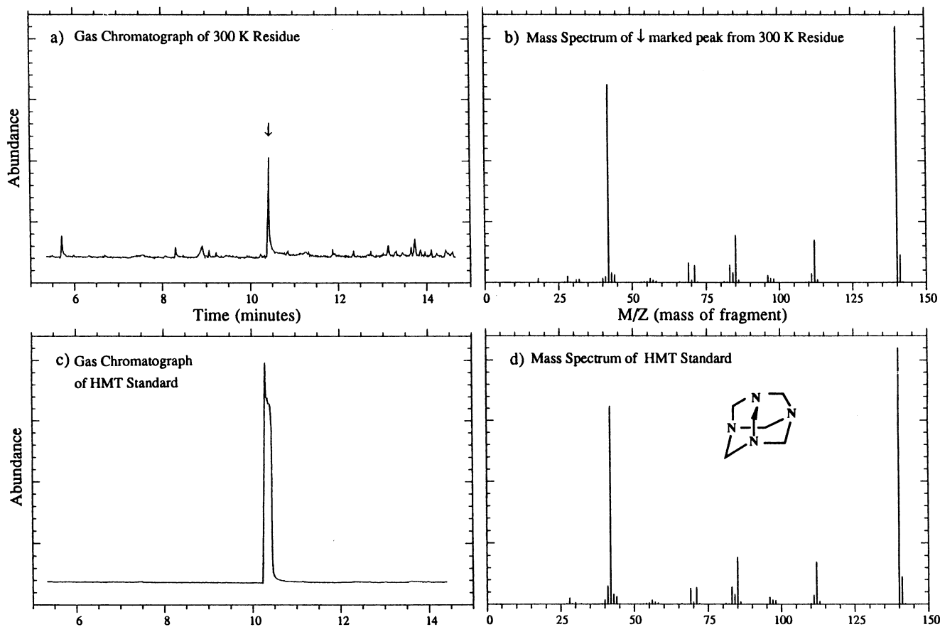
FIG. 3.—Gas chromatographs and mass spectra of the refractory residue produced by the irradiation of an \text{H}_2\text{O}:\text{CH}_3\text{OH}:\text{CO}:\text{NH}_3 = 100:50:10:10 ice followed by warming to 300 K compared to a sample of pure hexamethylenetetramine (HMT). The gas chromatographs of the residue and HMT standard are shown in panels (a) and (c), respectively, and the corresponding mass spectra of the most prominent peaks (retention time of about 10.2 minutes) are shown in (b) and (d). The structure of HMT is given in (d).
