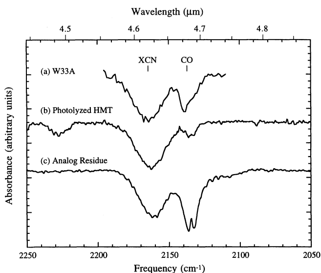
FIG. 9.— 2250\text{--}2050\text{ cm}^{-1} ( 4.44\text{--}4.88\text{ }\mu\text{m} ) infrared spectrum of (a) W33A, a protostar deeply embedded in an interstellar cloud of dust, gas, and ice (see Lacy et al. 1984), (b) HMT photolyzed in \text{H}_2\text{O} ( \text{H}_2\text{O}/\text{HMT} \approx 3 ) at 12 K and subsequently warmed to 150 K (taken from Bernstein et al. 1994), and (c) the residue produced when an \text{H}_2\text{O}:\text{CH}_3\text{OH}:\text{CO}:\text{NH}_3 = 100:50:10:10 ice is photolyzed at 12 K and subsequently warmed to 150 K.
