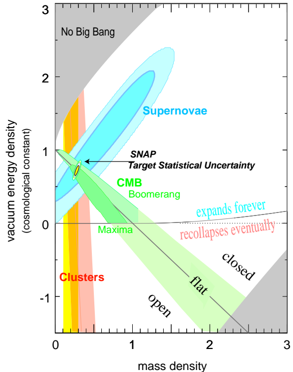
Fig. 1.— There is strong evidence for the existence of a cosmological vacuum energy density. Plotted are \Omega_M – \Omega_\Lambda confidence regions for current SN (Perlmutter et al. 1999), galaxy cluster, and CMB results. These results rule out a simple flat, [ \Omega_M = 1 , \Omega_\Lambda = 0 ] cosmology. Their consistent overlap is a strong indicator for dark energy. Also shown is the expected confidence region from the SNAP satellite for an \Omega_M = 0.28 flat Universe.
