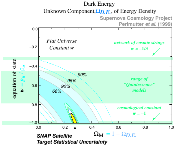
Fig. 2.— Best-fit 68%, 90%, 95%, and 99% confidence regions in the \Omega_M - w plane for an additional energy density component, \Omega_w , characterized by an equation-of-state w = p/\rho . (For Einstein’s cosmological constant, \Lambda , w = -1 .) The fit is constrained to a flat cosmology ( \Omega_M + \Omega_w = 1 ). Also shown is the expected confidence region allowed by SNAP assuming w = -1 and \Omega_M = 0.28 .
