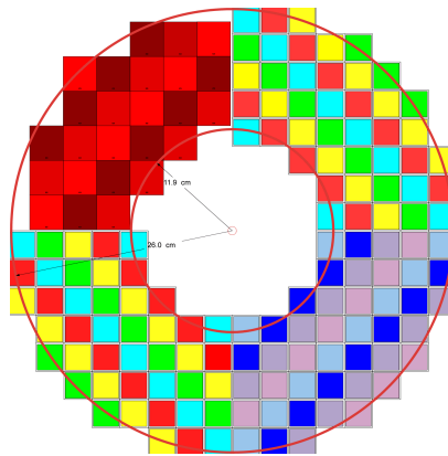
Fig. 6.— The CCD mosaic camera is tiled with 132 \ 3k \times 3k high-resistivity CCD's and 25 HgCdTe detectors and covers one square degree. The annular shape is necessary in a simple three-mirror anastigmat telescope design.
