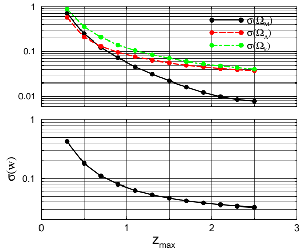
Fig. 4.— Accuracy in parameter estimation as a function of maximum redshift probed in SN Ia surveys. Shown is the statistical uncertainty in the determination of the cosmological parameters \Omega_M , \Omega_\Lambda , and \Omega_k (upper panel; knowledge of w assumed) and equation of state ratio w (lower panel; flat Universe assumed) each as a function of maximum redshift probed z_{\max} . Approximately 2400 supernovae distributed from z = 0 to z_{\max} are assumed in each case with statistical uncertainties only. Exploring redshifts between 0 and 1.7 is optimal, since this is where most of the dark energy action occurs. Going to redshifts beyond z \sim 1.8 would bring very little improvement in parameter-determination accuracy, as the dark energy is expected to be dynamically unimportant at such high redshifts.
