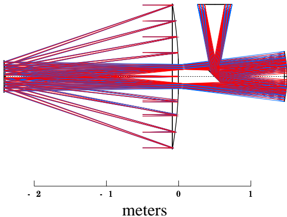
Fig. 5.— Side view of our baseline optical configuration, with a 2.0 meter primary mirror, a 0.45 meter secondary mirror, a folding flat, and a 0.7 meter tertiary mirror.
