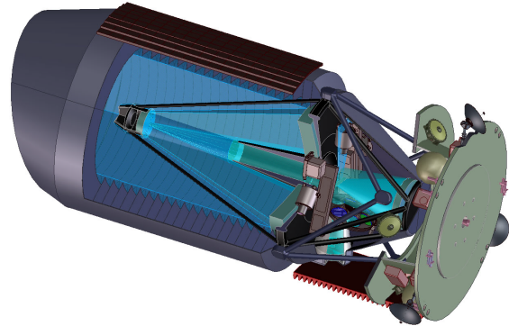
Fig. 3.— A cross-sectional view of the SNAP satellite. The principal assembly components are the telescope, optical bench, instruments, propulsion deck, bus, and thermal shielding.
