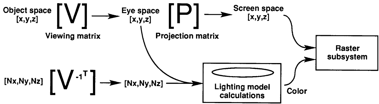
Figure 6. Lighting calculation.
