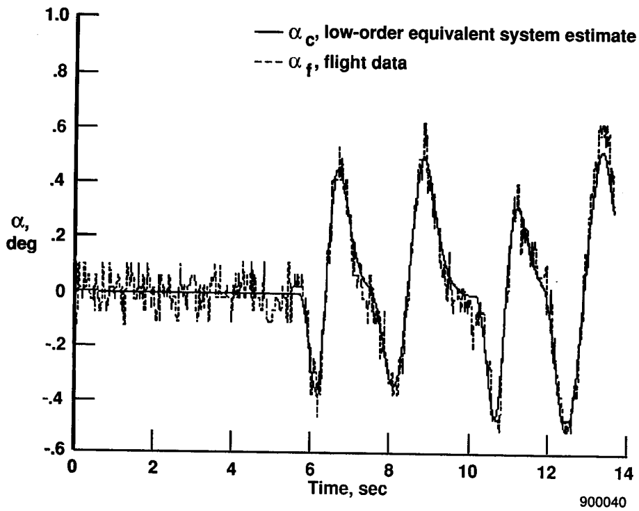
(a) Angle of attack.
