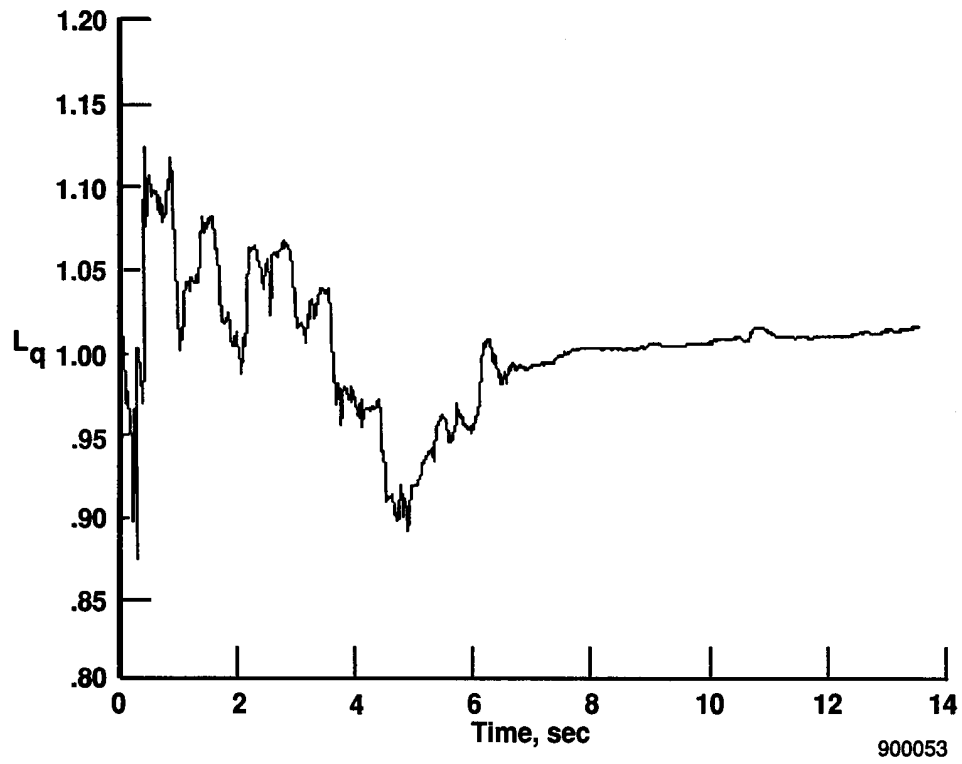
(h) L_q .
