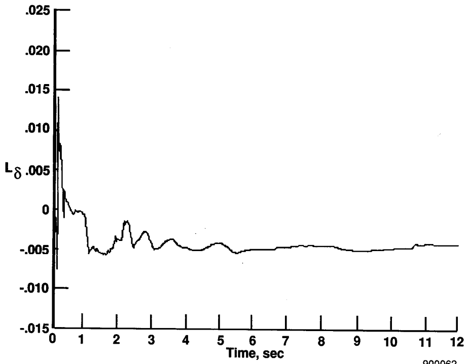
(c) L_{\delta} .
