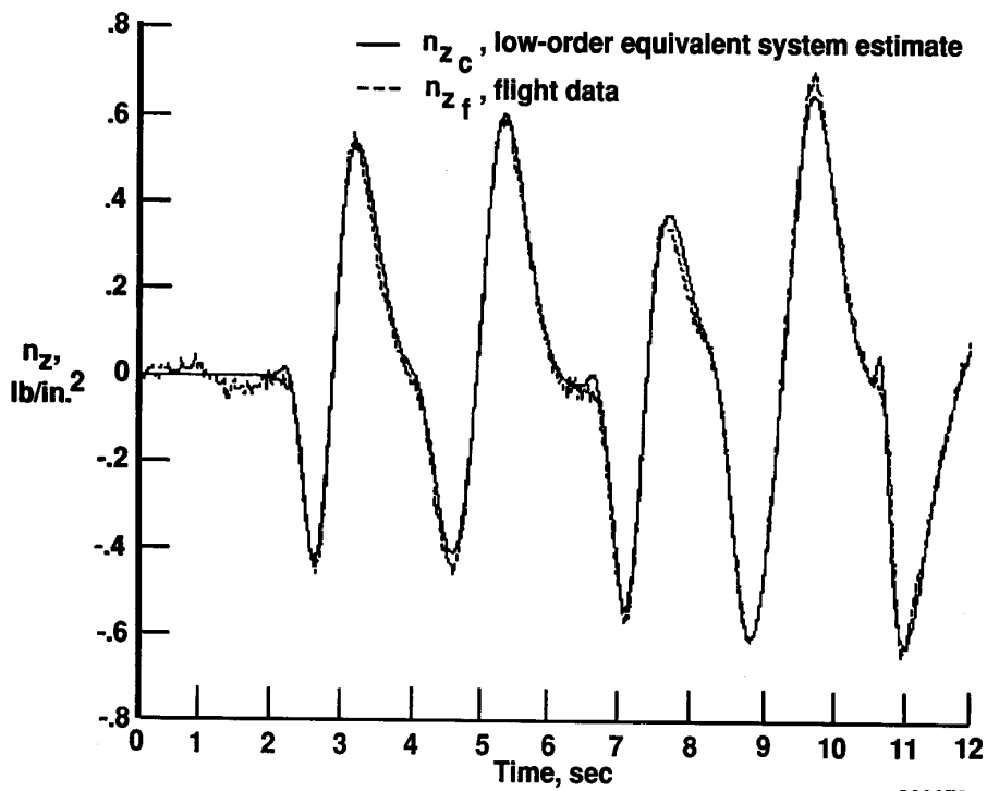
(c) Normal acceleration.
