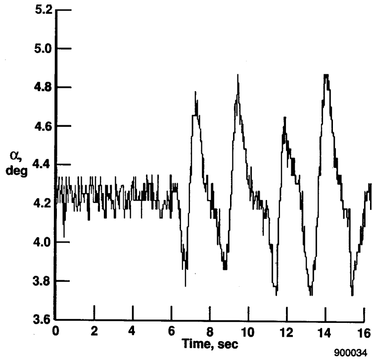
(b) Angle of attack.
