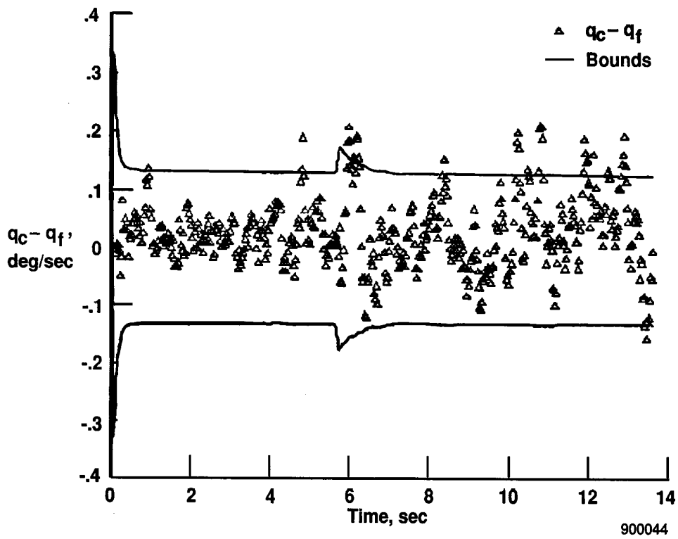
(b) Pitch rate.
