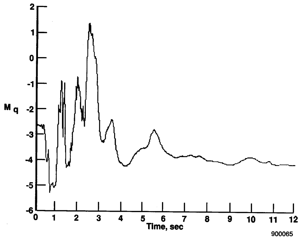
(f) M_q .
