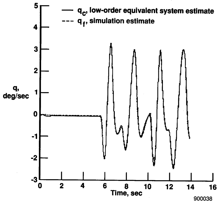
(b) Pitch rate.
