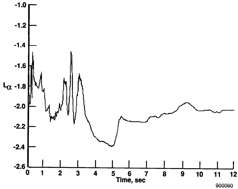
(a) L_{\alpha} .
