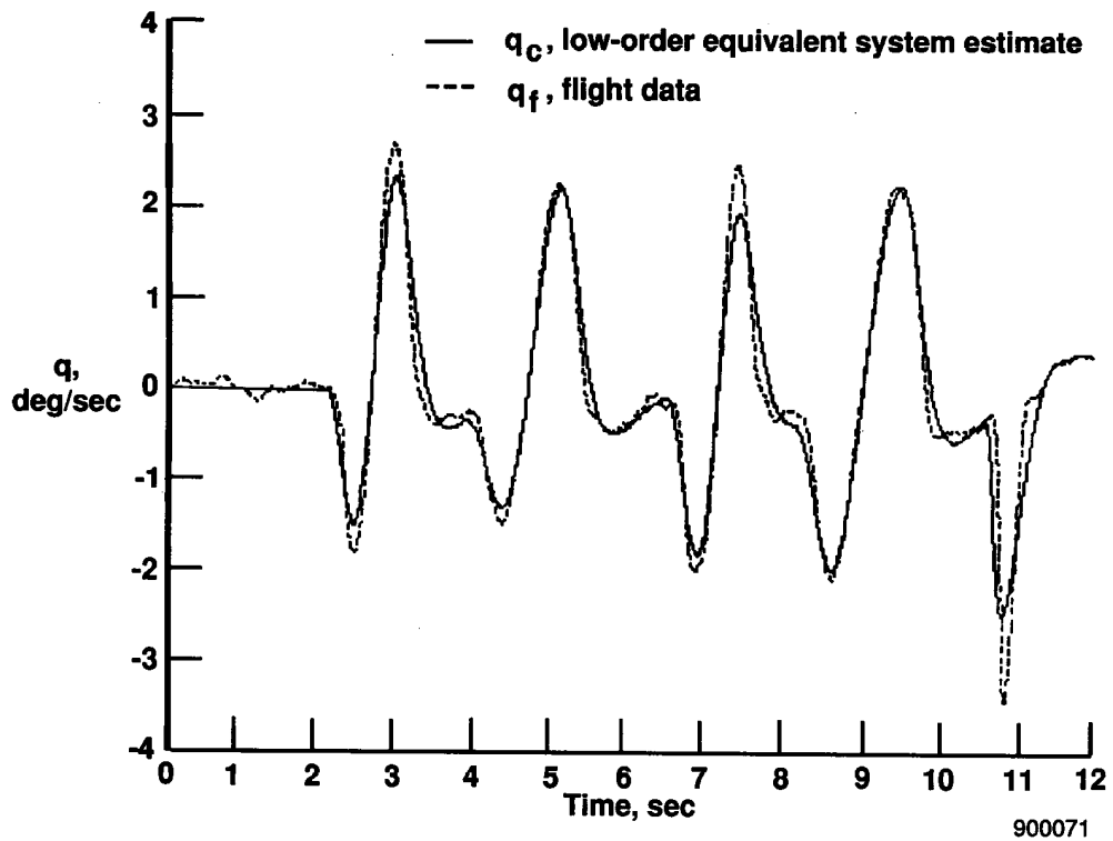
(b) Pitch rate.
