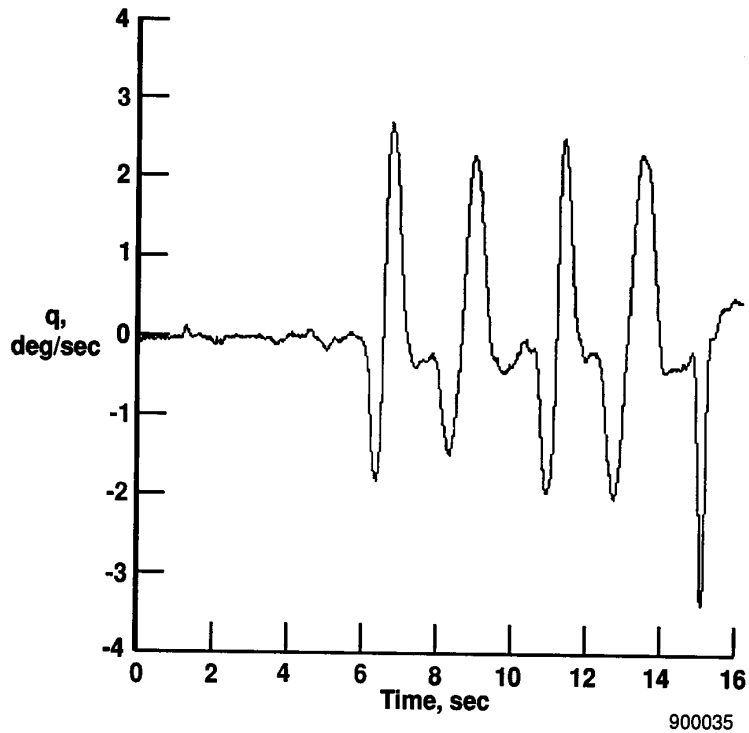
(c) Pitch rate.
