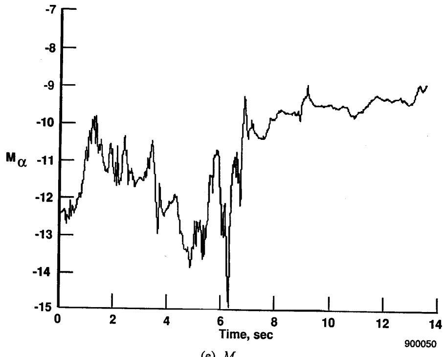
(e) M_\alpha .
