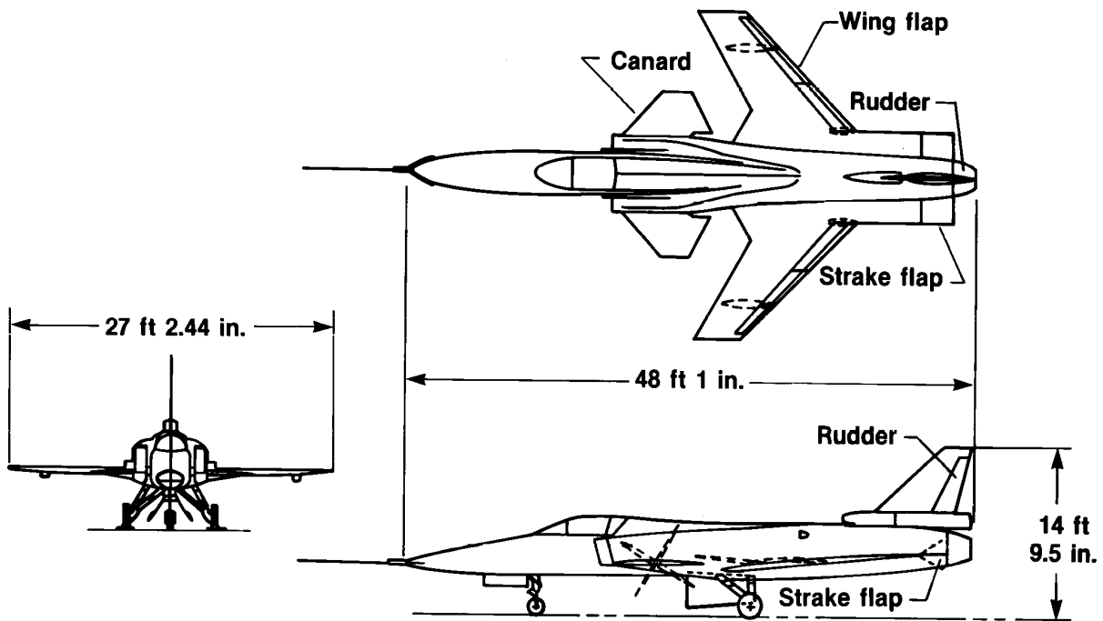
Fig. 1 The X-29A airplane.
