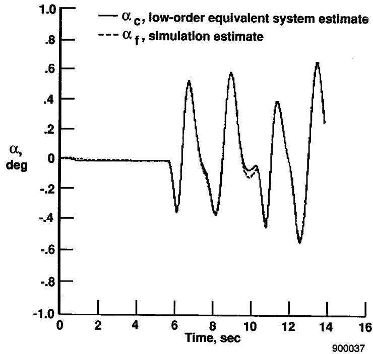
(a) Angle of attack.
