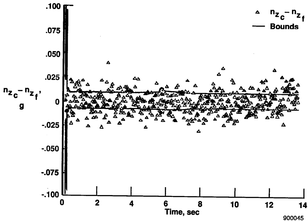
(c) Normal acceleration.
