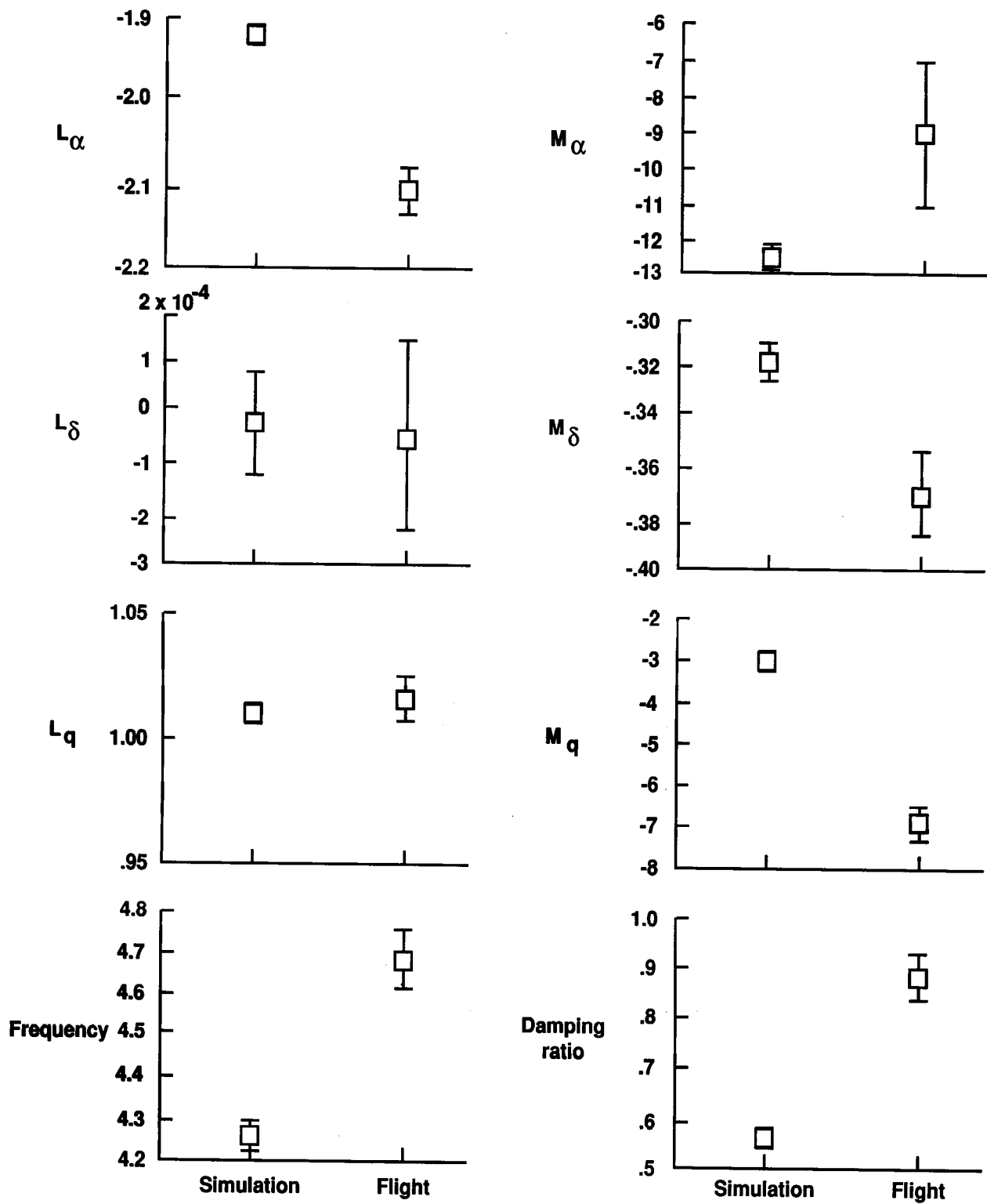
Fig. 8 Simulation results compared with flight data.
