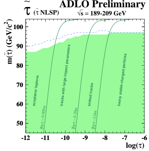
Fig. 2. Excluded mass as a function of \tilde{\tau}_1 lifetime. Expected limit and lines of equal \beta\gamma c\tau are shown, the latter to indicate the different lifetime regimes.
