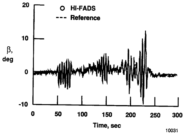
(a) Comparison of HI-FADS and reference angle of sideslip.
