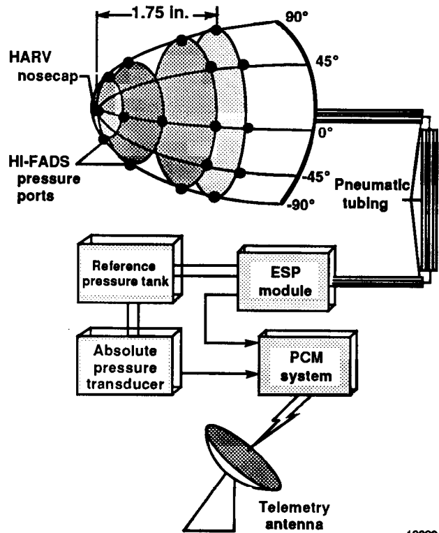
Fig. 2 The HI-FADS system hardware.
