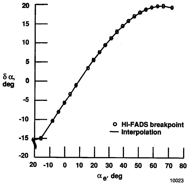
Fig. 5 Calibration results for effective angle-of-attack parameter.
