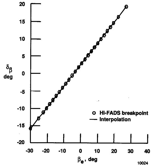
Fig. 6 Calibration results for effective angle-of-sideslip parameter.
