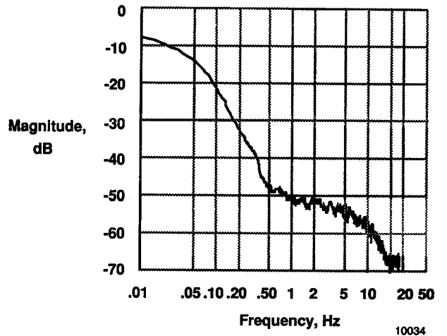
Fig. 13 The HI-FADS data PSD for Mach number.
