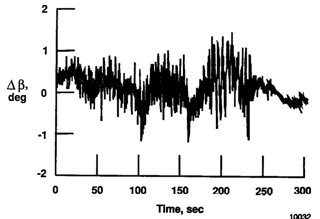
(b) Residual difference between HI-FADS and reference.
