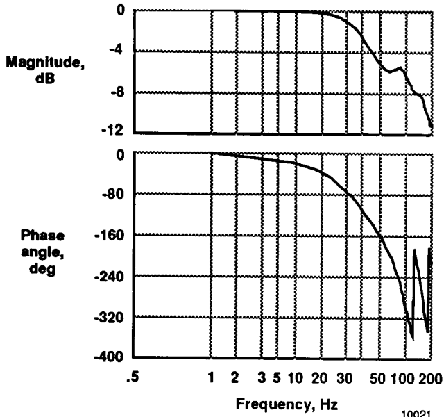
Fig. 3 Analytical predictions of the frequency response.
