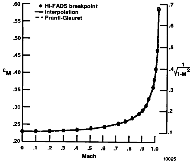
Fig. 7 Calibration results for \epsilon_M parameter.
