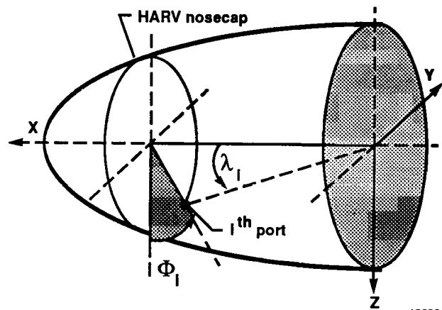
Fig. 4 Coordinate definitions of the i th HI-FADS pressure port.
