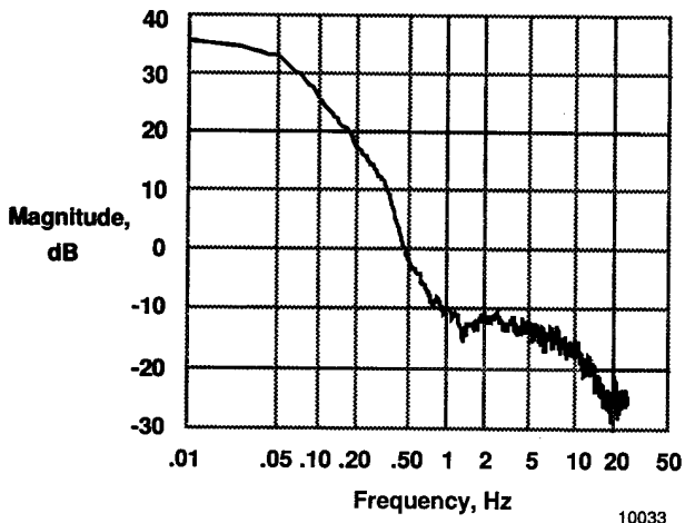
Fig. 12 The HI-FADS data PSD for angle of attack.
