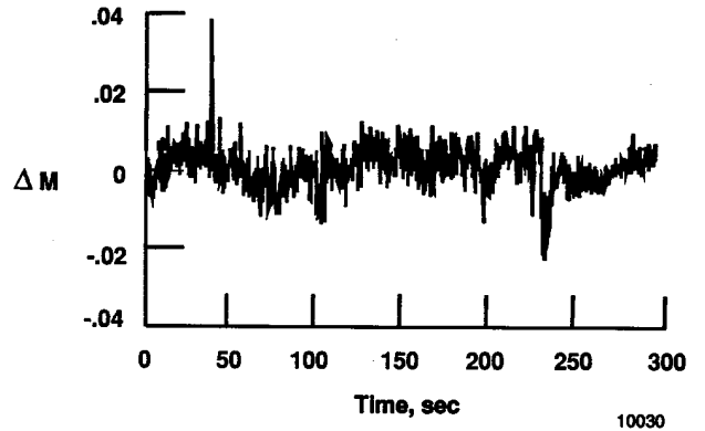
(b) Residual difference between HI-FADS and reference.
