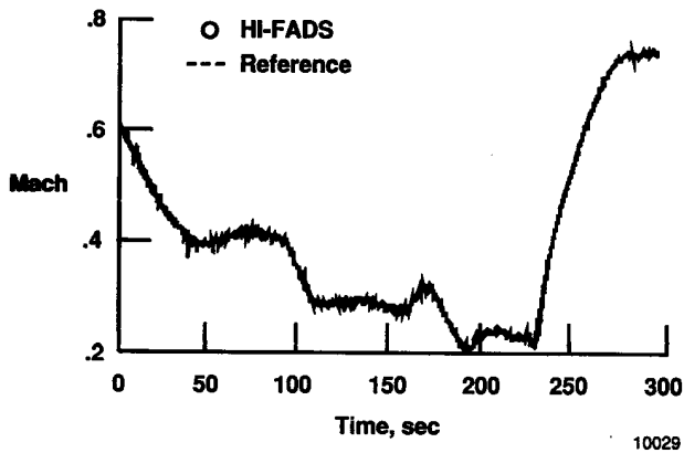
(a) Comparison of HI-FADS and reference Mach number.
