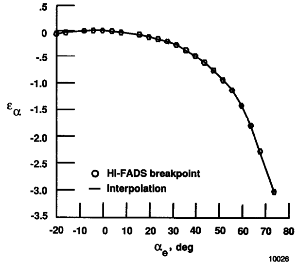
Fig. 8 Calibration results for \epsilon_\alpha parameter.
