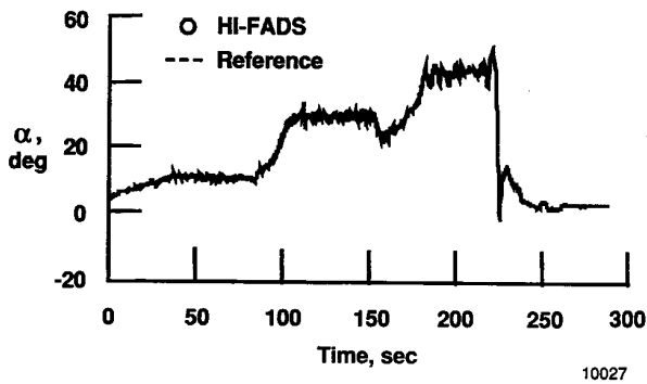
(a) Comparison of HI-FADS and reference angle of attack.
