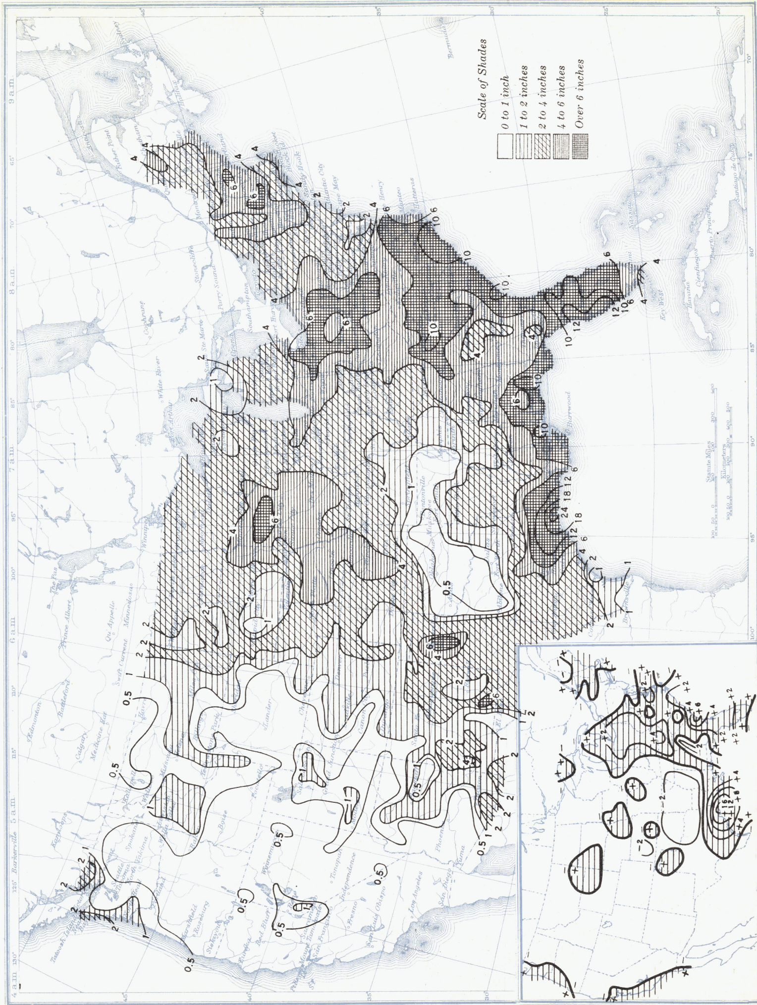
Chart V. Total Precipitation, Inches, July 1943. (Inset) Departure of Precipitation from Normal
