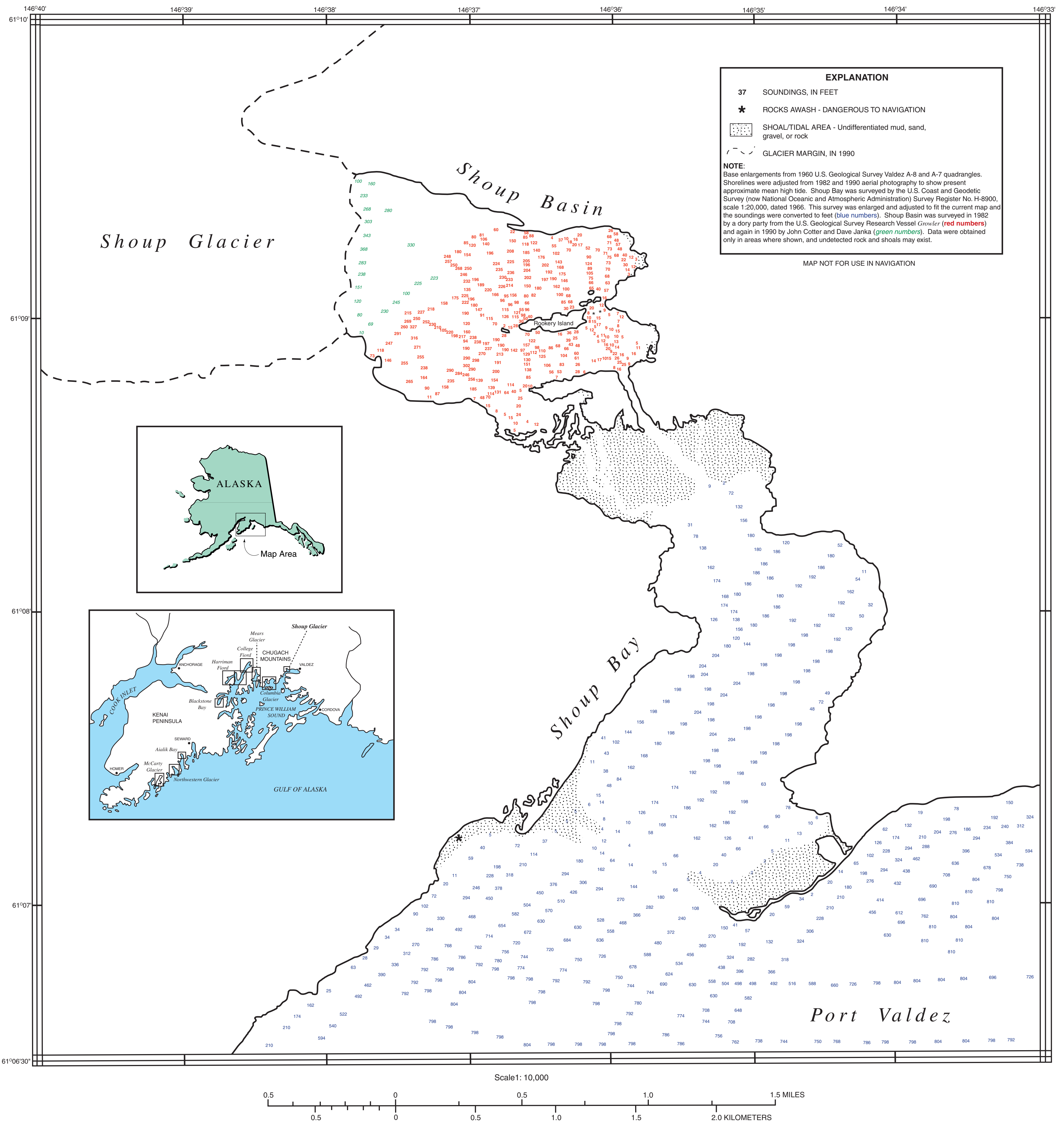
MAP SHOWING SOUNDINGS IN SHOUP BAY, SHOUP BASIN, AND PORT VALDEZ, ALASKA by Austin Post and Robert J. Viens 2000
