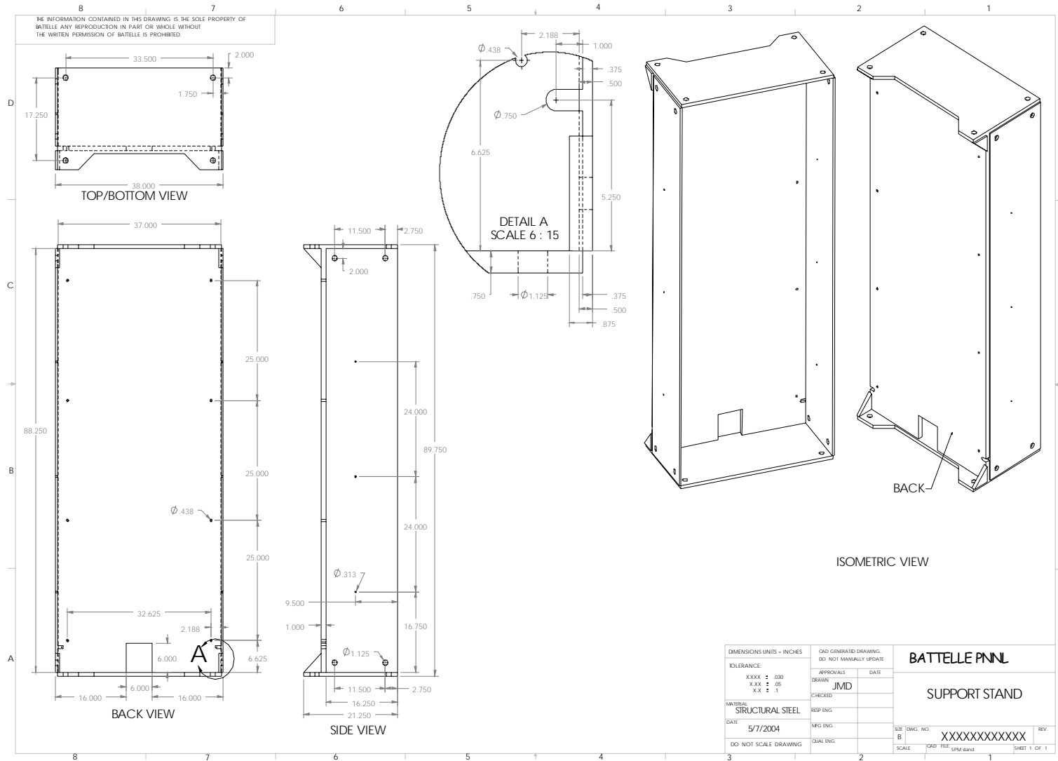
Figure 5.1. Support Structure Drawing
