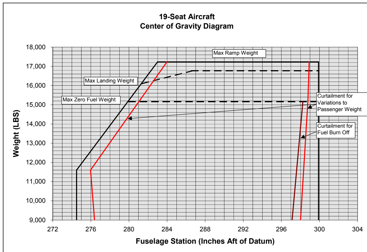
FIGURE 6-2. OPERATIONAL CG ENVELOPE—ACTUAL PASSENGER SEATING
