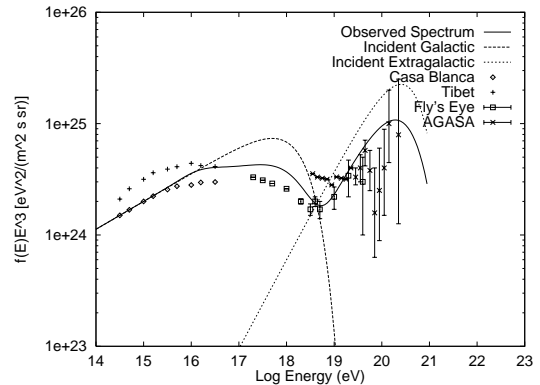
FIG. 1. The cosmic ray spectrum f(E) multiplied by E^3 for E > 10^{14} eV. Long and short dashed lines are respectively the incident galactic and extragalactic components. Solid line is the combined spectrum expected to be measured for y = 1/2 , \alpha = 2 . +’s are the Tibet data, diamonds the Casa Blanca data, squares the Fly’s Eye data and x’s the AGASA data.
