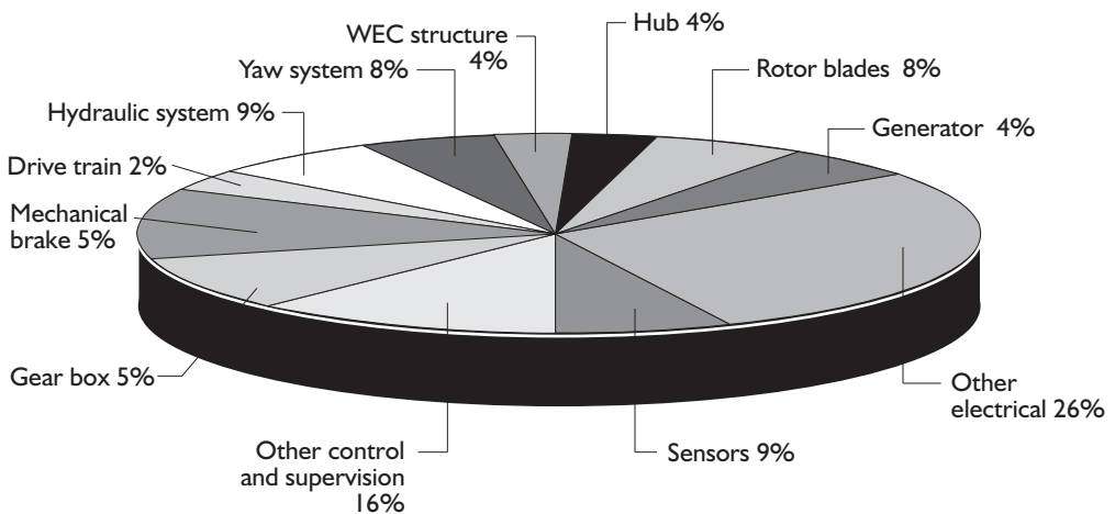
Figure 13.2 Failure and repair statistics for all WECs in the WMEP program
