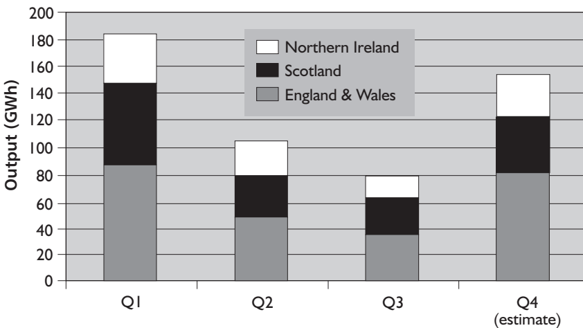
Figure 22.2 Wind energy output from current NFFO contracts during 2000
