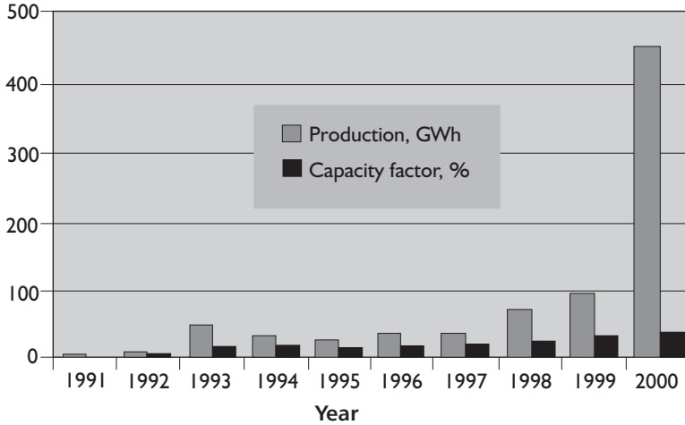
Figure 14.2 Electricity produced and capacity factor for wind turbines in Greece
