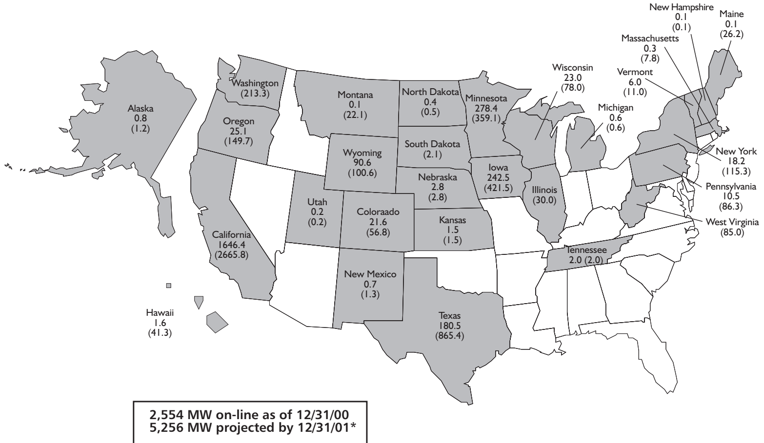
Figure 23.1 Wind power plant installed capacity in the United States at the end of 2000 and projected by the end of 2001
