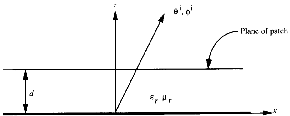
(b) Cross section of patch.
