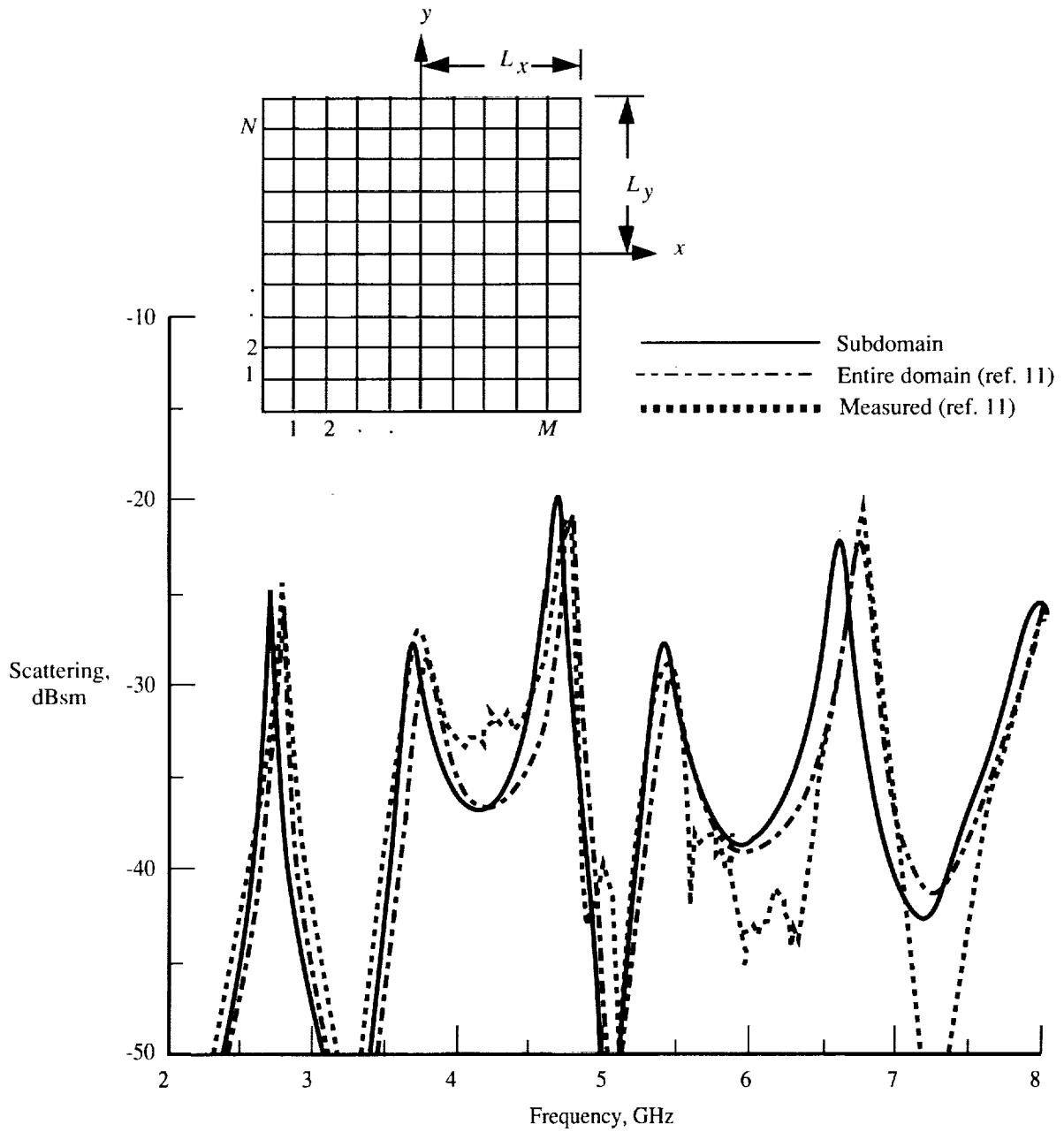
Figure 2. Comparison between subdomain, entire-domain, and measured scattering from a rectangular microstrip patch antenna. L_x = 1.88 cm; L_y = 1.30 cm; d = 0.158 cm; \epsilon_r = 2.17 ; Loss tangent = 0.001; \theta^i, \phi^i = 60^\circ, 45^\circ .
