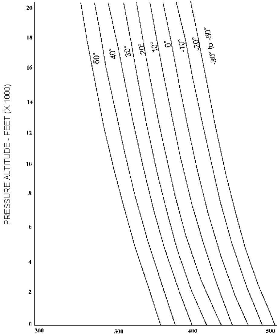
SHAFT HORSEPOWER AVAILABLE
