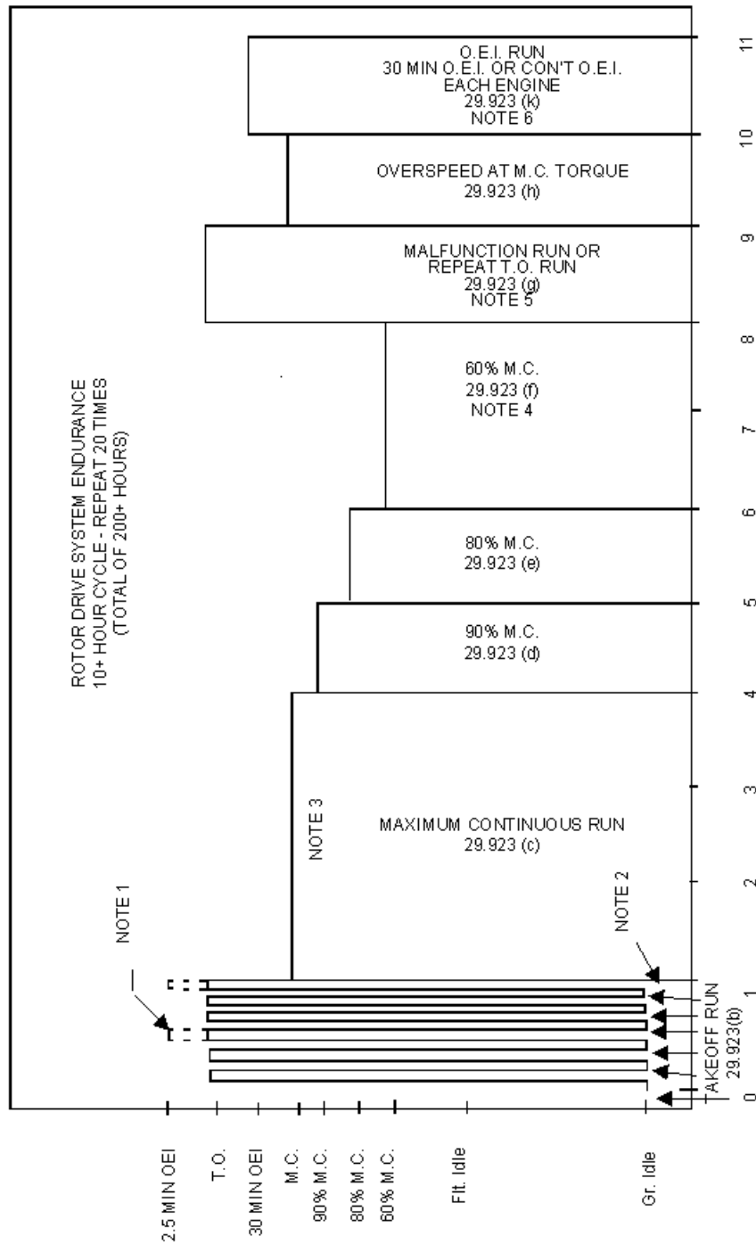
TIME - HOURS FIGURE AC 29.923A-1
