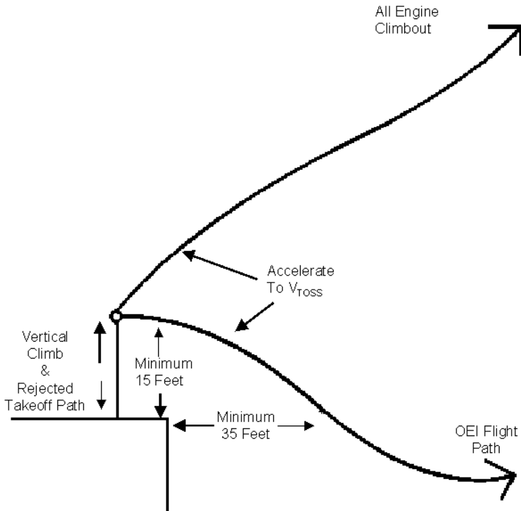
FIGURE AC 29.59-2 CATEGORY A VERTICAL TAKEOFF PROFILE PINNACLE
