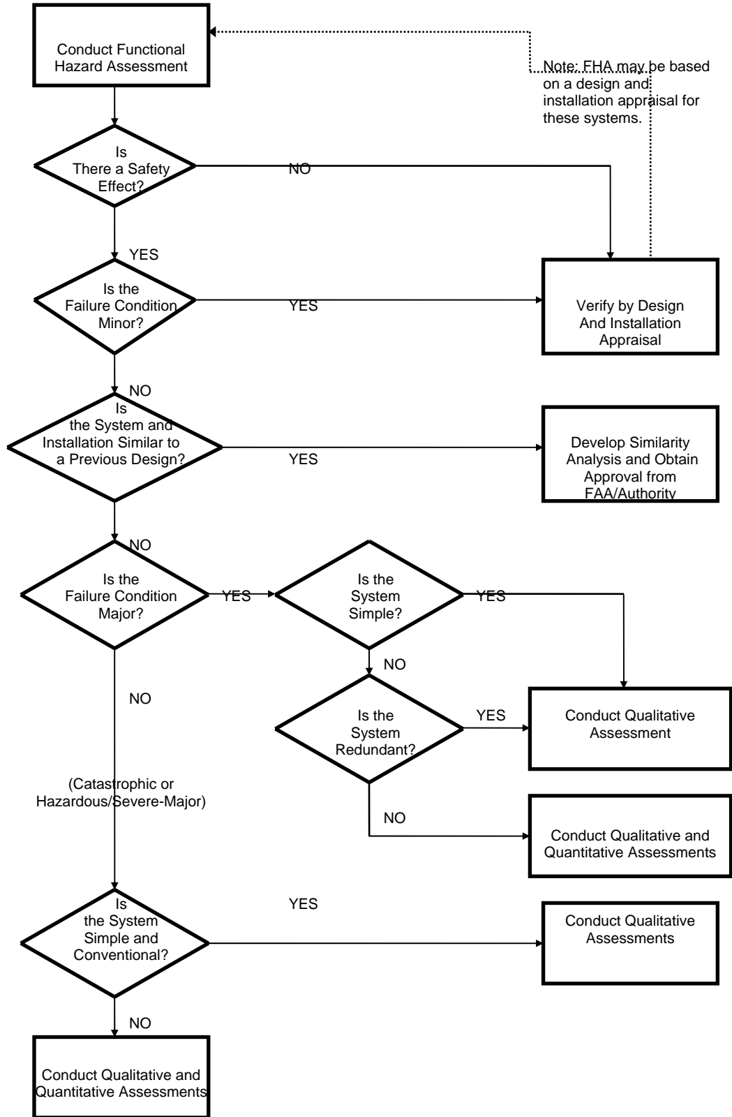
FIGURE AC 29.1309-5: Depth of Analysis Flowchart
