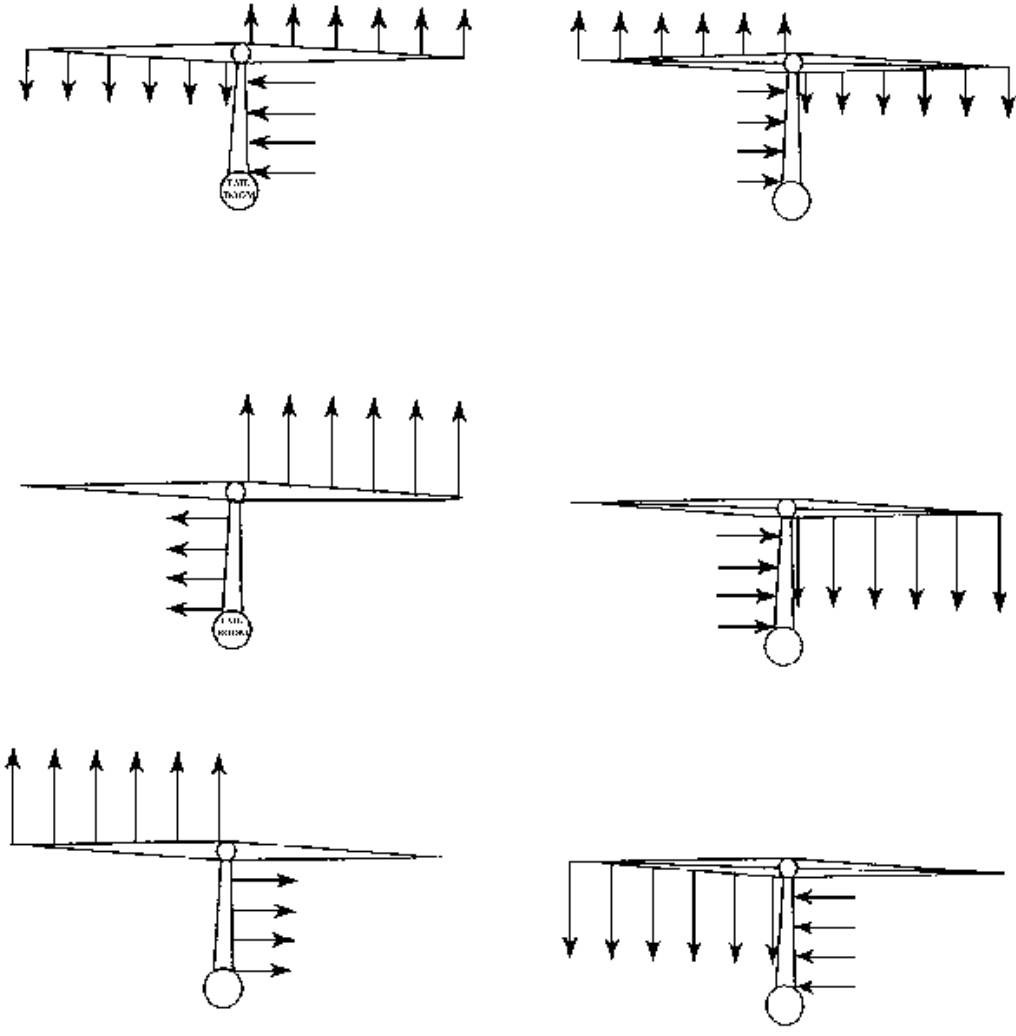
Figure AC 29.427-2 (View Looking Forward)
