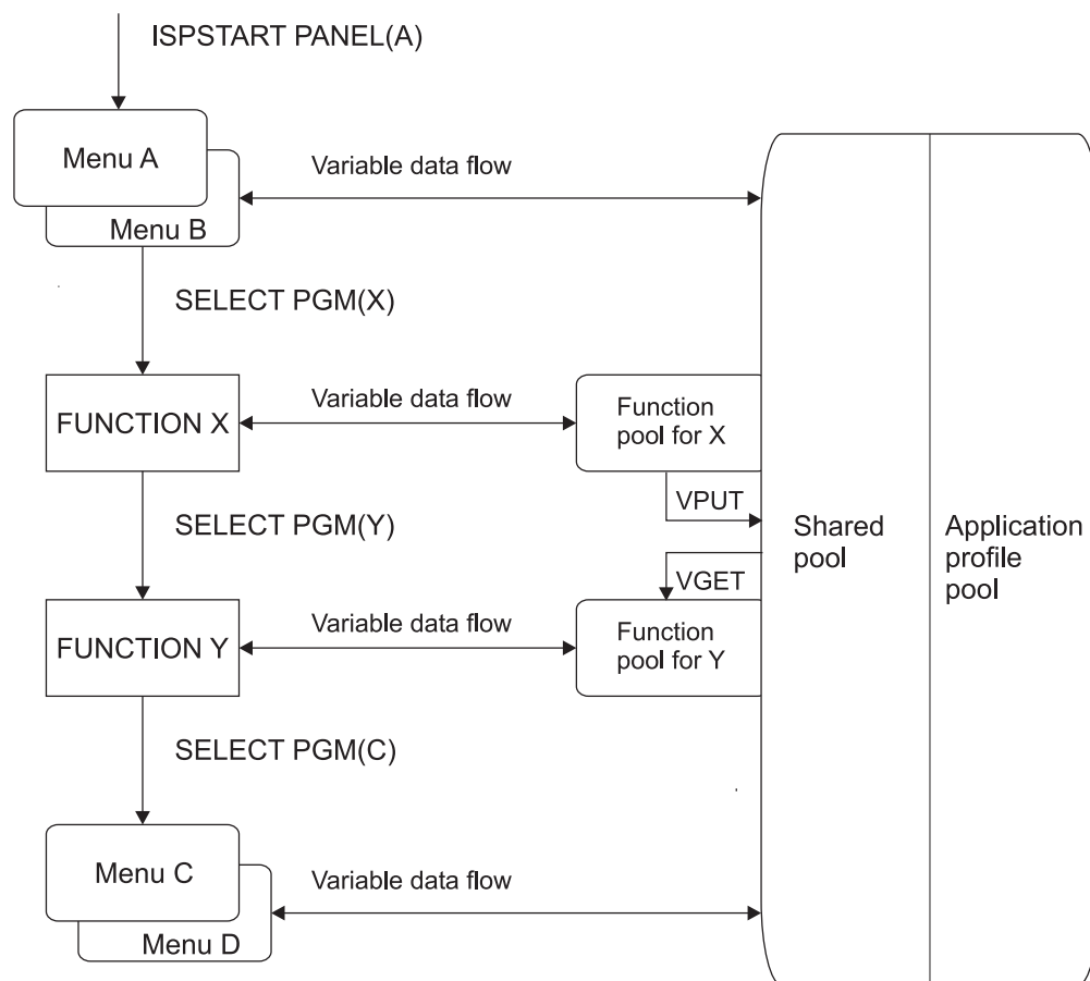
Figure 25. Control and Data Flow in a Dialog
