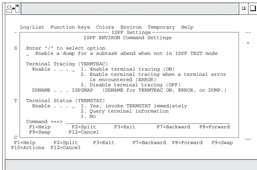
Figure 97. ENVIRON Settings Panel (ISPENVA)
