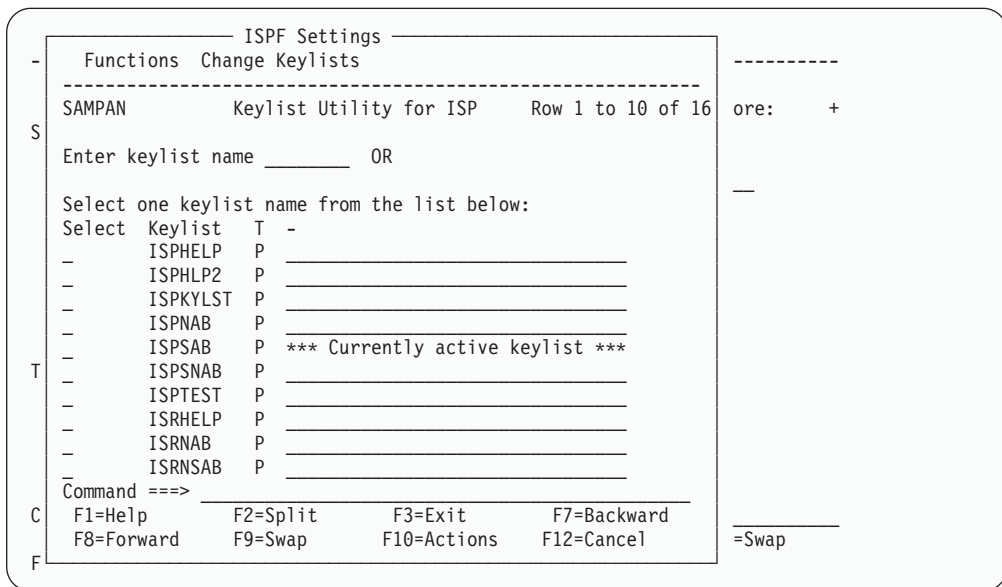
Figure 40. Sample CUA Panel (SAMPAN on ISPKLUP)
