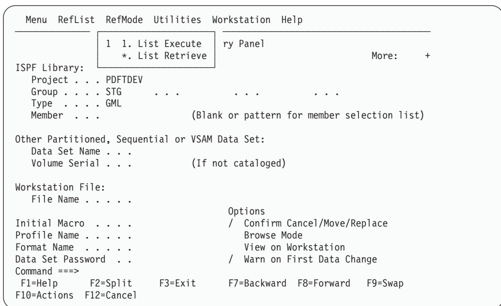
Figure 4. An Unavailable Choice on a Pull-Down
