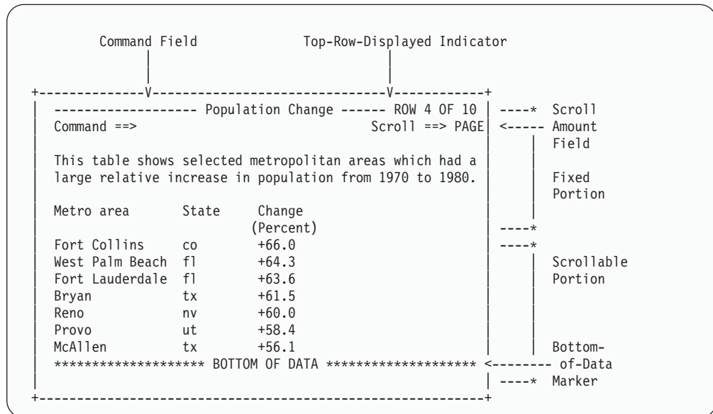
Figure 46. Parts of a TDBISPL display
