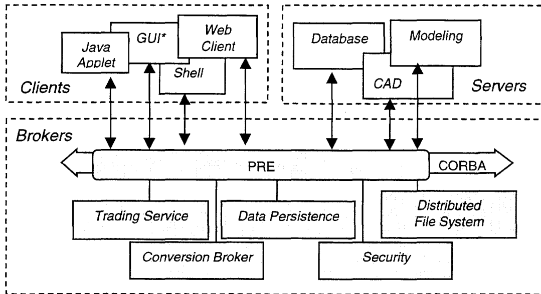
Figure 1. PRE architecture.
