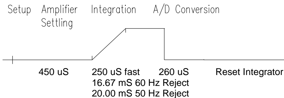
FIGURE 13.1-2. Timing of Single-Ended Measurement
