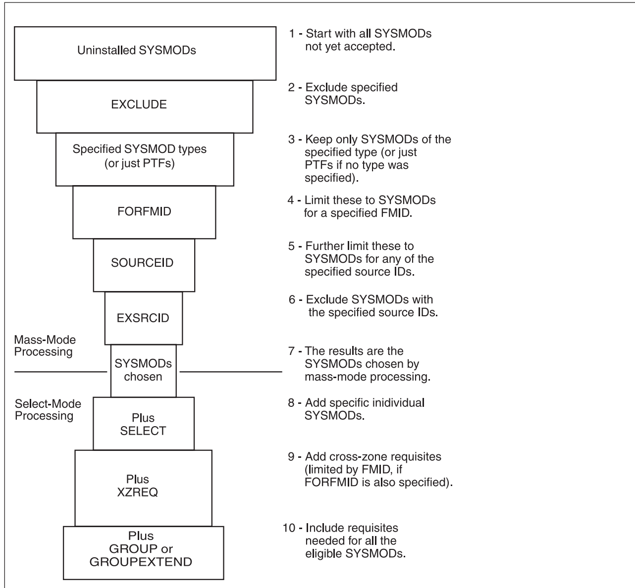
Figure 1. Combining SYSMOD selection operands on the ACCEPT command
