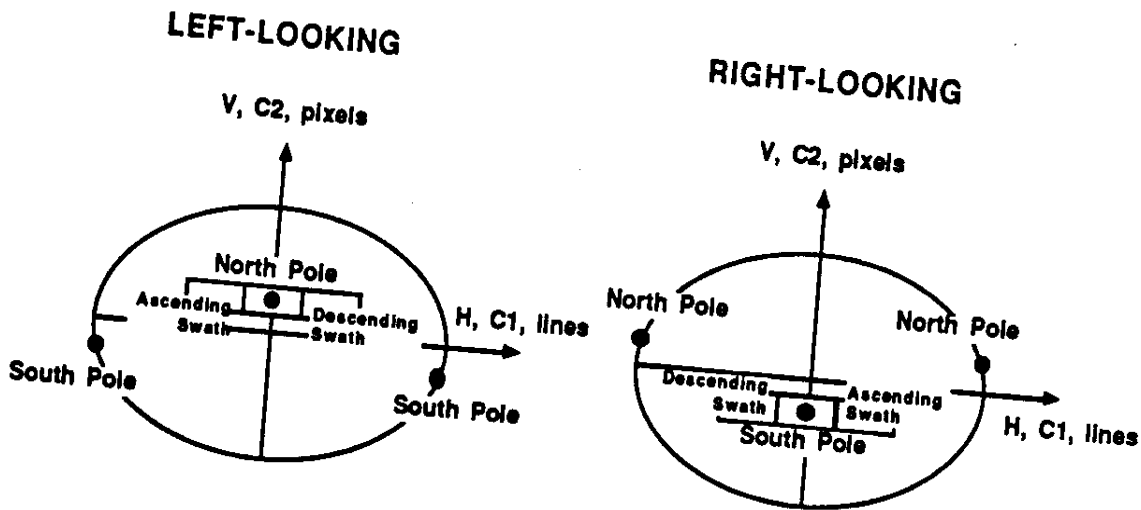
Figure E-2: Relation between the Oblique Sinusoidal and C1/C2 Axes
