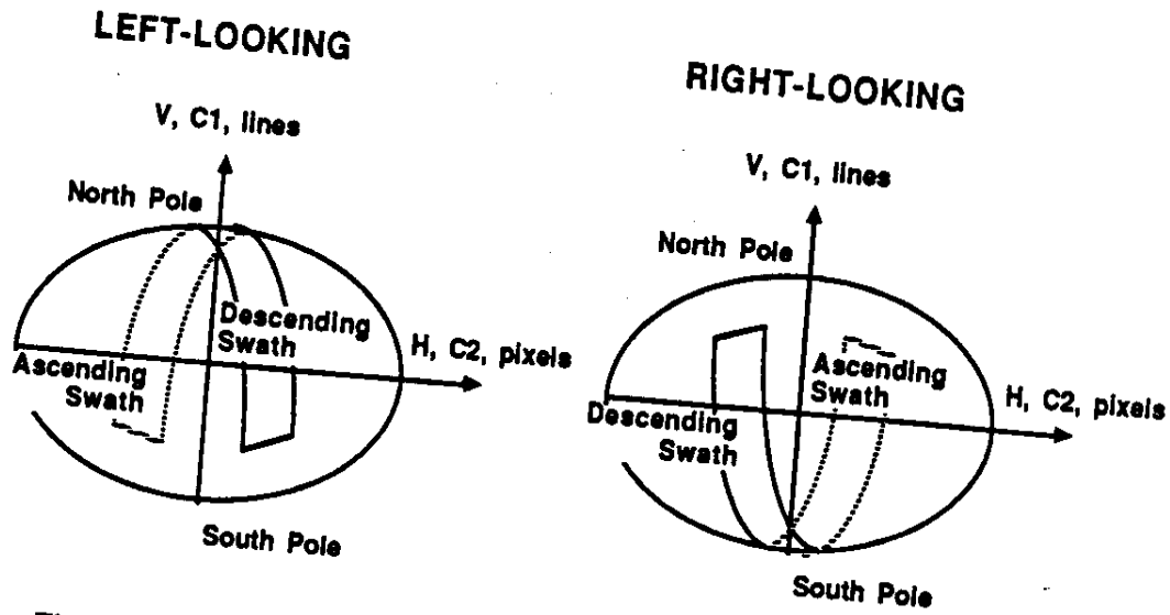
Figure E-1: Relation between the Sinusoidal and C1/C2 Axes
