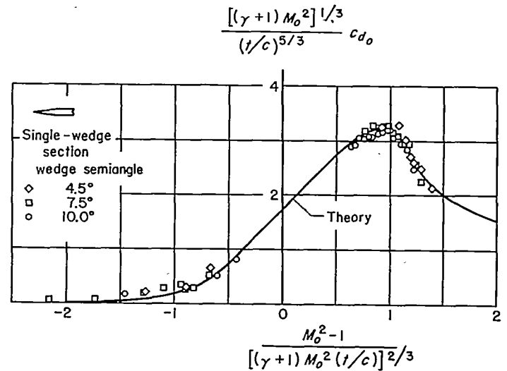
FIGURE 7.—Drag correlation of single-wedge section, k = M_0^2(\gamma + 1)/U_\infty .
