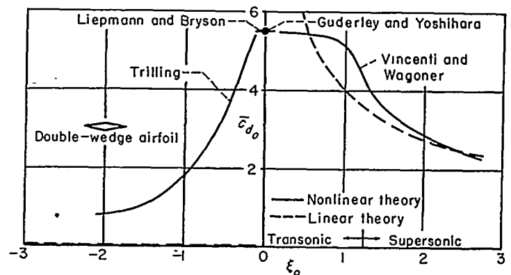
FIGURE 5.—Theoretical drag of double-wedge airfoil.
