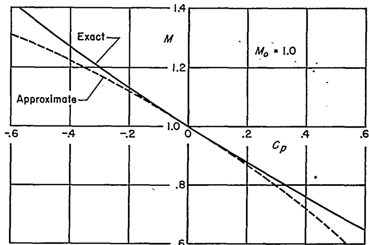
FIGURE 3.—Variation of local Mach number with pressure coefficient for M_o=1 .
