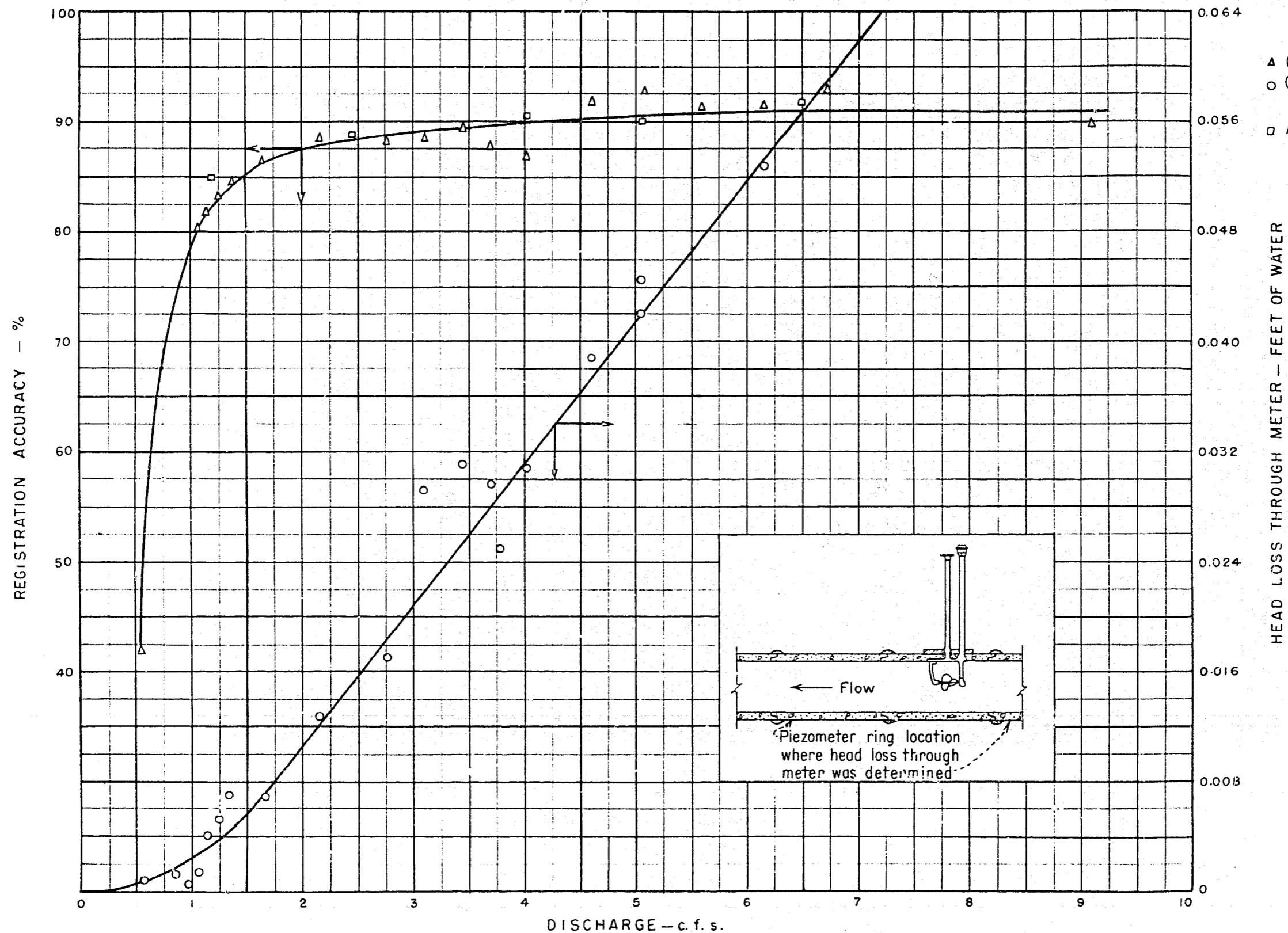
CALIBRATION CURVES 12" SUPERIOR "T" METER
