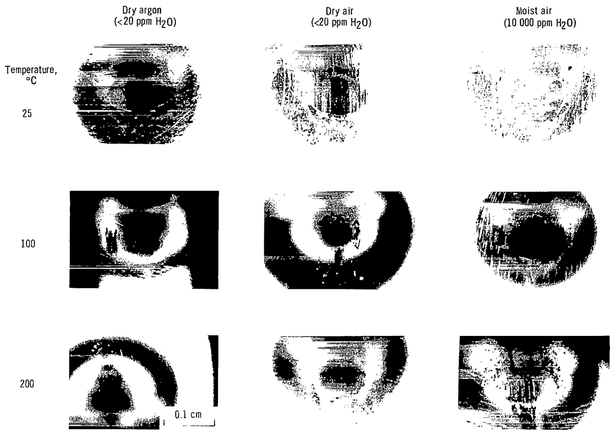
Figure 9. - Photomicrographs of rider transfer films after 60 kilocycles of sliding.
