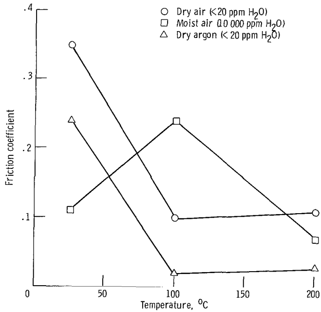
Figure 5. - Effect of temperature and atmosphere on friction coefficient of polyimide films.
