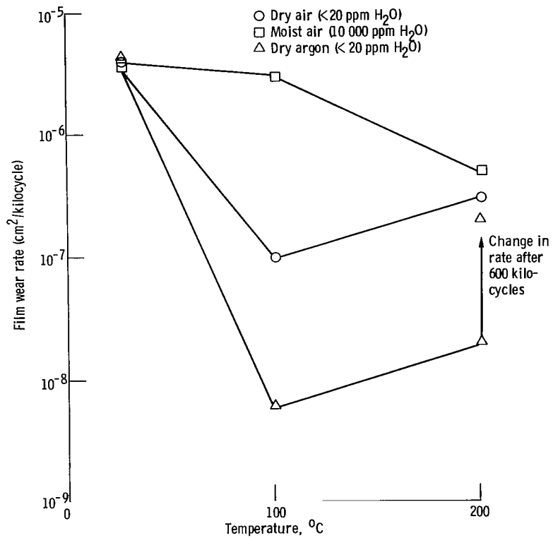
Figure 12. - Effect of temperature and atmosphere on wear rate of polyimide films.
