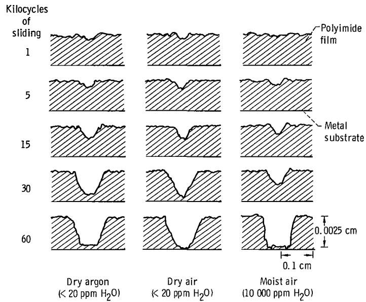
Figure 6. - Effect of atmosphere on wear of polyimide films at 25 o C. Rider and disk material, 440C stainless steel; sliding speed, 2.6 meters per second; load, 1 kilogram.
