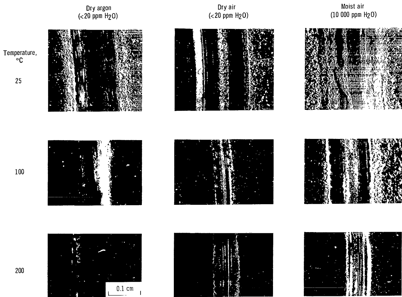
Figure 8. - Photomicrographs of polyimide film wear tracks after 60 kilocycles of sliding.
