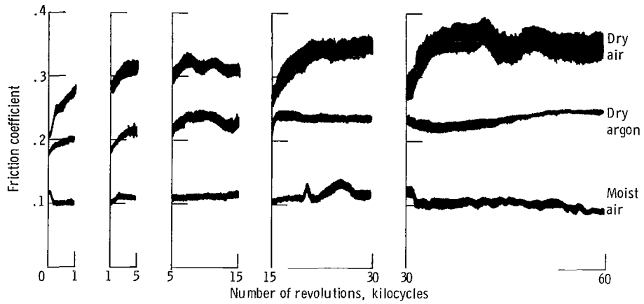
Figure 2. - Effect of atmosphere on friction coefficient of polyimide films at 25 0 C as function of repeated passes (number of revolutions). Rider and disk material, 440C stainless steel; sliding velocity, 2.6 meters per second; load, 1 kilogram; dry argon (<20 ppm H 2 O), dry air (<20 ppm H 2 O), moist air (10 000 ppm H 2 O).
