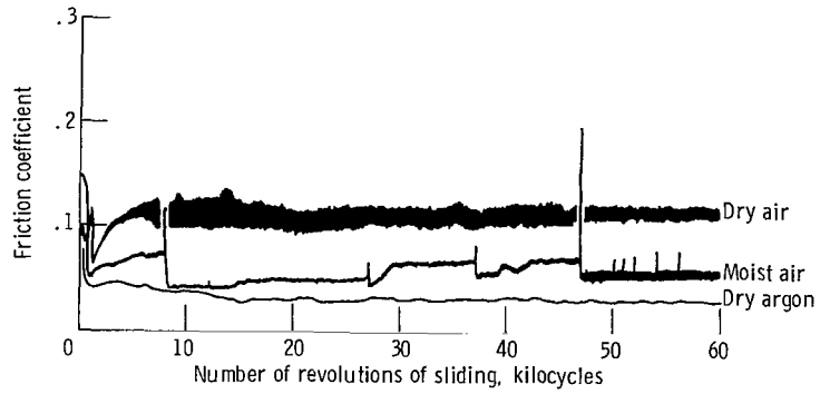
Figure 4. - Effect of atmosphere on friction coefficient of polyimide films at 200° C as function of repeated passes (number of revolutions). Rider and disk material, 440C stainless steel; sliding velocity, 2.6 meters per second; load, 1 kilogram; dry argon (< 20 ppm H 2 O), dry air (< 20 ppm H 2 O), and moist air (10 000 ppm H 2 O).
