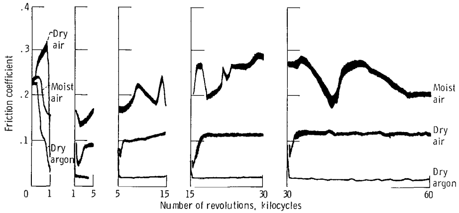
Figure 3. - Effect of atmosphere on friction coefficient of polyimide films at 100 0 C as function of repeated passes (number of revolutions). Rider and disk material, 440C stainless steel; sliding velocity, 2.6 meters per second; load, 1 kilogram; dry argon (<20 ppm H 2 O), dry air (<20 ppm H 2 O), moist air (10 000 ppm H 2 O).
