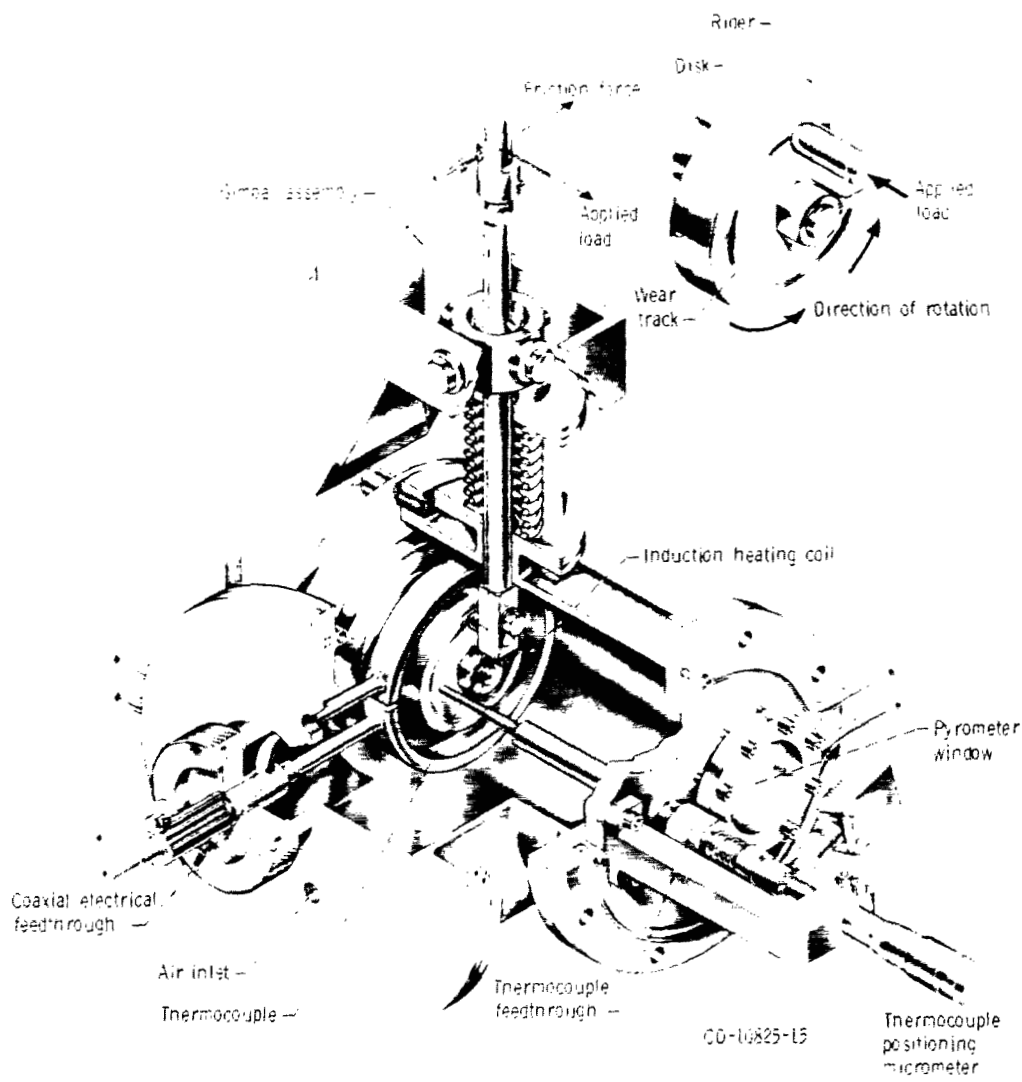
Figure 1. - Friction and wear apparatus.
