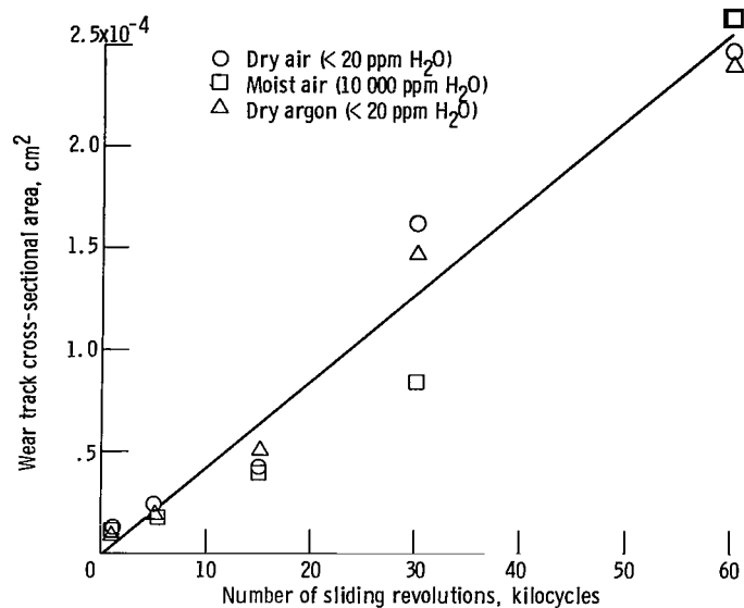
Figure 10. - Polyimide film wear at 25°C as function of kilocycles of sliding. Rider and disk material, 440C stainless steel; sliding velocity, 2.6 meters per second; load, 1 kilogram.
