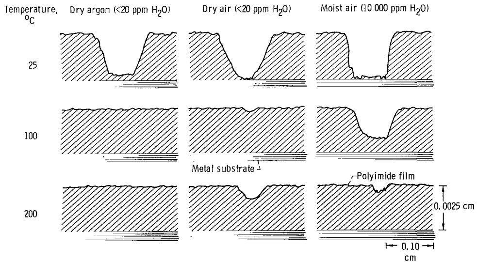
Figure 7. Surface profiles of polyimide film wear tracks after 60 kilocycles of sliding.
