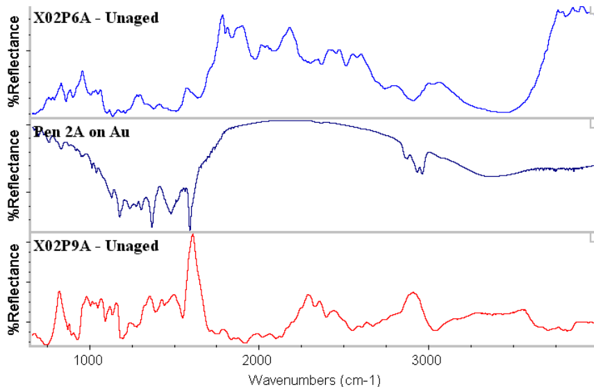
Fig. 1. Infrared spectra of a) a commercial blue ink on a commercial business paper, Xerox 4200DP, b) a commercial black ink on a reflecting metallic substrate, and c) a commercial red ink on the same Xerox 4200DP paper. The background base spectrum of the paper in the spectrum of each ink has been subtracted.
