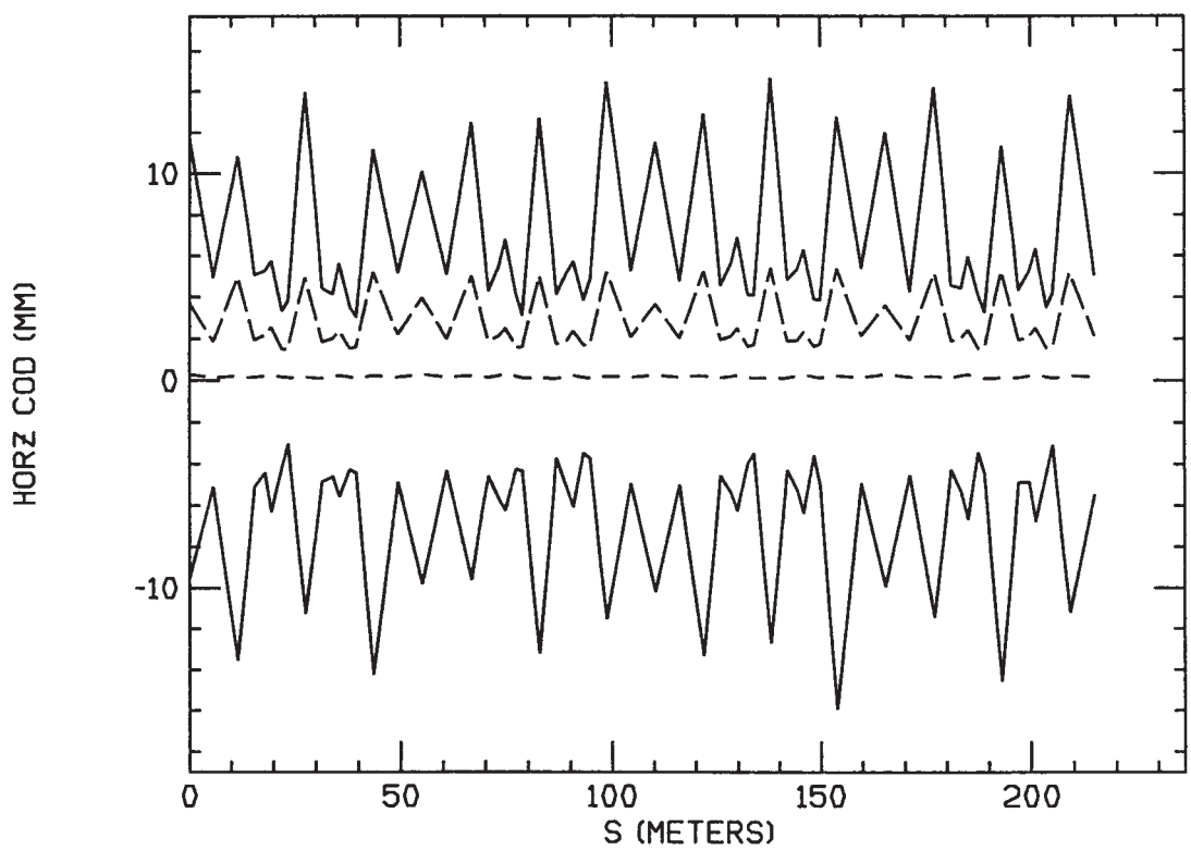
NSNS RING COD (MAX, MIN, RMS) Fig. 2a
