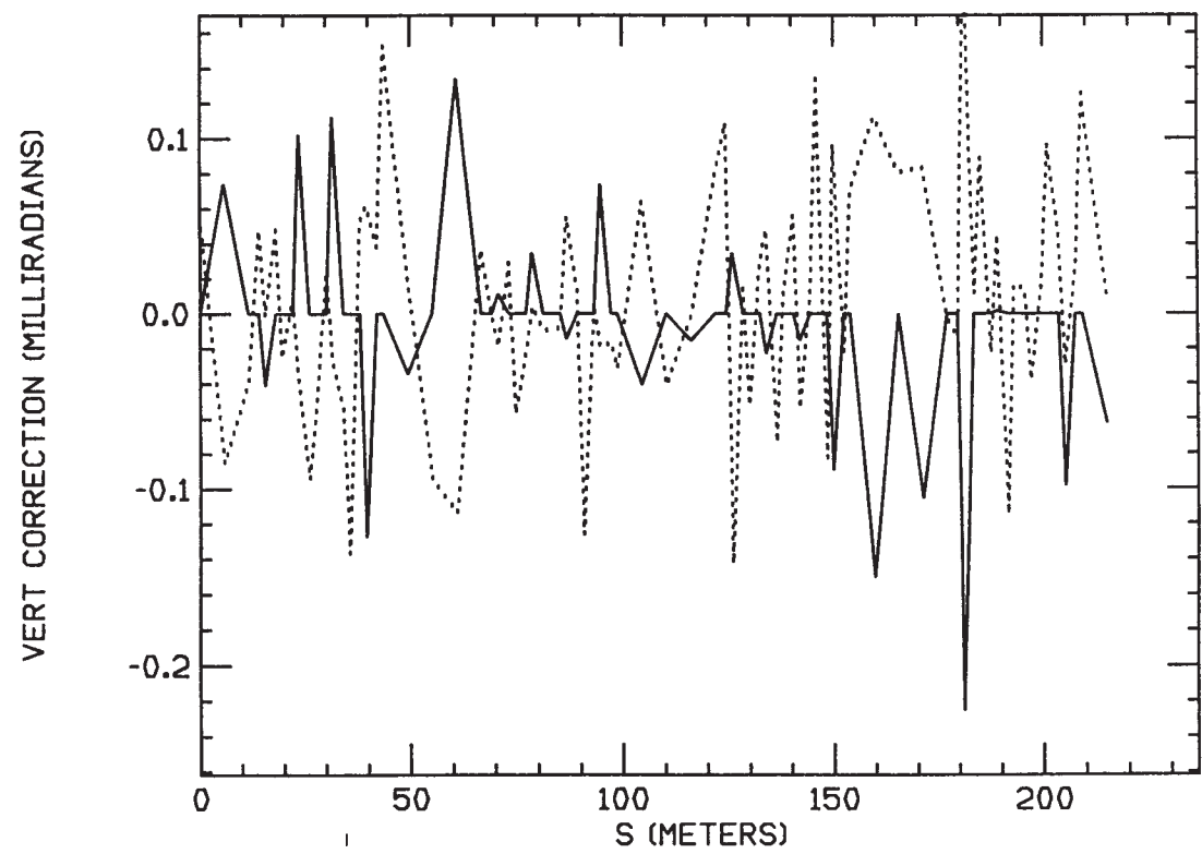
ERRORS (DOTTED) AND 3-BUMP CORRECTION 7b
