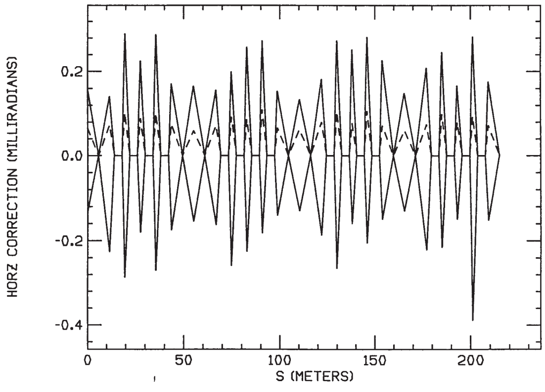
COD CORRECTION (HARMONIC, MAX, MIN, RMS) 2b
