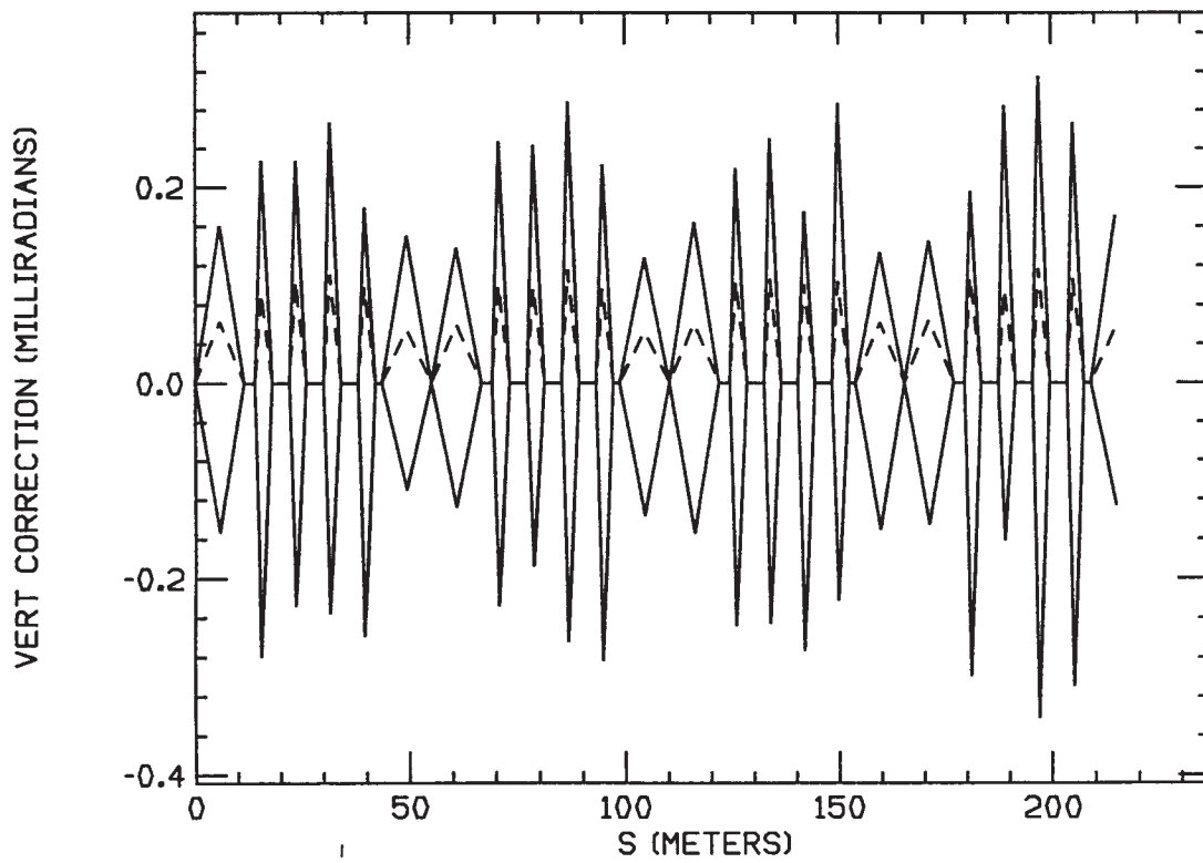
COD CORRECTION (3-BUMP, MAX, MIN, RMS) Fig. 8b
