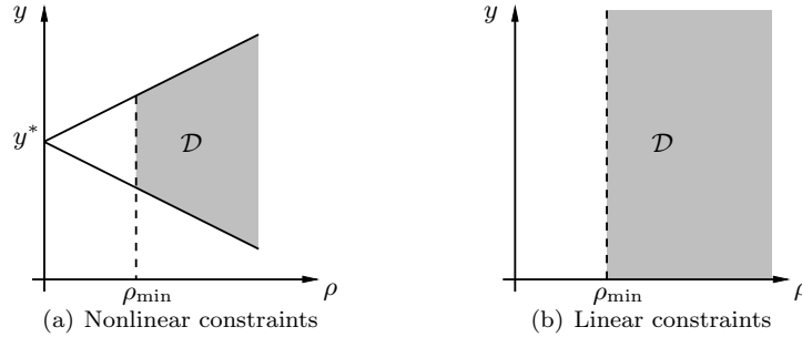
FIG. 2.2. The sets \mathcal{D} illustrate the required penalty parameter for the BCL method when the constraints are either nonlinear or linear.
