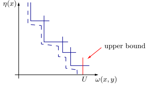
FIG. 2.1. A typical filter. All pairs (\omega, \eta) that are below and to the left of the envelope (dashed line) are acceptable to the filter (cf. (2.2)).
