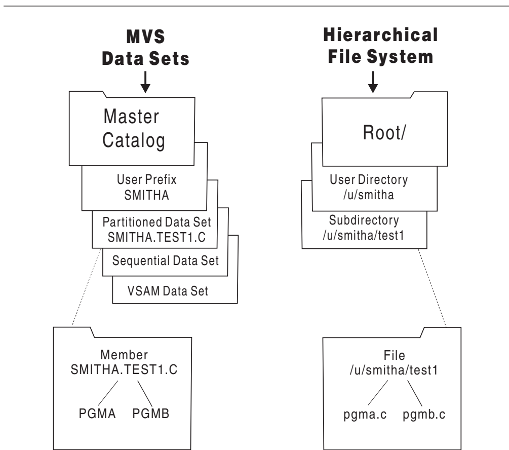
Figure 22. Comparison of MVS data sets and a hierarchical file system
