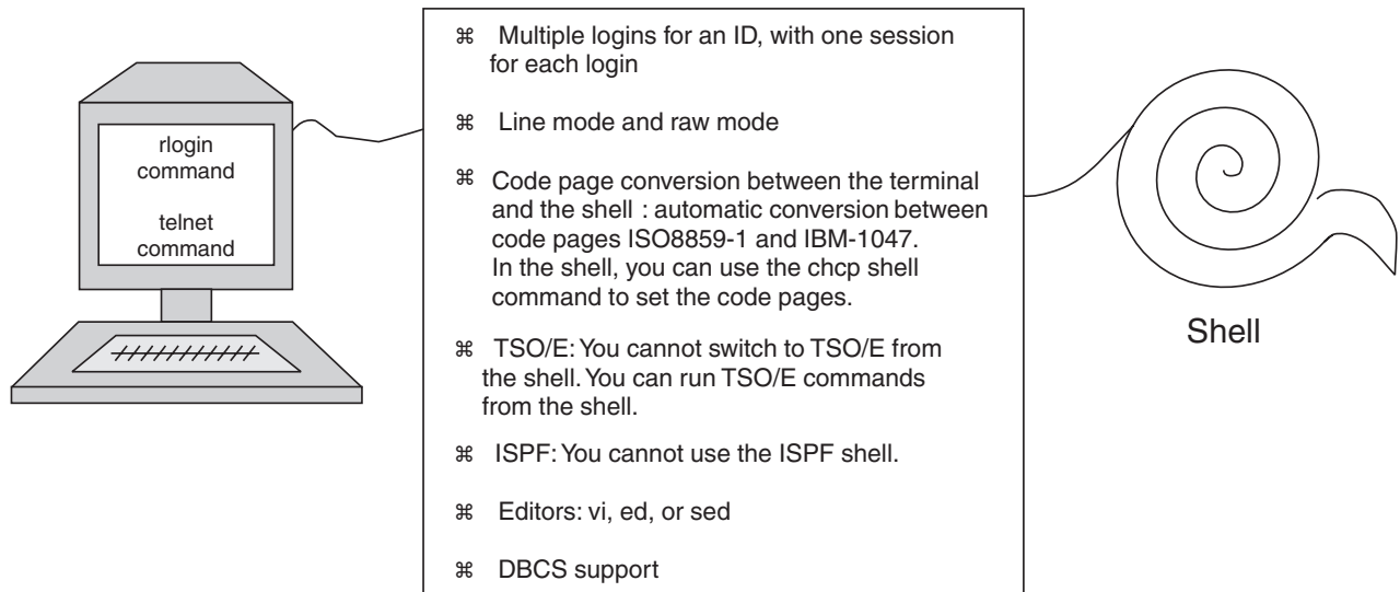
Figure 3. The asynchronous terminal interface to the shell
