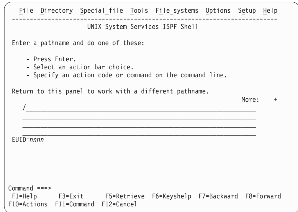
Figure 19. ISPF shell: The main panel
