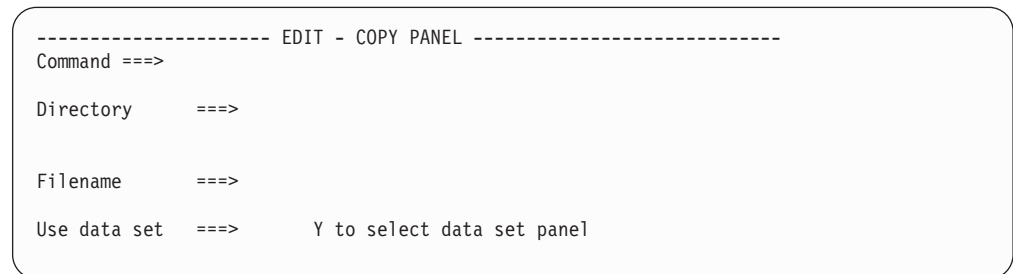
Figure 32. ISPF Edit Copy panel for an HFS file
