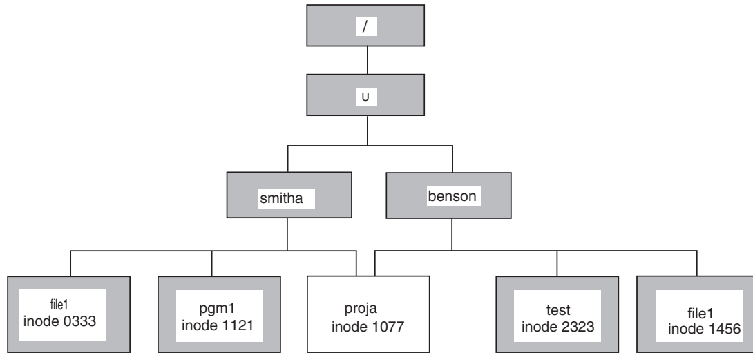
Figure 26. Hard link: a new name for an existing file. The hard link has an identical inode number.
