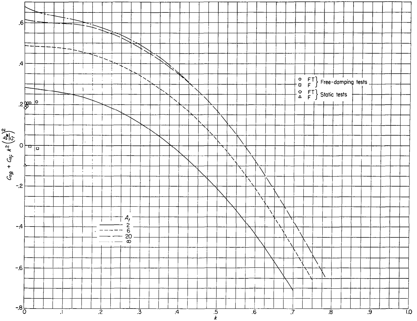
FIGURE 11.—The effect of aspect ratio on the directional stability as calculated by the method of Biot and Boehlein for a range of reduced frequencies.
