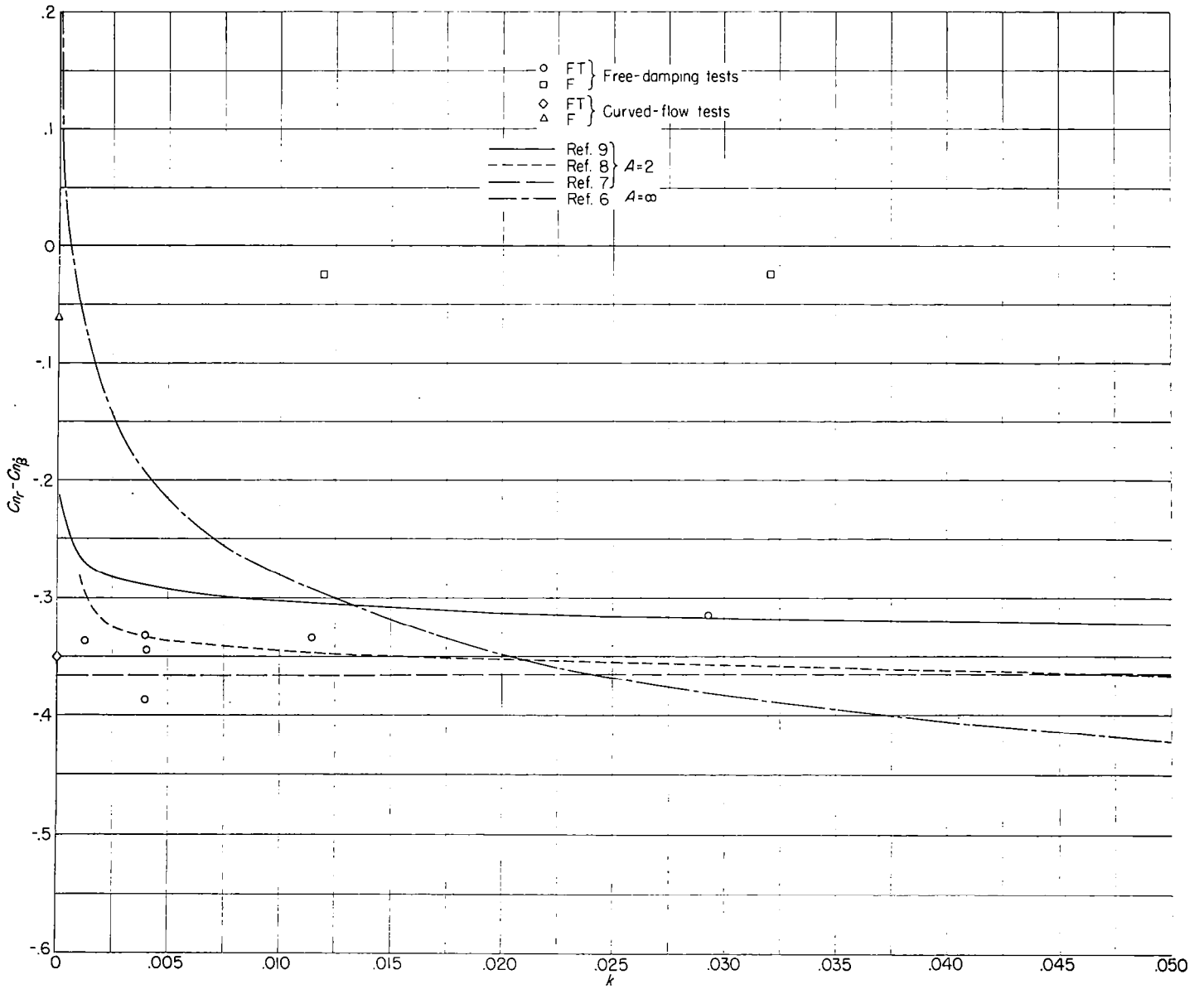
FIGURE 7.—The effect of frequency on the damping in yaw for a low range of the reduced frequency. Comparison of several methods for calculating frequency effect on the damping in yaw.
