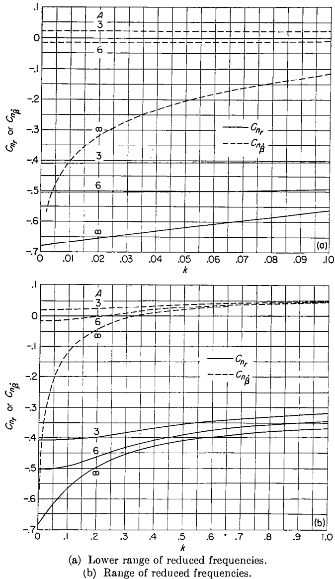
FIGURE 9.—The effect of reduced frequency on the stability derivatives C_{n_r} and C_{n_r\beta} .
