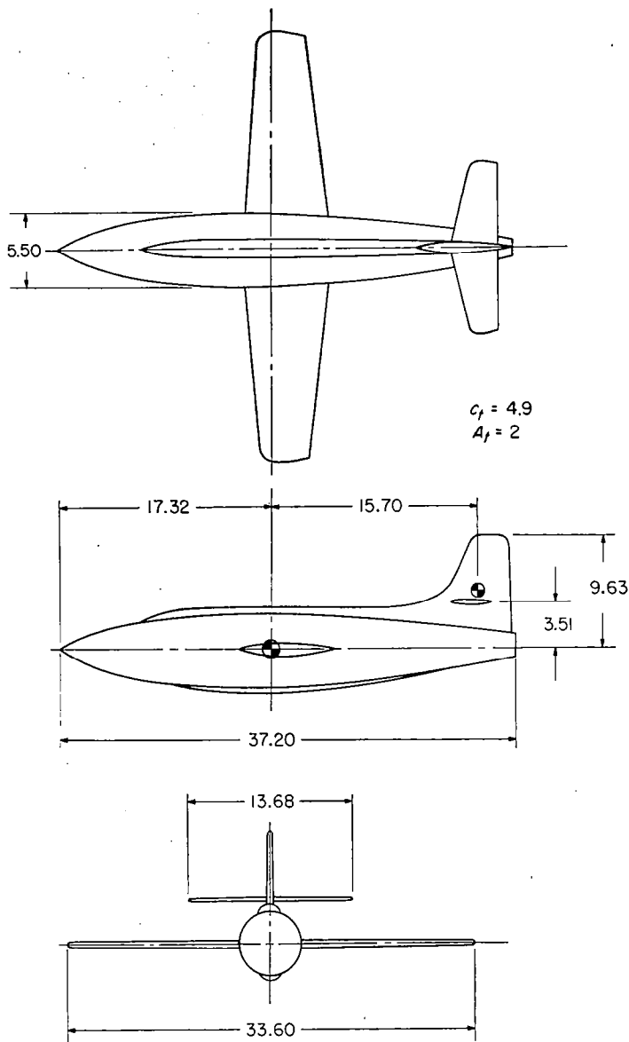
FIGURE 2.—Drawing of model tested. All dimensions are in inches.
