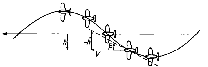
Sideslipping, \beta = \beta_0 e^{i\omega t}
