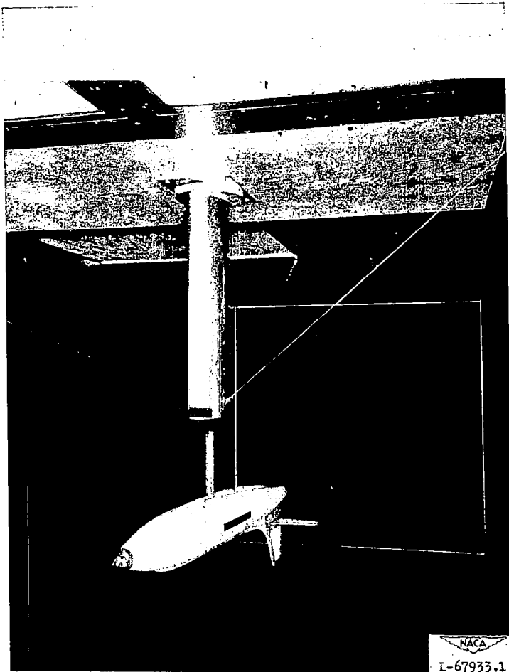
FIGURE 4.—Test model mounted on free-oscillation strut in Langley stability tunnel.
