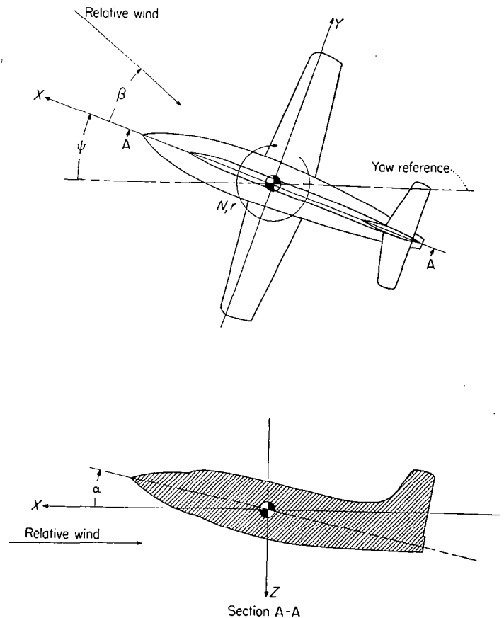
FIGURE 1.—System of stability axes. Arrows indicate positive forces, moments, and angular displacements. Yaw reference generally chosen to coincide with initial relative wind.
