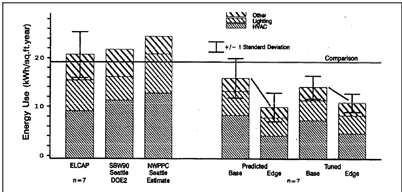
Figure 2. End-use Energy Consumption for Seven Energy Edge Small Offices and Comparison Buildings
