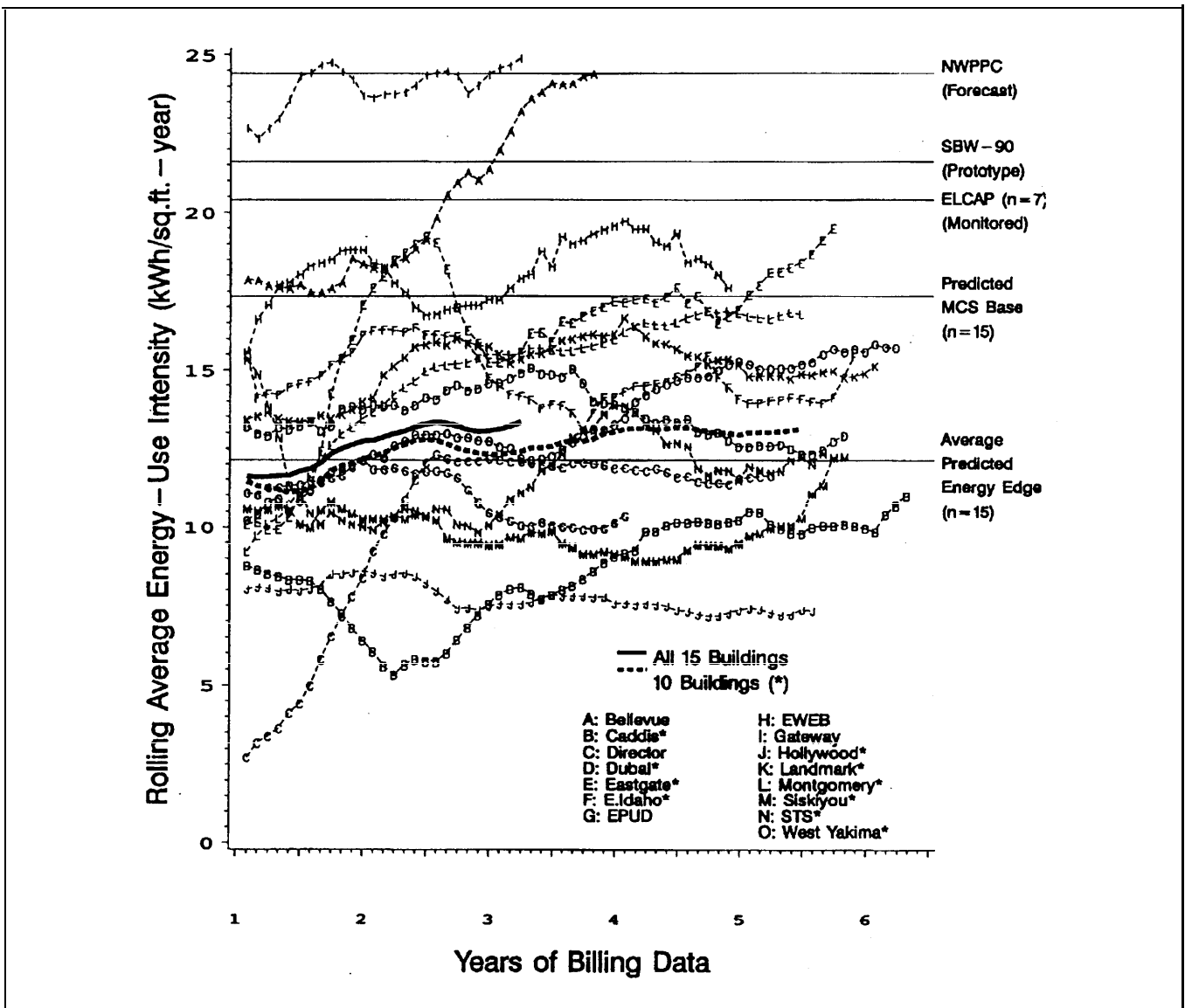
Figure 1. Energy Consumption Over Time for 15 Energy Edge Office Buildings and New Regional Comparison Buildings
