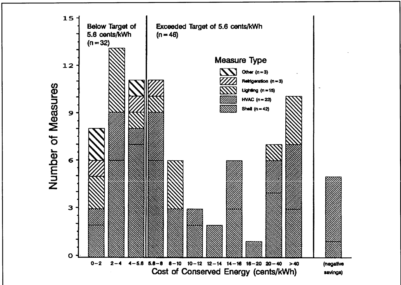
Figure 3. Distribution of CCEs for 78 Measures with Tuned Energy Savings from 18 Buildings. Forty-one percent of the measures met the CCE target
