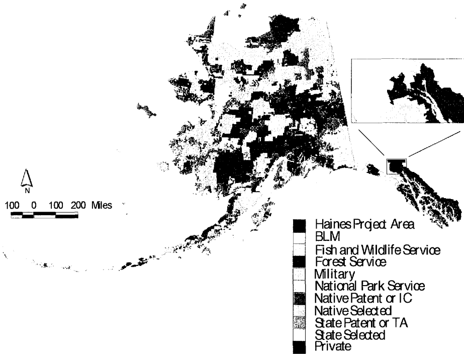
Figure 2. Land ownership within the Haines project area.
